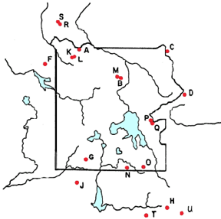
Fig. 5. Locations of whitebark pine cone transects within the study area.
