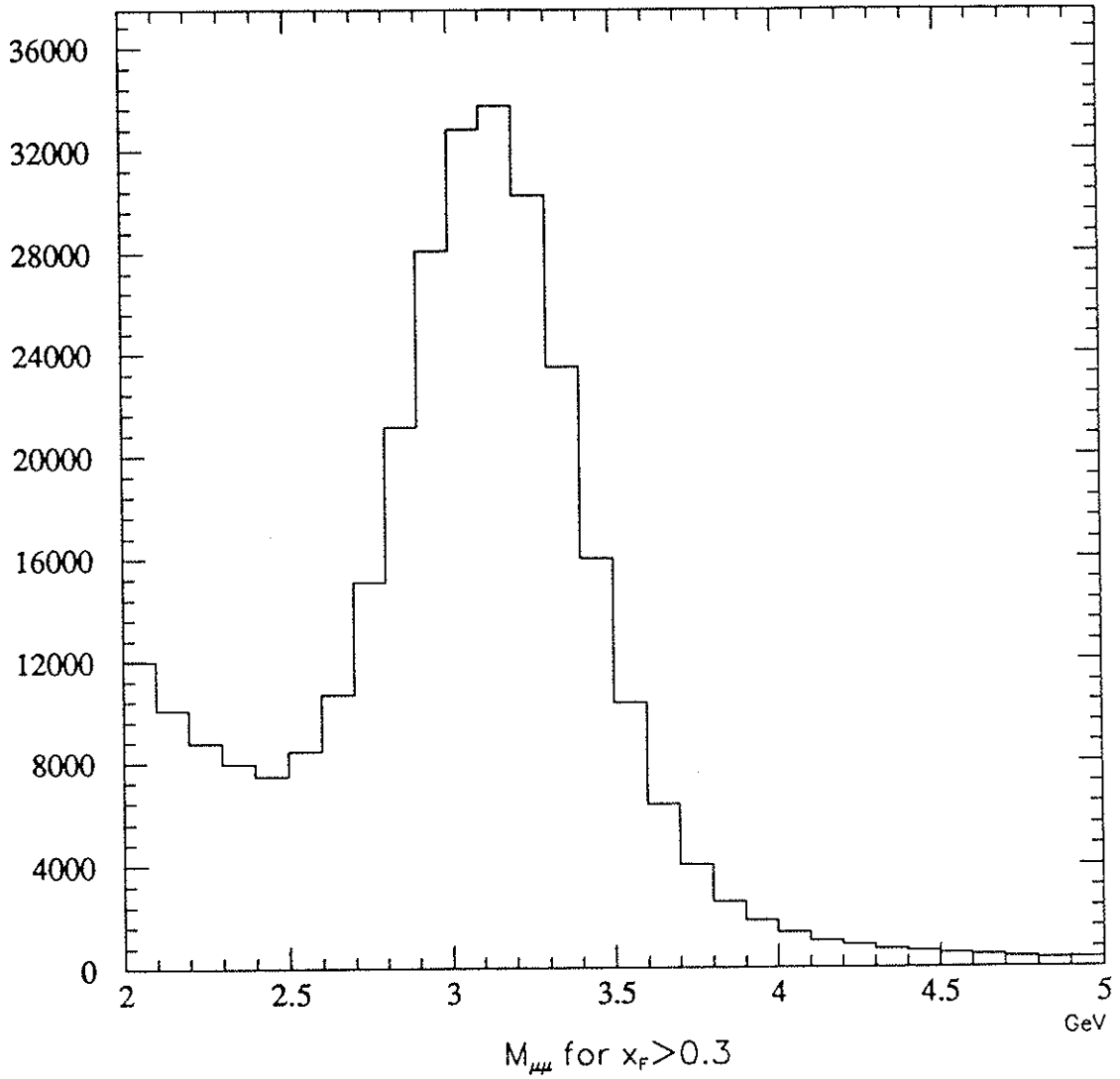
Figure 3.7: Invariant \mu^+\mu^- mass spectrum of events with x_F > 0.3 in p+Cu collisions.
