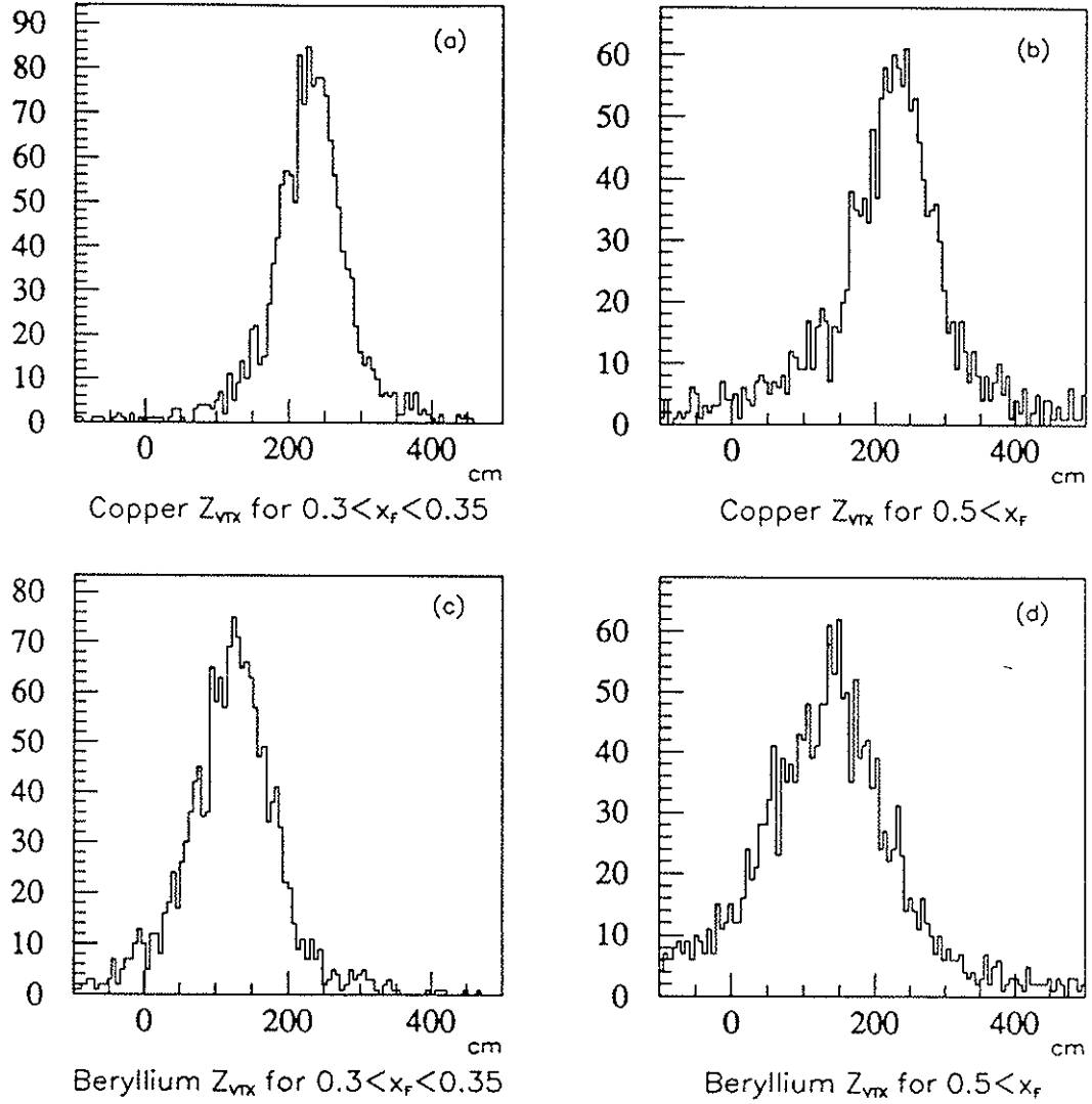
Figure 3.2: Z_{vtx} determined from the track traceback in the Y-Z view. (a) and (b) show the distributions in the copper dump data for two regions in x_F , while (c) and (d) show the same regions in x_F for the beryllium dump data. Note that the beam dump extends from Z = 203 cm to Z = 599 cm, and the beryllium extends from Z = 60 cm to Z = 151 cm.
