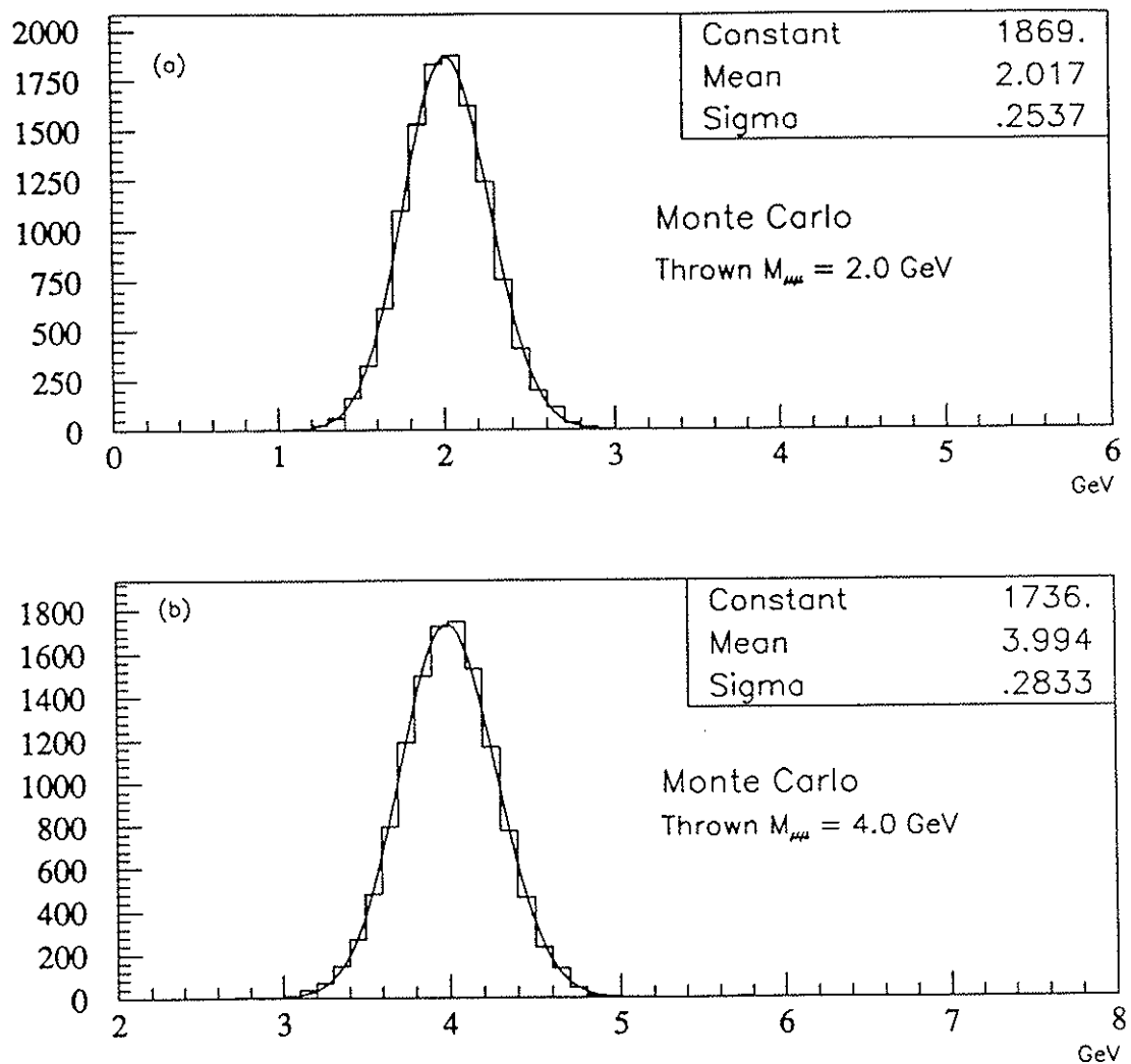
Figure 3.3: Reconstructed dimuon mass of Monte Carlo events. (a) shows the reconstructed mass spectrum for Monte Carlo dimuons generated with m_{\mu\mu} = 2.0 GeV, while (b) shows the one for m_{\mu\mu} = 4.0 GeV. The inset values are from a gaussian fit.
