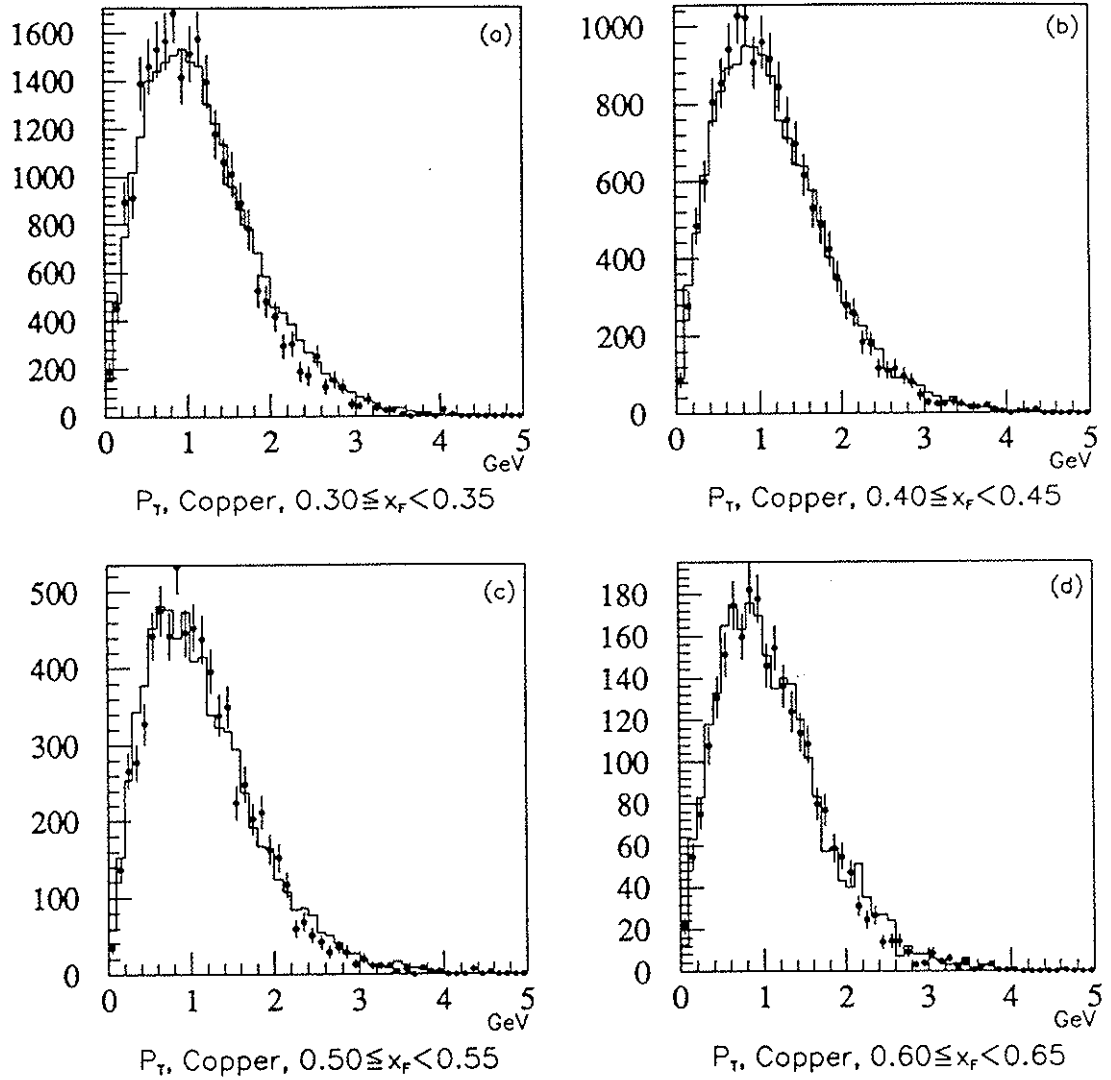
Figure 3.17: Reconstructed p_{\perp} distributions for copper dump data and Monte Carlo events. (a) – (d) show x_F bins with mean x_F at 0.325, 0.425, 0.525, and 0.625. The solid line is data from the copper beam dump, and the points are reconstructed Monte Carlo events. Monte Carlo events were generated according to the distribution of equation (3.18), with p_0 = 2.79 GeV at low x_F , and slowly decreasing to p_0 = 2.60 GeV at x_F = 0.925 .
