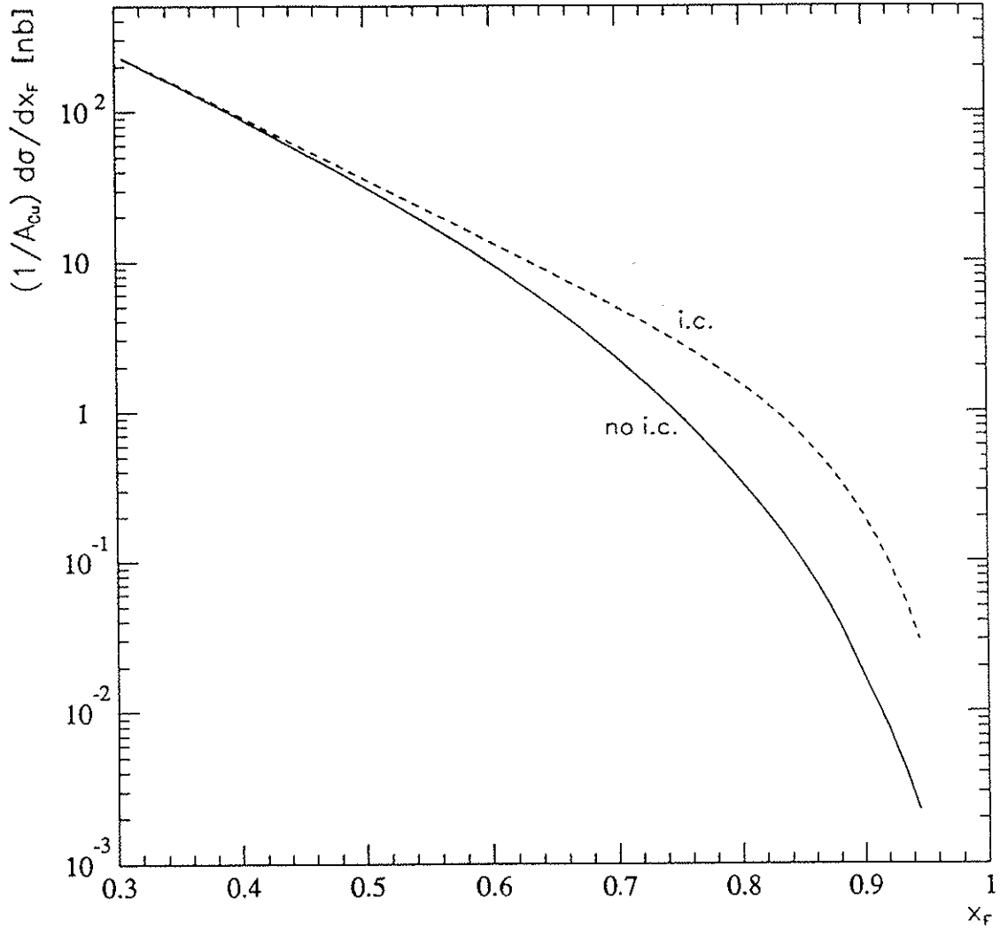
Figure 1.7: Intrinsic charm model calculation of d\sigma/dx_F(p + Cu \rightarrow J/\psi + X) . The solid curve shows the prediction of the semilocal parton duality model, including the effect of target parton shadowing. The dashed curve shows the cross section including the additional contribution predicted by the intrinsic charm model.
