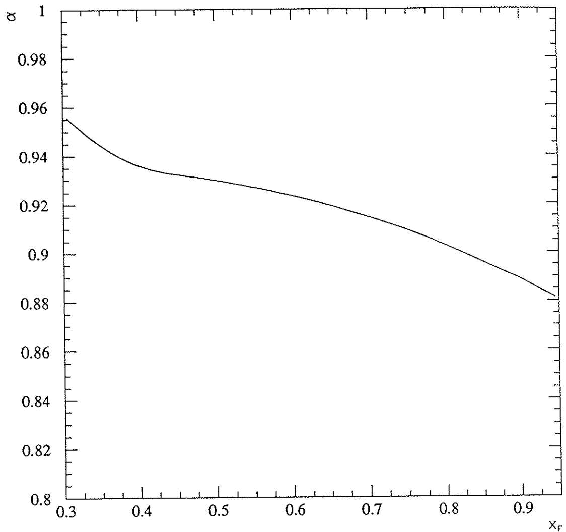
Figure 1.5: A -dependence of J/\psi production predicted by target parton shadowing. Assuming d\sigma/dx_F \propto A^\alpha , the prediction was determined by a semilocal duality calculation for p+\text{Cu} and p+\text{Be} collisions. MRS set S_0 parton distribution functions were used, with target distribution functions modified according to equations (1.11) and (1.12).
