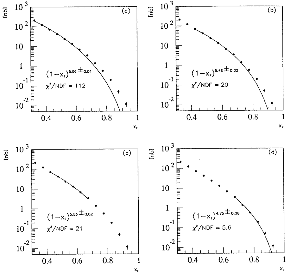
Figure 4.3: Fits to (1 - x_F)^n for p+Cu data. (a) shows the fit to the entire range in x_F , (b) excludes the first two points, (c) is fit to the range 0.40 < x_F < 0.70 , and (d) is fit for x_F > 0.65 .
