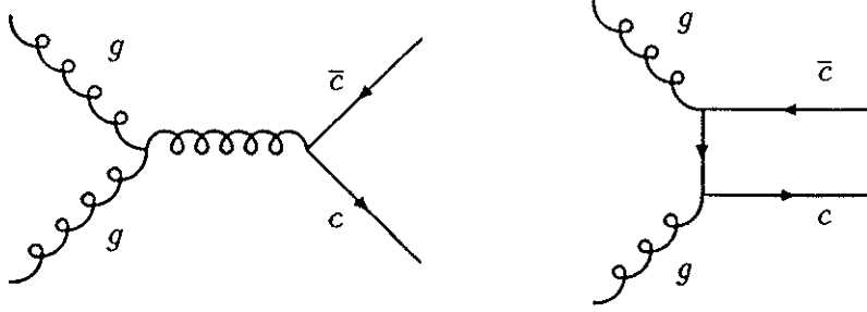
Figure 1.2: gg fusion diagrams
