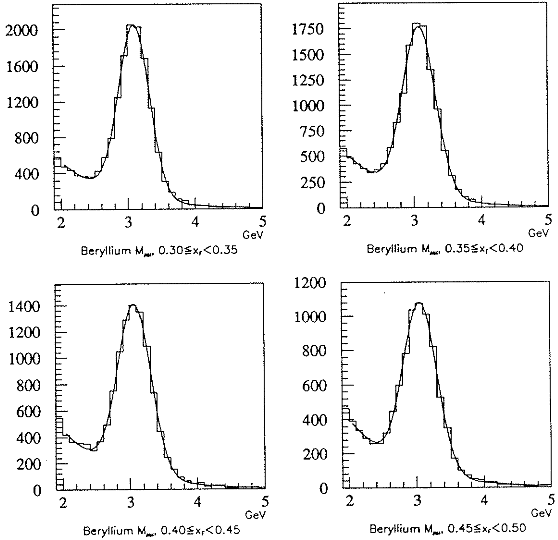
Figure 3.13: Fits to dimuon mass spectra with 0.3 < x_F < 0.5 , for the beryllium dump data. The ordinate shows the number of events per 100 MeV bin.
