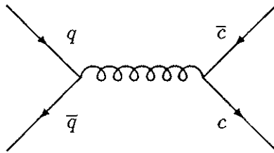
Figure 1.1: q\bar{q} annihilation diagram
