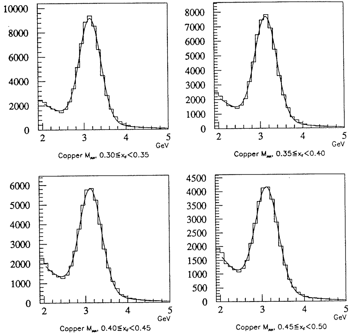
Figure 3.9: Fits to dimuon mass spectra with 0.3 < x_F < 0.5 , for the copper dump data. The ordinate shows the number of events per 100 MeV bin.
