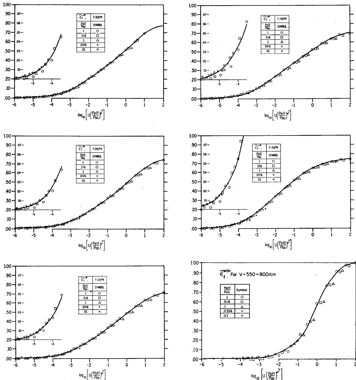
FIG. 26. The mean slab absorptivity of H_2O , from which the contribution of the range of wave number 550-800 \text{ cm}^{-1} is omitted. In the lower right corner is shown the slab absorptivity of H_2O for the omitted range of wave number.
