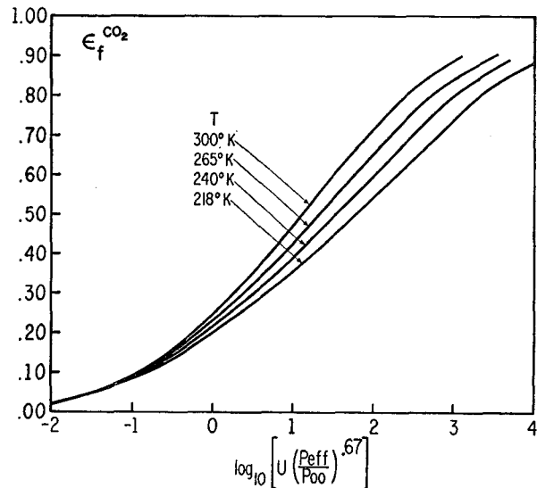
FIG. 29. Slab absorptivities of CO 2 at various temperatures.
