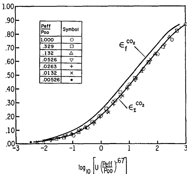
FIG. 28. Slab absorptivity \epsilon_f and column absorptivity \epsilon_1 of CO 2 at 300K. Bandwidth is assumed to be 250 cm -1 .
