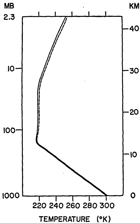
FIG. A-7. Thermal equilibrium obtained by using the scaling approximation (solid line) and by adopting the effective pressure defined by equation (A-1). S_e = 2 \text{ ly min}^{-1} , \cos \bar{\zeta} = 0.5 , r = 0.5 . No clouds. Gaseous absorbers: distributions of 35N, April.
