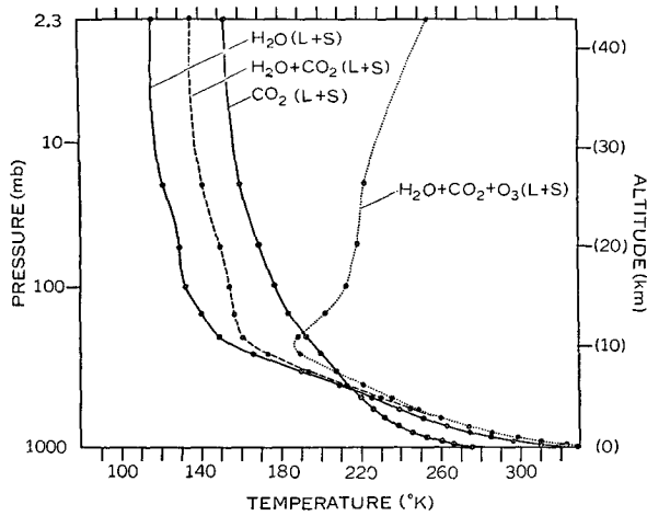
FIG. 6a. Pure radiative equilibrium for various atmospheric absorbers. The distribution of gaseous absorbers at 35N in April are used. S_c = 2 \text{ ly min}^{-1} , \cos \bar{\zeta} = 0.5 , r = 0.5 . No clouds. (L+S) means that the effects of both long wave radiation and solar radiation are included.
