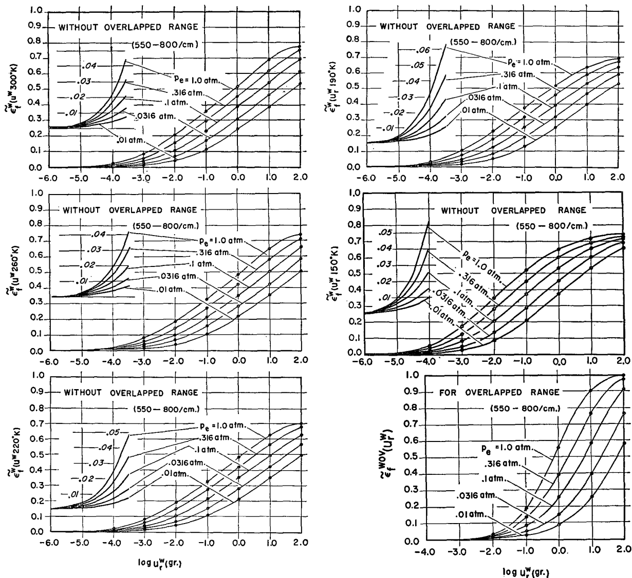
FIG. A-1. The mean slab absorptivities of water vapor for various pressures and temperatures. The mean slab absorptivity of water vapor for the range overlapped with the 15 \mu band of \text{CO}_2 is shown in the lower right corner. The mean slab absorptivity and the logarithm (base 10) of the effective optical thickness (gram \text{cm}^{-2} ) are the ordinate and abscissa, respectively.
