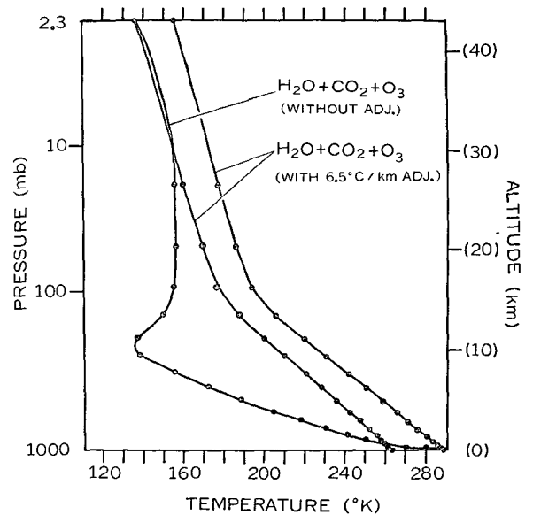
FIG. 6d. Pure radiative and thermal equilibrium without sunshine. The temperature of the earth's surface was fixed at 289K for pure radiative equilibrium, and at 289K or 263K for thermal equilibrium.
