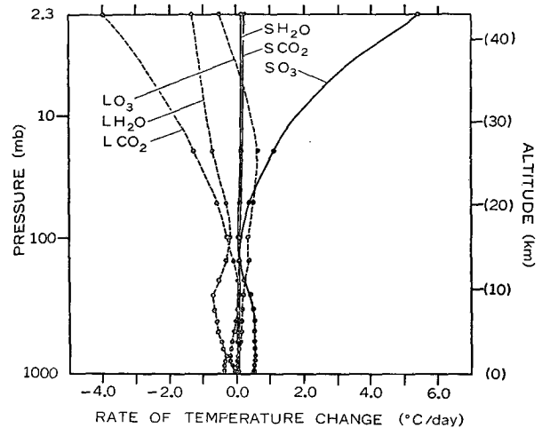
FIG. 6b. Vertical distributions of the rate of temperature change of the (\text{H}_2\text{O} + \text{CO}_2 + \text{O}_3) atmosphere in pure radiative equilibrium due to various absorbers. \text{LH}_2\text{O} , \text{LCO}_2 , and \text{LO}_3 show the rate of temperature change due to long wave radiation of water vapor, \text{CO}_2 (the effect of \text{H}_2\text{O} overlapping was included), and \text{O}_3 . \text{SH}_2\text{O} , \text{SCO}_2 , and \text{SO}_3 show the rate of temperature change due to the absorption of solar radiation by water vapor, \text{CO}_2 , and \text{O}_3 .
