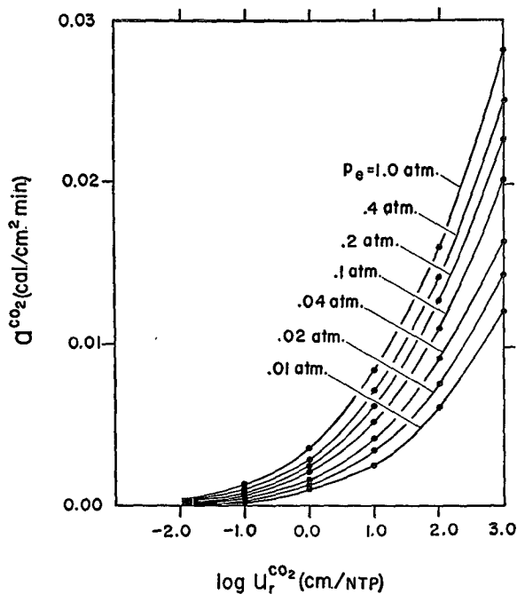
FIG. A-5. Absorption of solar radiation by CO 2 under various pressures. The rate of absorption (cal min -1 cm -2 ) and the logarithm (base 10) of the effective optical thickness (cm at N.T.P.) are the ordinate and abscissa, respectively.
