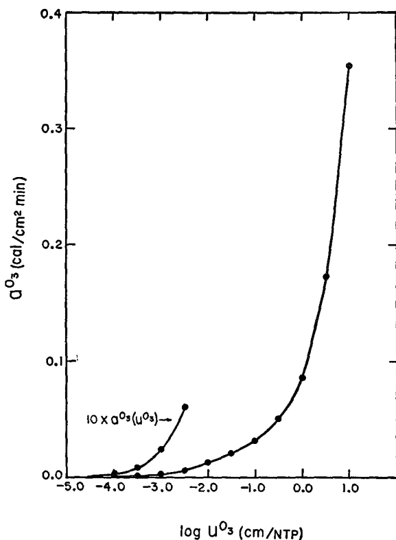
FIG. A-6. Absorption of solar radiation by O 3 under various pressures. The rate of absorption (cal min -1 cm -2 ) and the logarithm (base 10) of the effective optical thickness (cm at N.T.P.) are the ordinate and abscissa, respectively.
