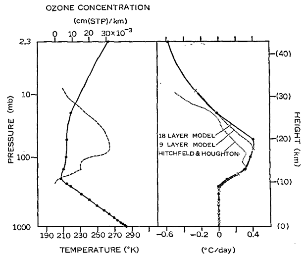
FIG. A-8. On the right, the rate of temperature change obtained by Hitchfeld and Houghton (1961) (dotted line) is shown together with that obtained by our scheme (solid and dashed lines). On the left are shown the vertical distributions of O_3 (dashed line) and temperature (solid line).
