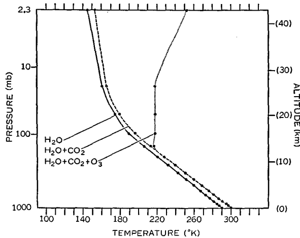
FIG. 6c. Thermal equilibrium of various atmospheres which have a critical lapse rate of 6.5 \text{ deg km}^{-1} . Vertical distributions of gaseous absorbers at 35N, April, were used. S_c = 2 \text{ ly min}^{-1} , \cos \bar{\zeta} = 0.5 , r = 0.5 , no clouds.
