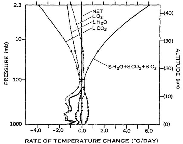
FIG. 8b. Vertical distributions of radiative balance components for the thermal equilibrium of the atmosphere with the average cloudiness shown in Fig. 8a. "Net" means the net rate of temperature change due to all of these components. Refer to Fig. 6b for further explanation.
