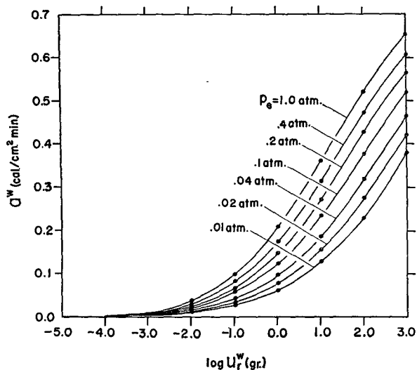
FIG. A-4. Absorption of solar radiation by water vapor under various pressures. The rate of absorption (cal min -1 cm -2 ) and the logarithm (base 10) of the effective optical thickness (gram cm -2 ) are the ordinate and abscissa, respectively.
