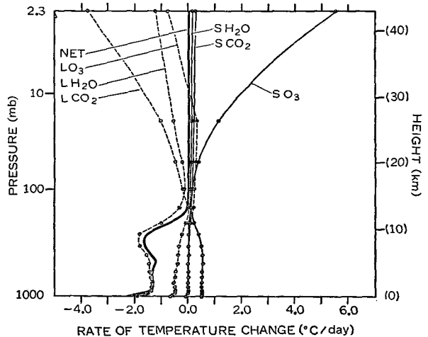
FIG. 8c. Vertical distributions of the radiative heat balance components for the thermal equilibrium of a clear atmosphere. Refer to Fig. 6b for further explanation.
