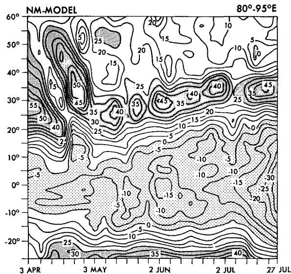
FIG. 5.3. Latitude-time section of zonally averaged ( 80^{\circ}\text{--}95^{\circ}\text{E} ) 5-day mean zonal winds ( \text{m s}^{-1} ) at the 190 mb level of the NM-model.
