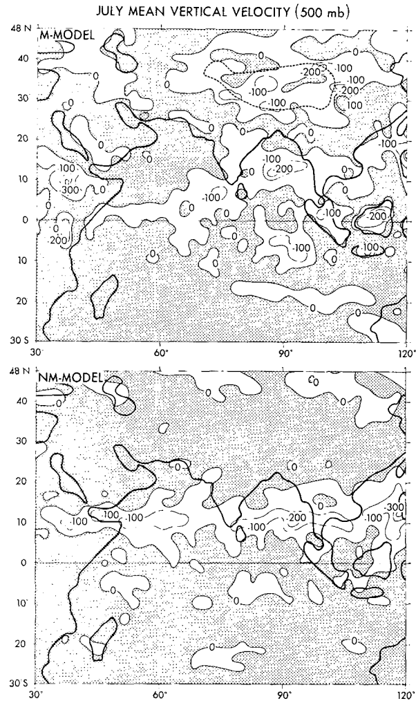
FIG. 4.6. Horizontal distribution of July mean vertical velocity (mb day -1 ) at the 500 mb level of the M-model (top) and the NM-model (bottom).
