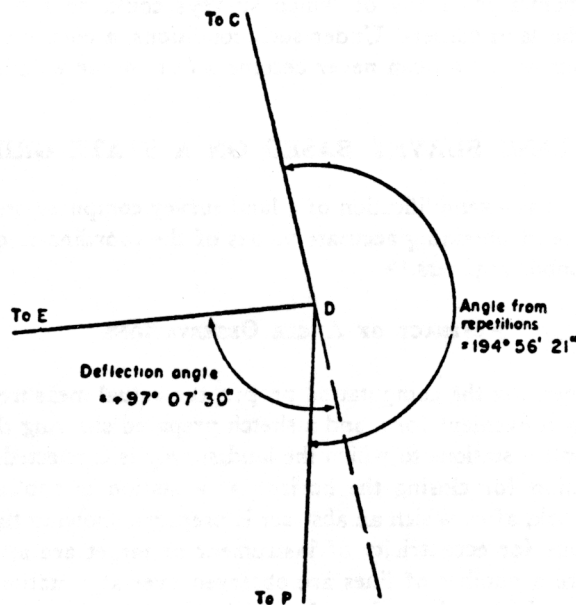
FIGURE 17.—Two methods of observing horizontal angles
