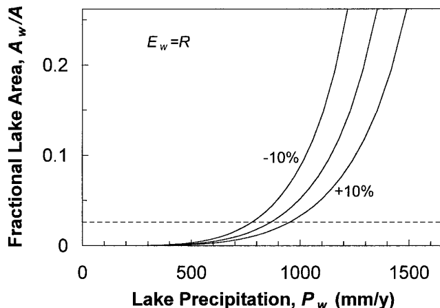
FIG. 2. Fractional lake area A_w/A as function of lake precipitation P_w , for various values of surface net radiation, R . Calculations were performed using E_w = R in place of (7). The central curve uses R = 1590 mm/yr, while other curves use values of R 10% lower or higher than this value. Maximum graph values and horizontal dashed line are as in Figure 1.
