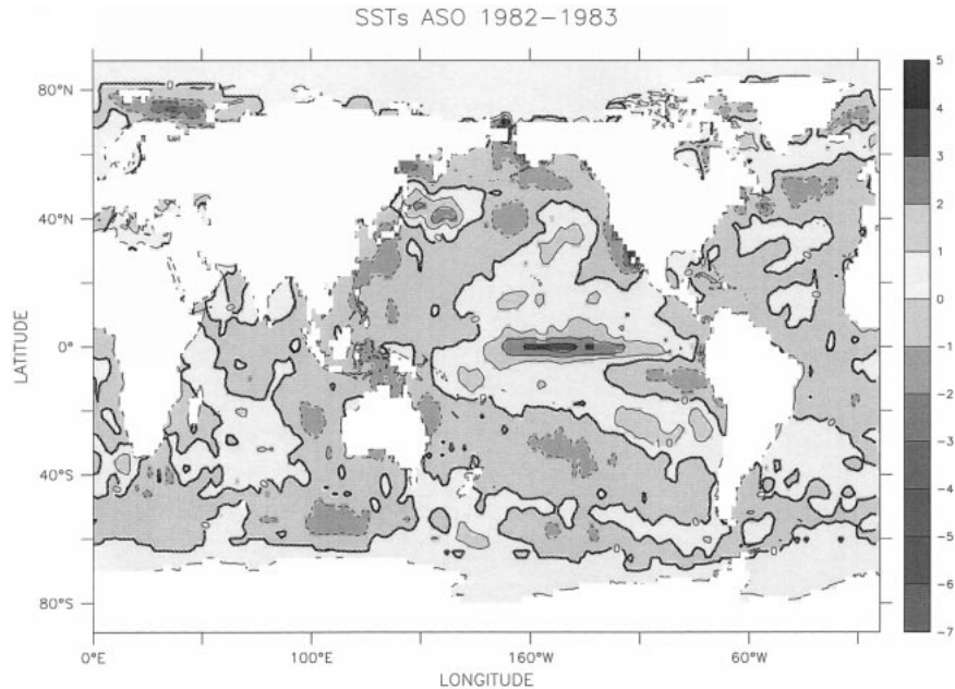
FIG. 1. Difference in Aug–Oct average SSTs (in ^{\circ}\text{C} ) between 1982 and 1983.
