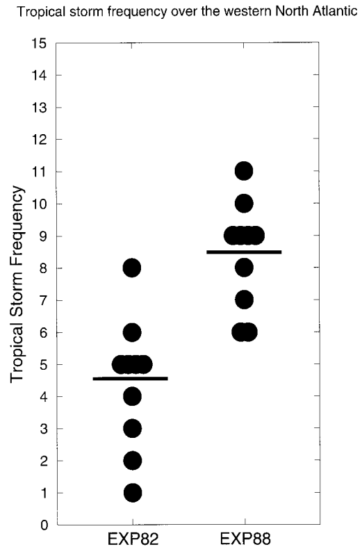
FIG. 3. Ensemble distribution of tropical storm frequency over the western North Atlantic for EXP82 and EXP88. Each circle represents one member of the ensemble. The horizontal line represents the mean of the ensemble.
