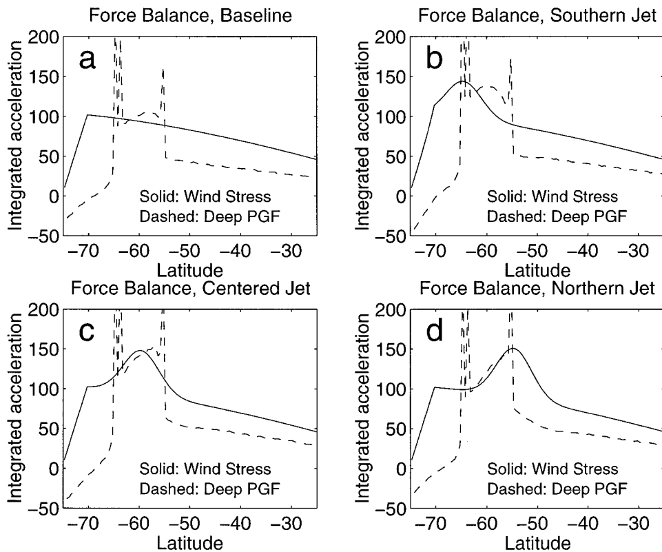
FIG. 7. Balance between the wind stress (solid lines) and the pressure gradient below 2000 m depth (dashed lines) for the four runs with interfacial damping, demonstrating that within the latitudes of the passage ( 65^{\circ} to 55^{\circ} S) these two terms are largely in balance. Strong frictional ageostrophic effects are seen at the edges of the passage. (a) Baseline case, (b) southern jet case, (c) centered jet case, and (d) northern jet case.
