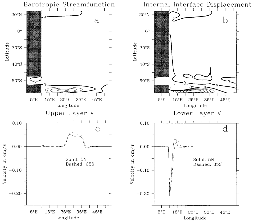
FIG. 8. Same as Fig. 4 but with fixed sources and sinks instead of interfacial damping.
