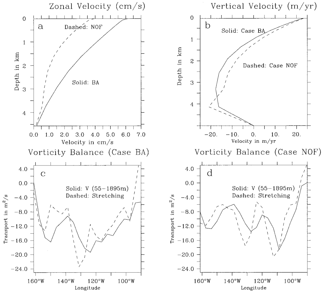
FIG. 12. Velocity changes between the baseline (BA) and negative offset cases (NOF). (a) Averaged zonal velocity at 57.8°S, 160°–90°W (SE Pacific). (b) Averaged vertical velocity from 60° to 55°S. Note that the changes are zero at the upper boundary (where Ekman pumping is important) and relatively small elsewhere in the water column. (c) Geostrophic vorticity balance along 57.8°S for baseline case. Solid line is integrated southward transport from 55 to 1895 m. Dashed line is f/\beta(w|_{55m} - w|_{1895m}) , the transport associated with vortex stretching. (d) Geostrophic vorticity balance for case NOF. Note that there are differences, due to changes in the deep overturning, but that the overall level of transport is similar.
