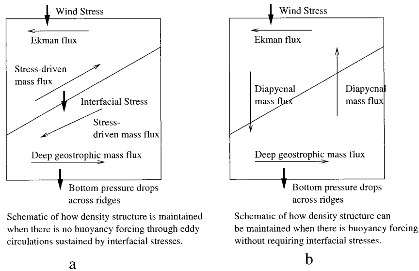
FIG. 2. Illustration of two extreme cases illustrating the relationship between the zonal momentum balance and buoyancy forcing. Light arrows represent mass fluxes. Heavy arrows represent momentum fluxes. (a) A case where there is no diapycnal mass flux between the light and dense layers. In order to establish a steady state, momentum must be fluxed from the upper layer to the lower layer and the mass fluxes generated by the stress between layers must balance the surface Ekman flux and the deep geostrophic mass flux below the ridges. (b) A case where buoyancy forcing allows for diapycnal mass fluxes between the upper and lower layers. This case does not require interfacial stresses to close the momentum balance. Note that in both cases, averaging vertically will yield a balance between wind stress and "form drag."
