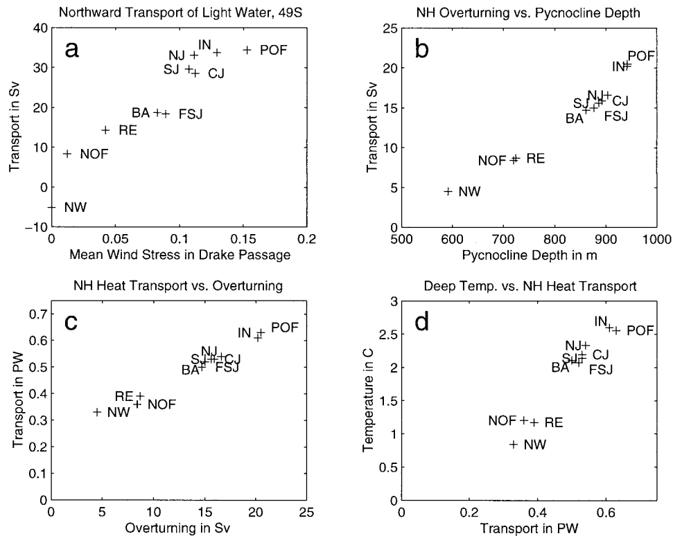
FIG. 14. How Southern Ocean winds produce changes in the ACC: (a) Northward transport of light ( \sigma_0 < 27.2 ) water vs average wind stress in Drake Passage. Note that there is a general trend that as the wind stress increases, the northward transport of light water increases. (b) NH overturning vs pycnocline depth. Note that as the northward transport of light water increases, so does (in general) the overturning. (c) Northward heat transport vs overturning. As the overturning increases, it transports more and more heat northward, so that more water is being transformed. The range of the temperature transformation in the model is about 7.5^\circ\text{C} . (d) Increase in deep temperatures just to the north of the ACC correlated with Northern Hemisphere heat transport. The temperatures to the south change little.
