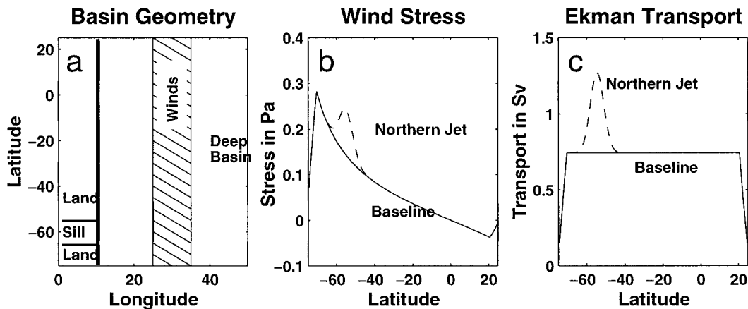
FIG. 3. Schematic of the simple model runs. (a) Model geometry. The basin is reentrant over the sill between 55^{\circ} and 65^{\circ} S. The sill depth is 2000 m and the deep basin is 4000 m deep. Winds are applied within the deep basin only over the hatched portion. (b) Wind stress within the forcing region for two cases, the baseline case with constant Ekman transport everywhere except near the boundaries, and the northern jet case, with a jet of winds centered at 55^{\circ} S. (c) Ekman transport (in Sv) for the two cases in (c).
