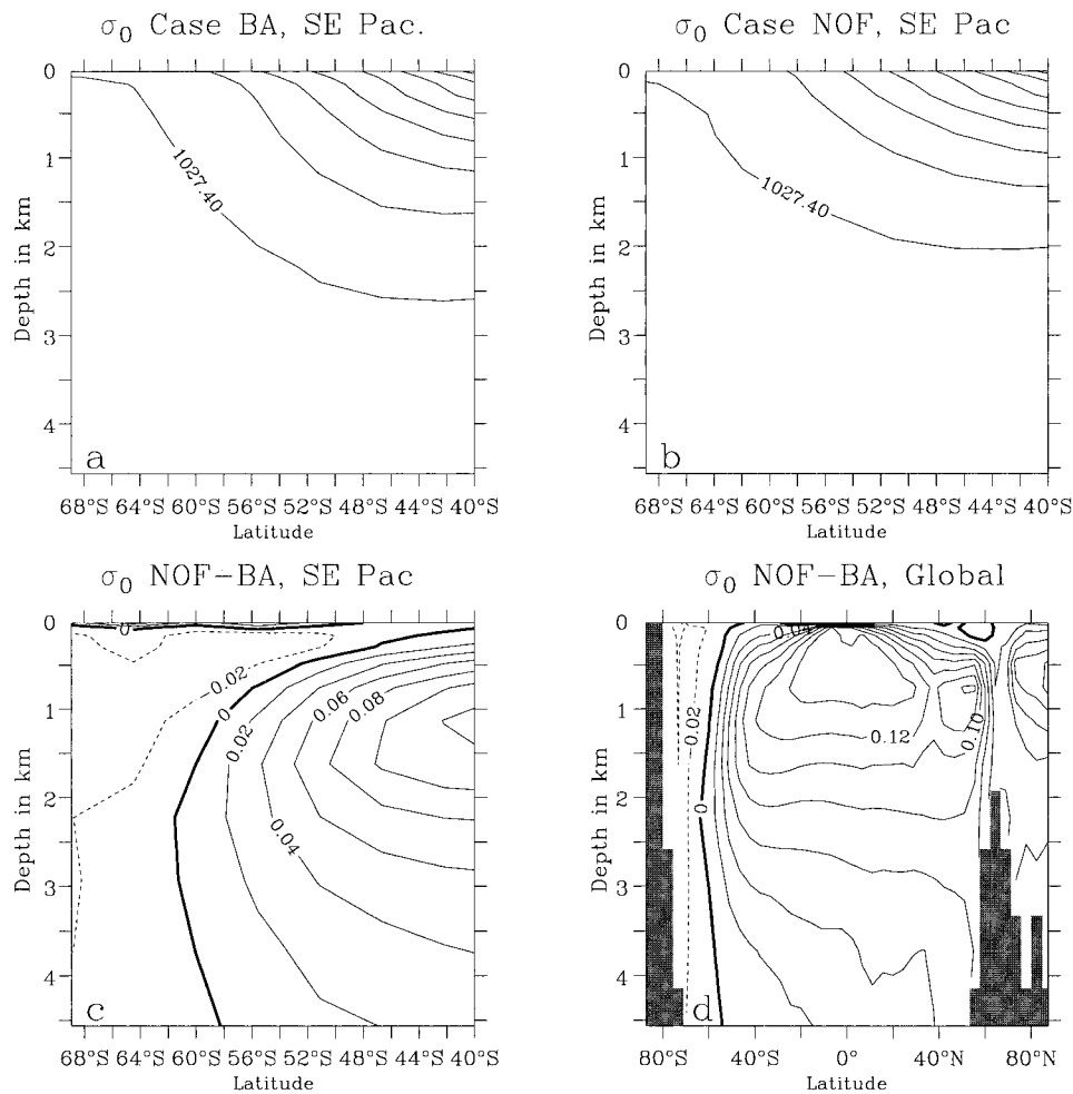
FIG. 13. Illustration of how the density structure changes between the baseline and negative offset case: (a) \sigma_0 for the baseline case in the southeast Pacific, (b) \sigma_0 for the negative offset case, (c) difference in \sigma_0 for the southeast Pacific (negative offset - baseline), and (d) globally averaged difference in \sigma_0 , (negative offset - baseline).
