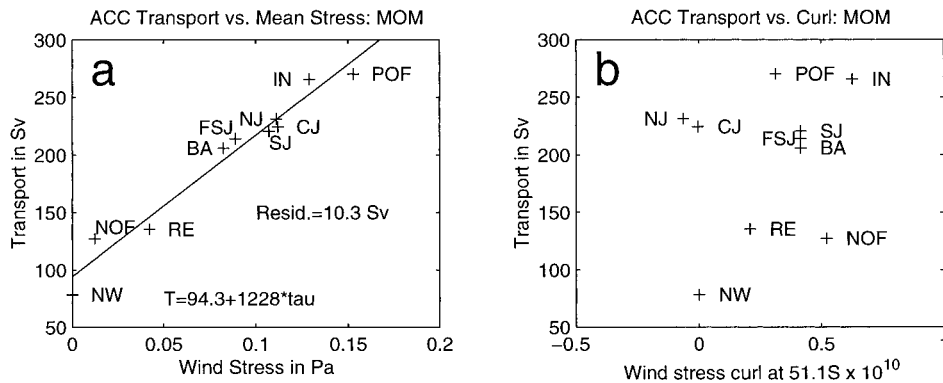
FIG. 9. Regression of the ACC and deep transport in the global runs vs wind stresses. (a) ACC transport vs mean wind stress in channel. (b) ACC transport vs wind stress curl at 51.1°S.
