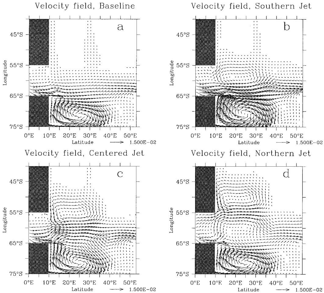
FIG. 6. Velocity fields for the four runs with interfacial damping. Standard vector is 0.015 \text{ m s}^{-1} . (a) Baseline case, (b) southern jet, (c) centered jet, and (d) northern jet.
