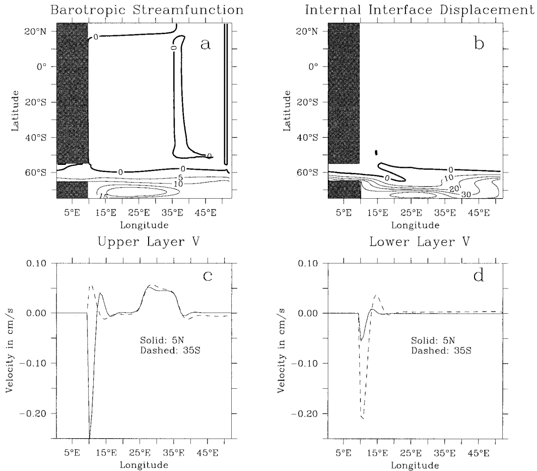
FIG. 4. Solution for the baseline case with interfacial damping. (a) Barotropic streamfunction (in Sv). (b) Interface height displacement (in m). (c) Upper layer meridional velocity at 5°N and 35°S. (d) Lower layer meridional velocity at 5°N and 35°S.
