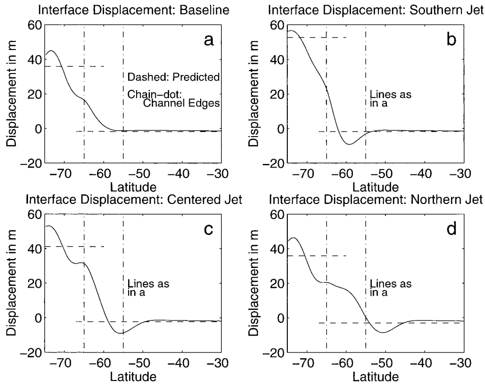
FIG. 5. Internal interface height displacement averaged across the center of the basin for the runs with interfacial restoring. Dashed lines are predicted height displacements from (7) and (8). Chain-dotted lines mark the latitudes of the channel edges.
