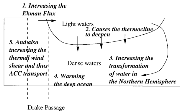
FIG. 1. A conceptual picture of how Southern Hemisphere winds change the depth of the pycnocline, the Northern Hemisphere overturning, and the ACC transport.
