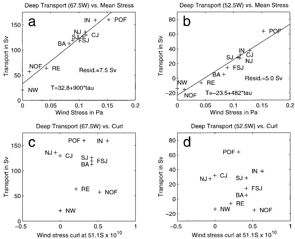
FIG. 10. Regression of the deep transport at two locations vs wind stress and wind stress curl. (a) Deep transport at 67.5°W (in Drake Passage) vs mean wind stress in channel latitudes. (b) Deep transport at 52.5°W vs mean wind stress. (c) Deep transport at 67.5°W transport vs wind stress curl at 51.1°S. (d) Deep transport at 52.5°W vs wind stress curl at 51.1°S.
