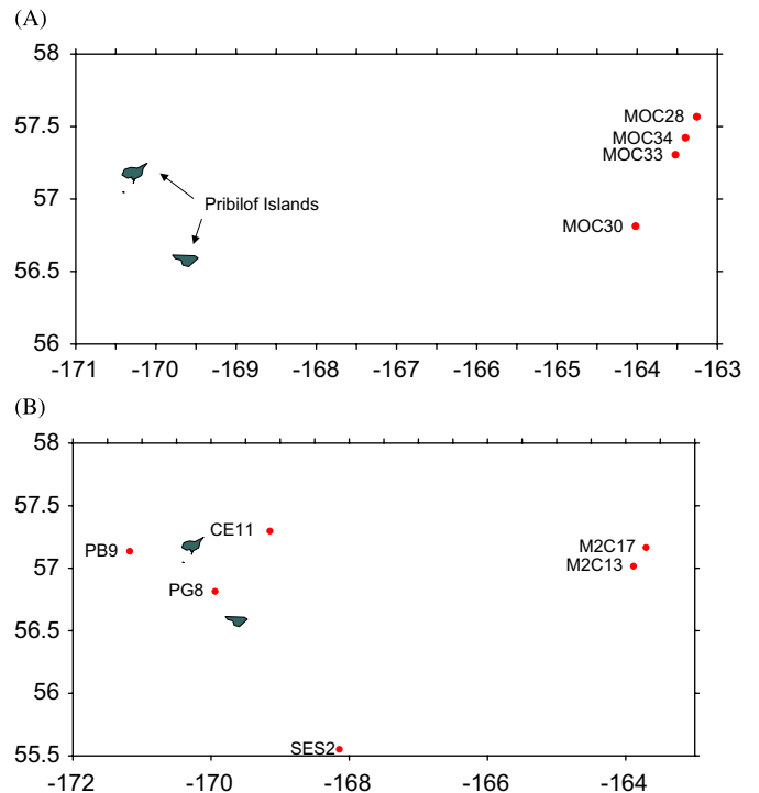
Fig. 9. Location of fish sampling stations on the southeastern Bering Sea shelf in July–August. (A) 1999; (B) 2004.
