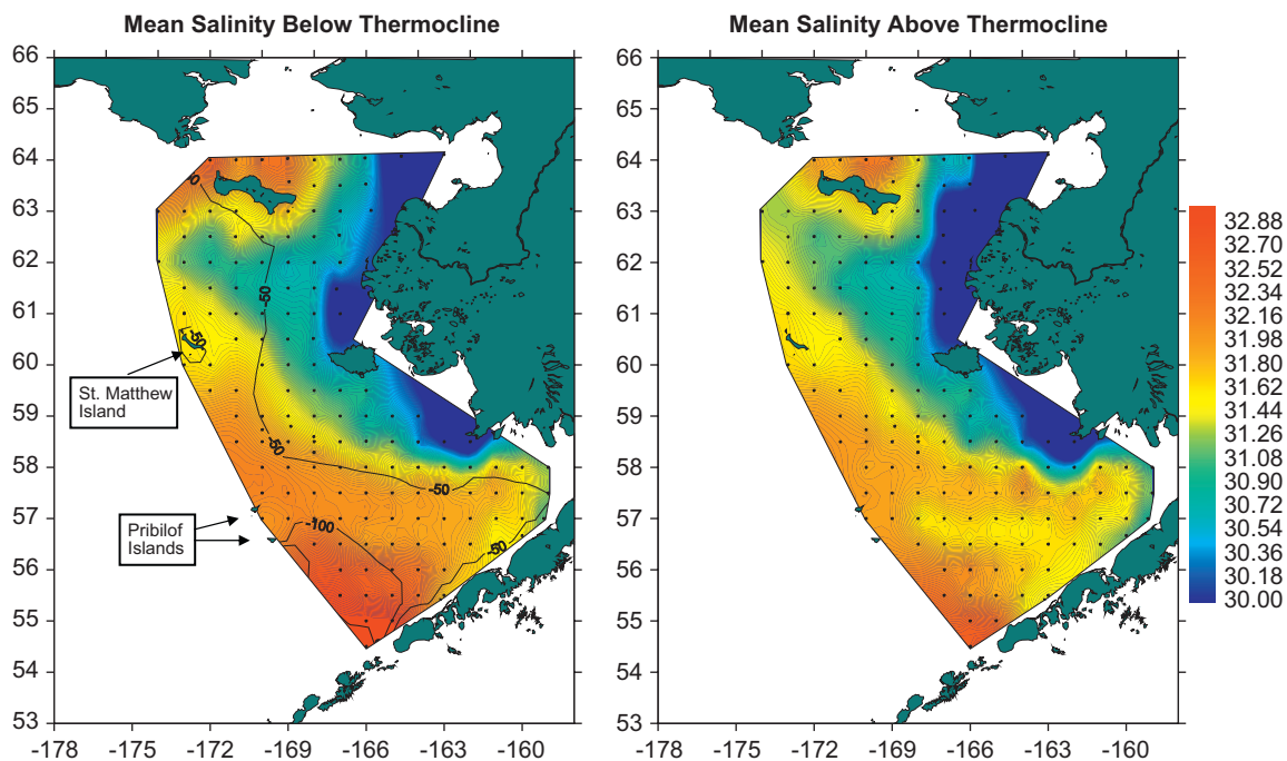
Fig. 15. Mean salinity above and below the thermocline on the eastern Bering Sea shelf in August–September 2004. Black dots indicate station locations; lines indicate 50, 100 and 200-m isobaths (BASIS data).
