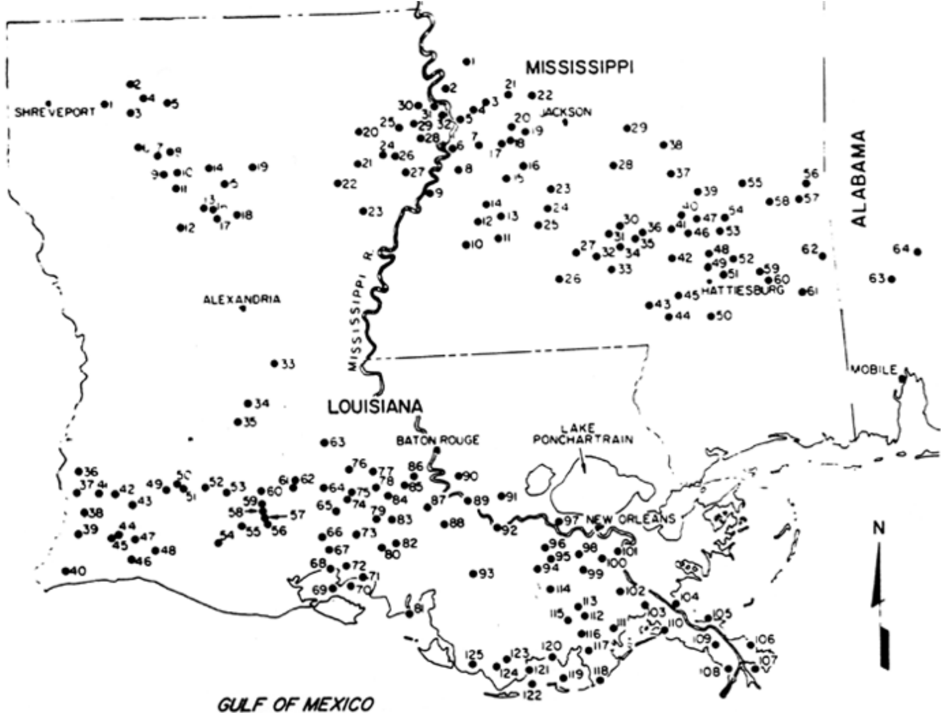
Figure 5 - Location of Louisiana, Mississippi, and Alabama Salt Domes (from Jirik and Weaver 1976)
