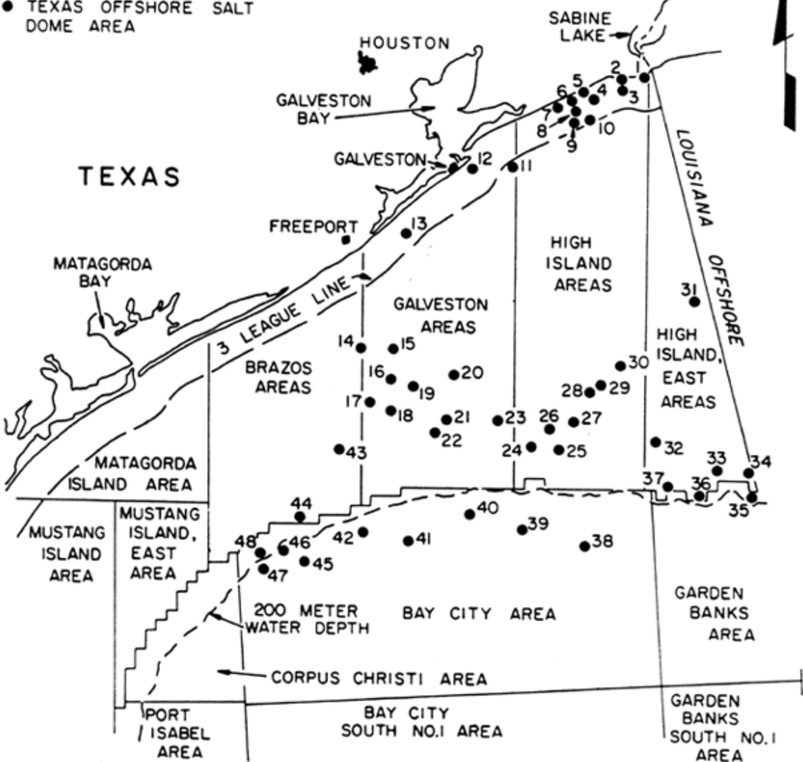
Figure 2 - Location of Texas Offshore Salt Domes (from Jirik and Weaver 1976)
