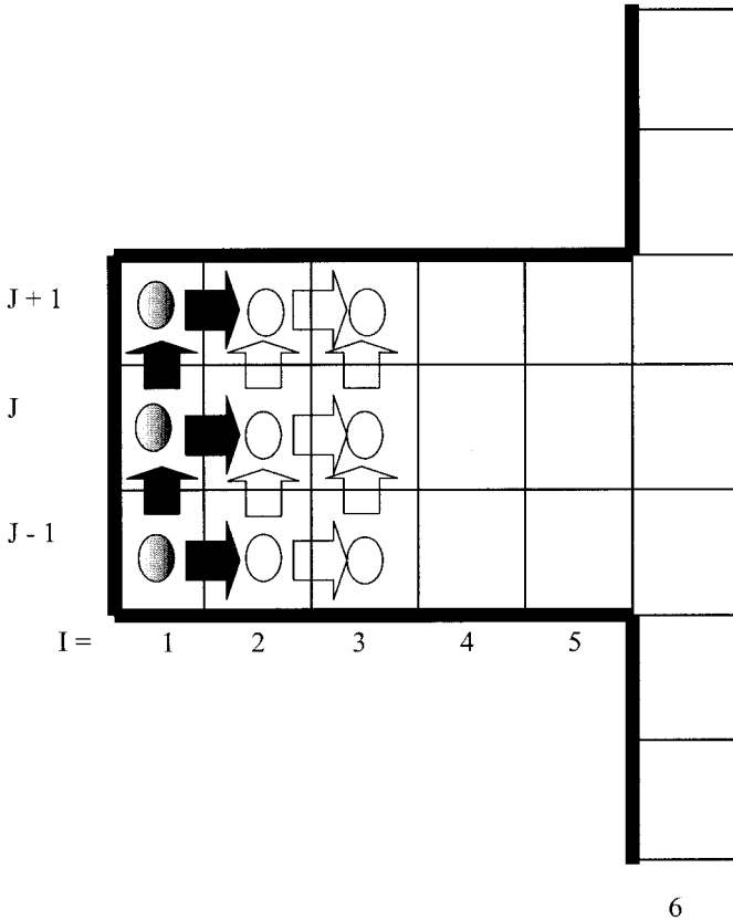
Figure A.2. The schematic of the specified and calculated U, V, and \eta for the IO port ( 26 \leq J \leq 49 ) for I = 1; 2; 3 . The prescribed normal, U(2, J) , and tangential velocities V(1, J) are denoted by black arrows; the computational boundary conditions are \eta(1, J) = \eta(2, J) (denoted by partially filled ovals) and U(1, J) = U(2, J) (not shown). Clear arrows and ovals denote variables that are calculated by using dynamical equations.
