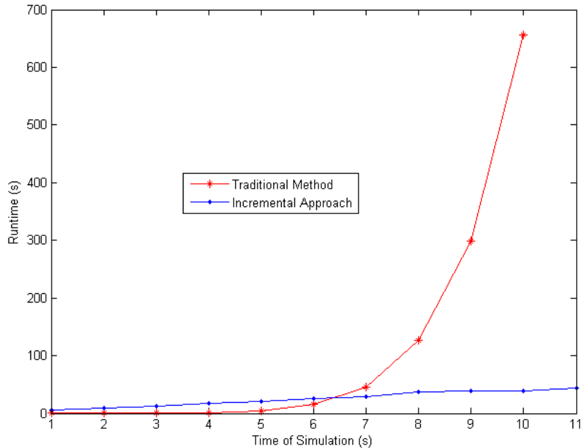
Figure 16. Runtime of traditional method and incremental approach shown as a function of simulation time or space to accommodate simulation. The traditional method reaches a memory limit after ten seconds in this simulation.
