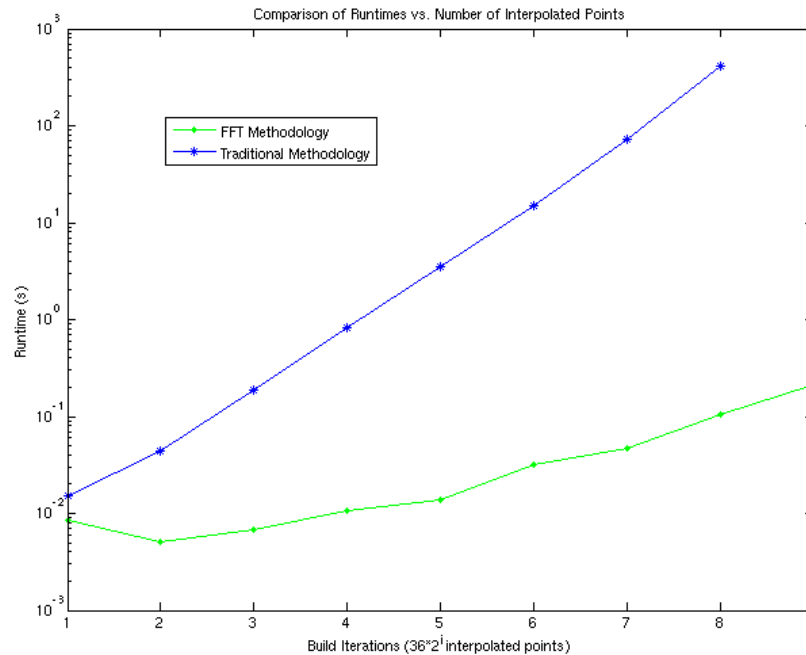
Figure 15. FFT methodology for periodic data shown to be several orders faster than traditional method. The traditional method reaches a memory limit after eight iterations.
