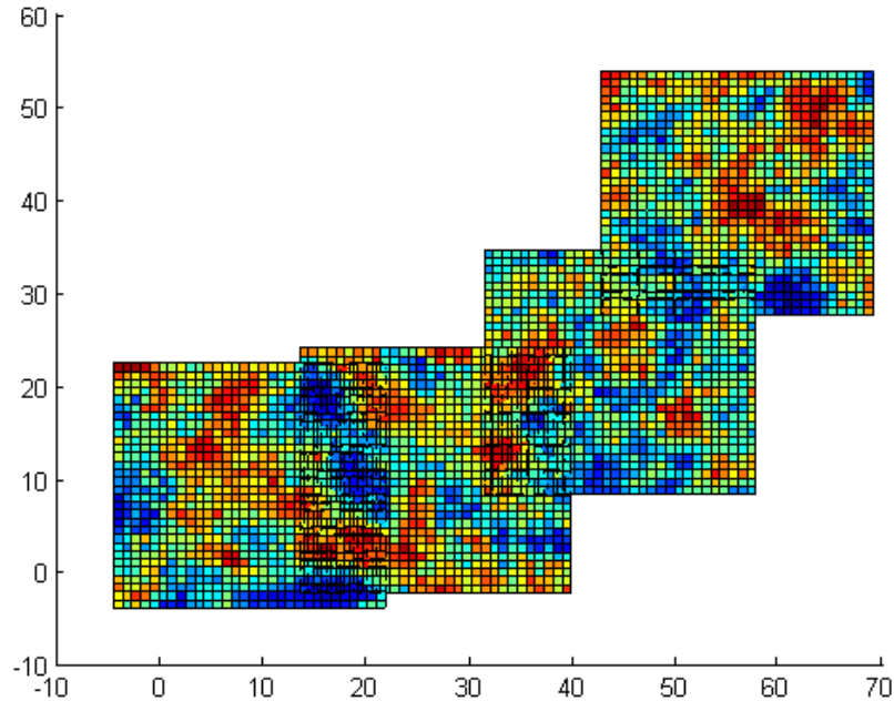
Figure 10. Example of a grid refinement with ICKA.
