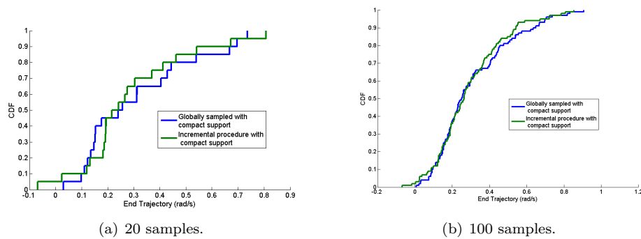
Figure 11. Convergence study of dynamic grid simulation when convergence target uses compact support.
