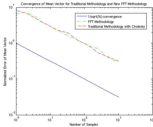
(b) Stationary, high-frequency data: \gamma = 4, \alpha_x = \alpha_y = 1, a_0 = 1, a_1 = a_2 = 0
