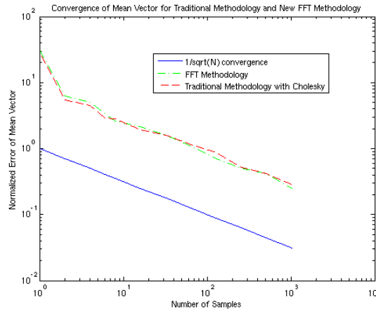
(a) Non-stationary, low-frequency data: \gamma = 4, \alpha_x = \alpha_y = 3, a_0 = 0, a_1 = a_2 = .5
