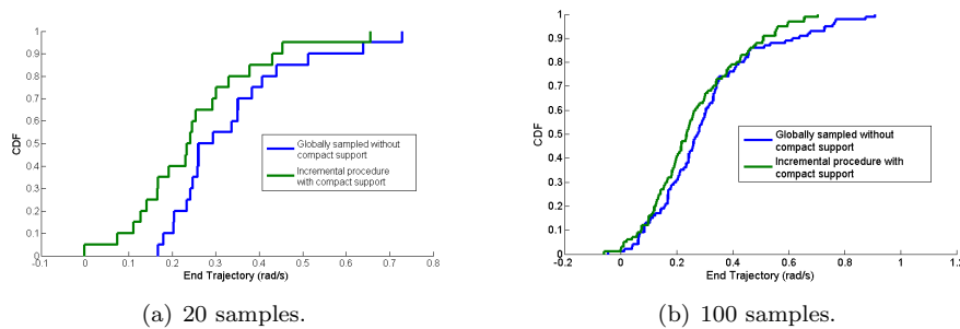
Figure 13. Convergence study of dynamic grid simulation when convergence target uses Eq. 5.
