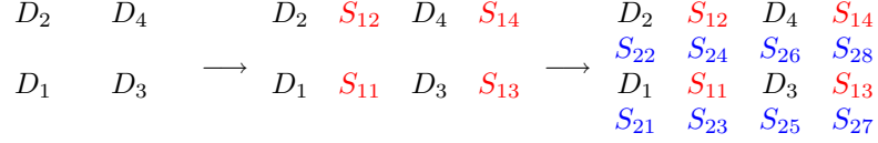
Figure 2. Pictorial representation of first two iterations of sampling method.
