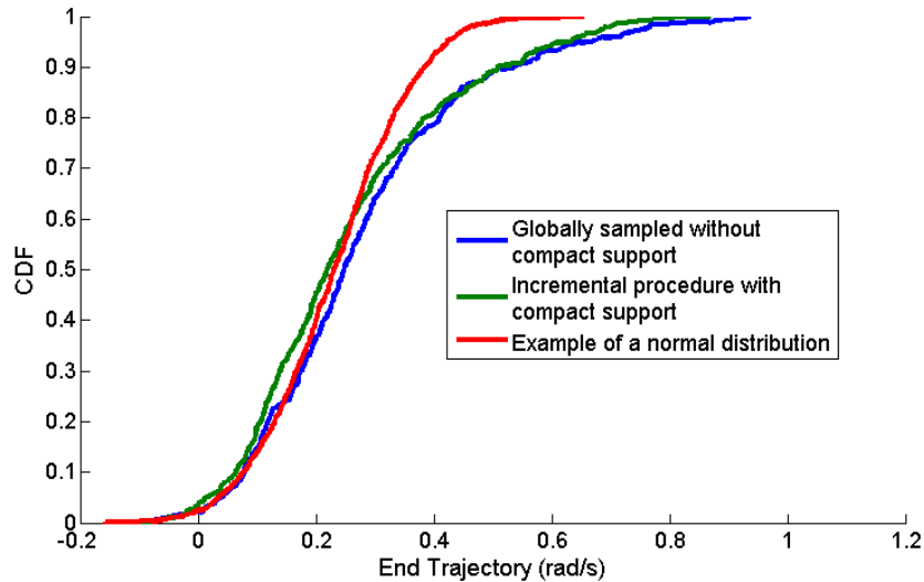
Figure 14. Convergence study of dynamic grid simulation when convergence target uses Eq. 5: 500 samples.
