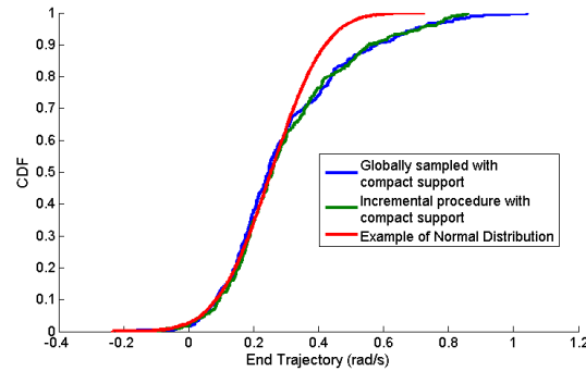
Figure 12. Convergence study of dynamic grid simulation when convergence target uses compact support: 500 samples.
