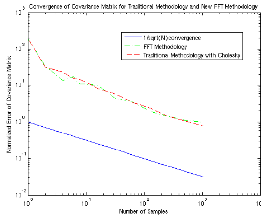
(b) Non-stationary, low-frequency data \gamma = 4, \alpha_x = \alpha_y = 3, a_0 = 0.5, a_1 = a_2 = 0.1 .
