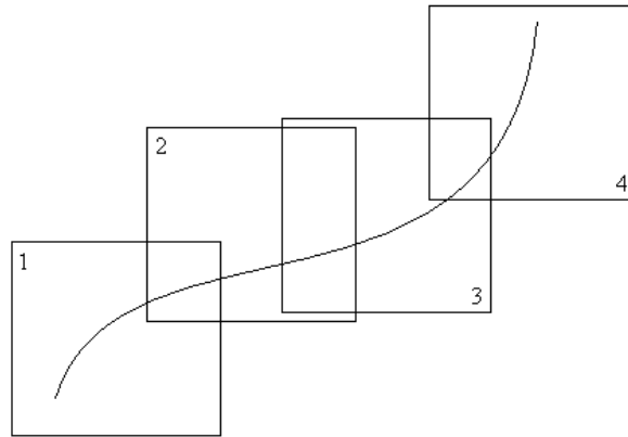
Figure 5. Pictorial representation of incremental sampling procedure.
