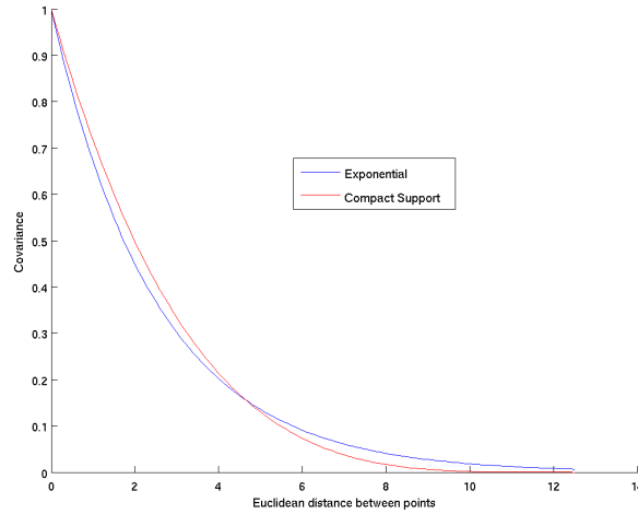
Figure 4. Comparison of exponential kernel and compact kernel; \alpha_{x_1} = \alpha_{x_2} = 2.5 and \epsilon = 12.5 .
