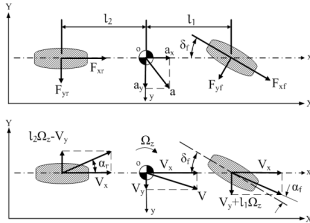
Figure 1. Bicycle model used in preliminary research of methodology [21].
