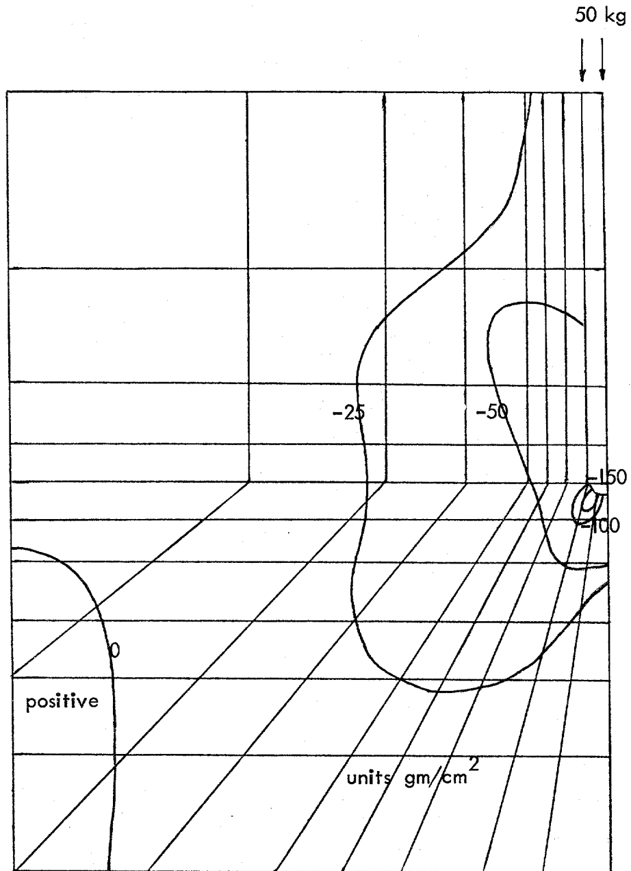
Figure 44. Shear stress contours of pile in soil field - cyclic load, 0 to 50 kg.
