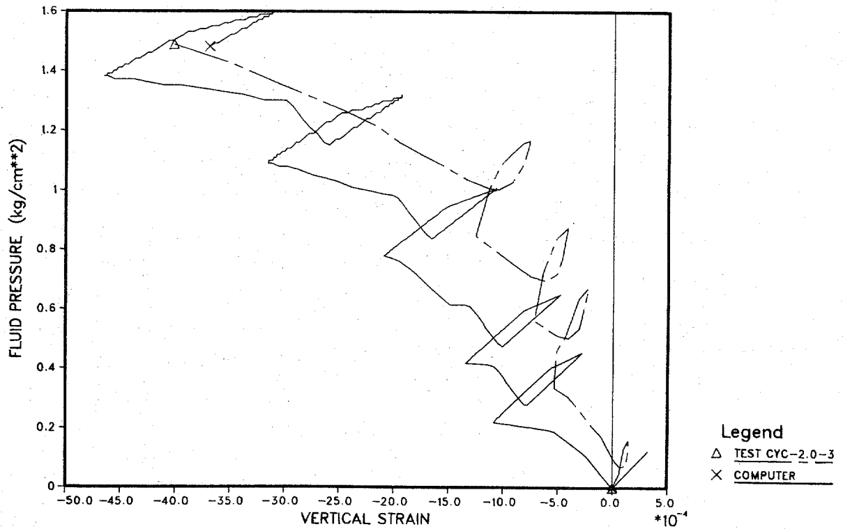
(b) Pore pressure.
