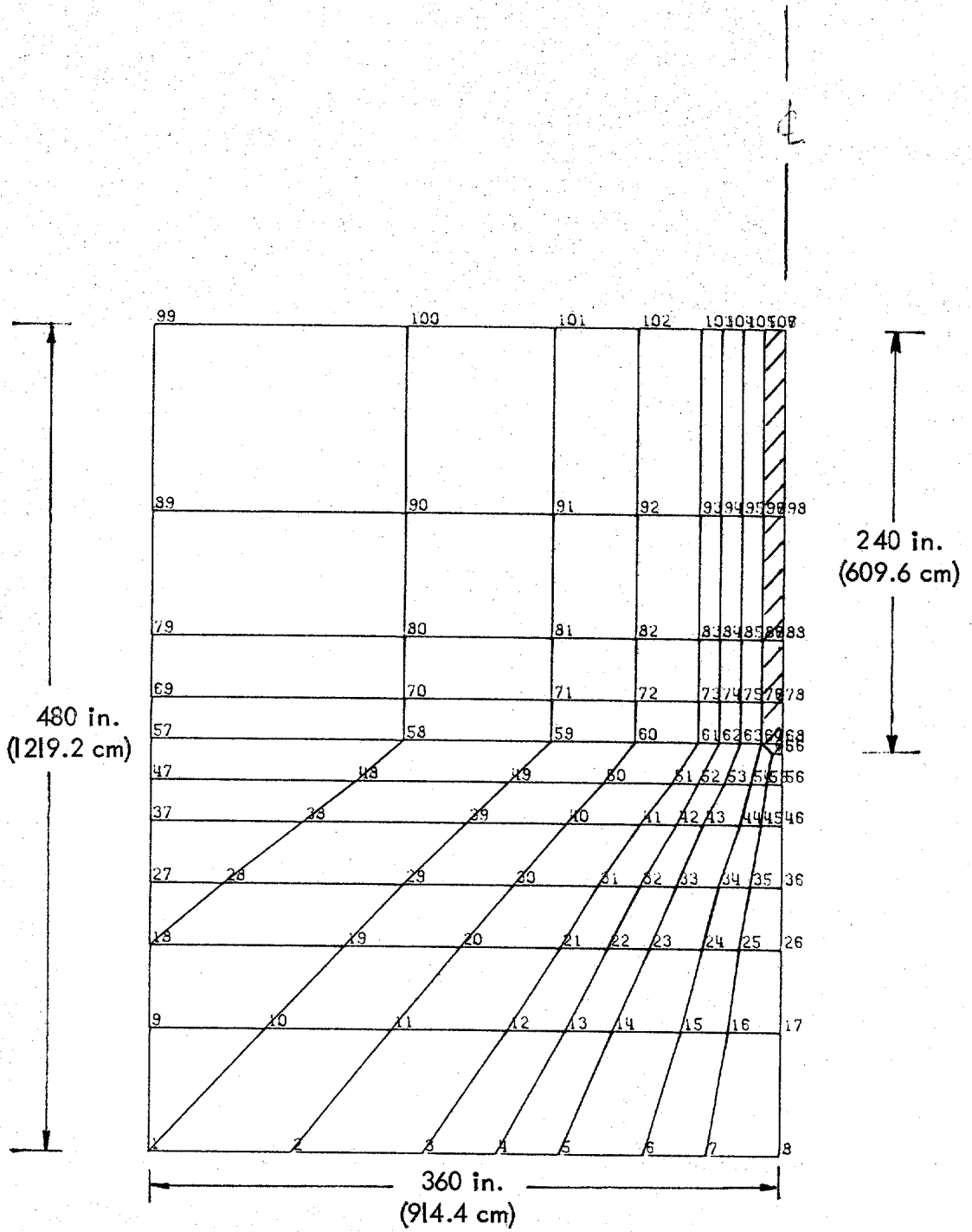
Figure 39. Mesh of pile in soil field.
