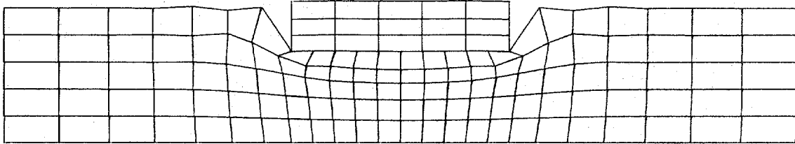
(a) End of static solution, step 5.
