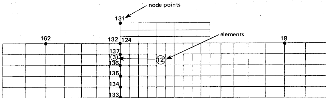
Figure 20. Undeformed mesh.
