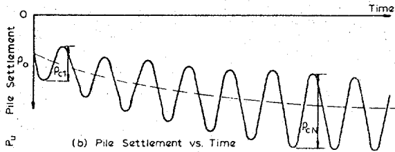
(b) Pile Settlement vs. Time
