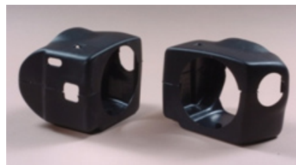
Automotive parts (steering column covers) made with recycled plastics recovered from end-of-life-vehicles.
