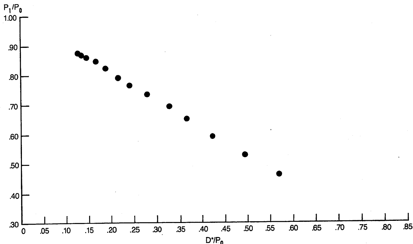
Figure 5-52. PLOT OF POINTS (D^*/P_0, P_1/P_0) DERIVED FROM THE SMOOTHED AGE DISTRIBUTION FROM THE 1961 AND 1971 CENSUSES OF INDIA
