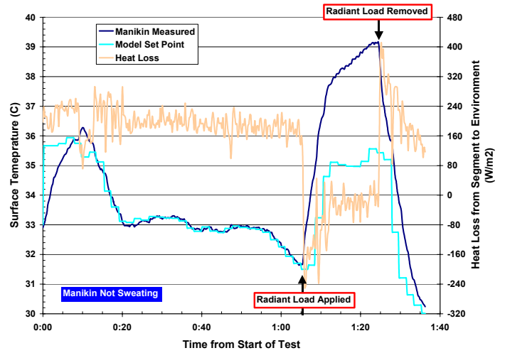
Figure 6. Radiant Heating of a Segment
