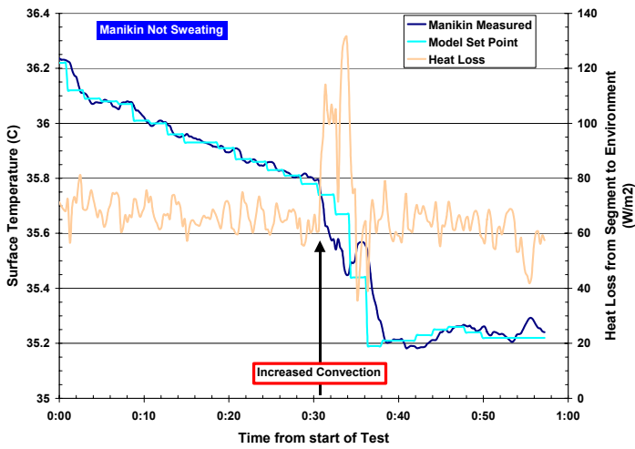
Figure 5. Forced Convection Cooling of a Segment
