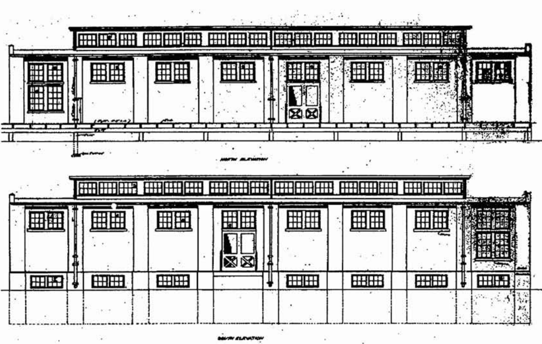
Building No 4, Store House, North and South Elevation
