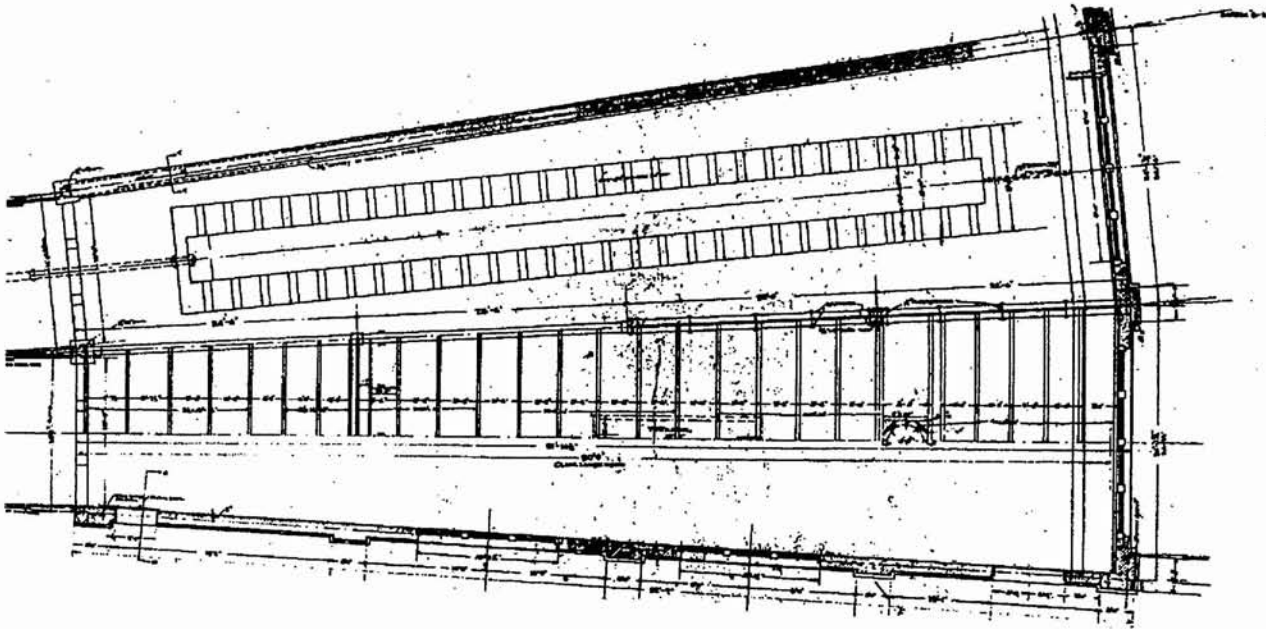
Building No 2, East Roundhouse, Plan, Note: No Window and Door Openings along South Facade
