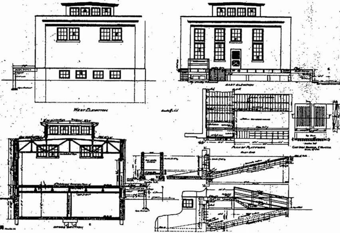
Building No 4, Store House, West and East Elevation and Section
