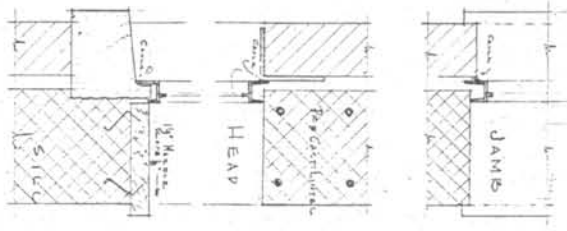
TYPICAL WINDOW DETAILS
