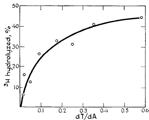
FIG. 5. Influence of \text{d}(\text{T})_{300}:\text{d}(\text{A})_{4000} ratio on hydrolysis of the \text{d}(\text{T})_{300} . Each tube contained, in 0.1 ml, 7 pmoles of ^3\text{H} - \text{d}(\text{T})_{300} , 500 \mu\text{M} dTTP, 4 pmoles of DNA polymerase and 0.5, 0.7, 1, 2, 3, 4, 6, or 8 pmoles of \text{d}(\text{A})_{4000} . The samples were incubated 3 min at 21^\circ . The insoluble material was determined by adsorption to DEAE paper. In control tubes with no dTTP, no hydrolysis was observed ( <4\% ). \text{dT}/\text{dA} is the molar ratio expressed in concentrations of nucleotide residues.
