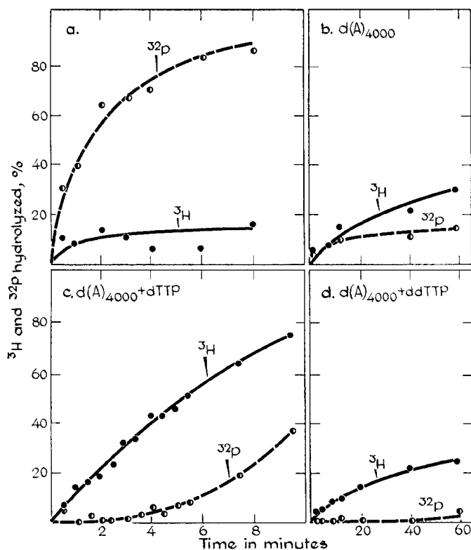
FIG. 6. Rate of degradation by DNA polymerase of ^3\text{H-d(T)}_{200} with 20 ^{32}\text{P} -thymidylate residues at the 3'-end. Each tube contained, in 0.1 ml, 35 pmoles of ^3\text{H} , ^{32}\text{P-d(T)}_{220} ( ^{32}\text{P} , 1 \times 10^8 cpm per \mu\text{mole} ; ^3\text{H} , 2 \times 10^7 cpm per \mu\text{mole} ), 20 pmoles of DNA polymerase, 63 mM phosphate (pH 7.4), and 5 mM \text{MgCl}_2 . Added, as indicated, were 2.5 pmoles of \text{d(A)}_{4000} , 0.5 mM dTTP, and 0.5 mM ddTTP. Samples were removed at intervals and the amount which adsorbed to DEAE paper was measured. Note that the time scales in a and c are 10 times those in b and d .
