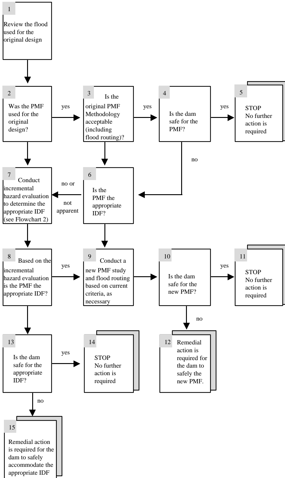
FIGURE 1. FLOWCHART 1 -- PROCEDURES FOR DETERMINING THE APPROPRIATE INFLOW DESIGN FLOOD (IDF) AND THE NEED FOR REMEDIAL ACTION
