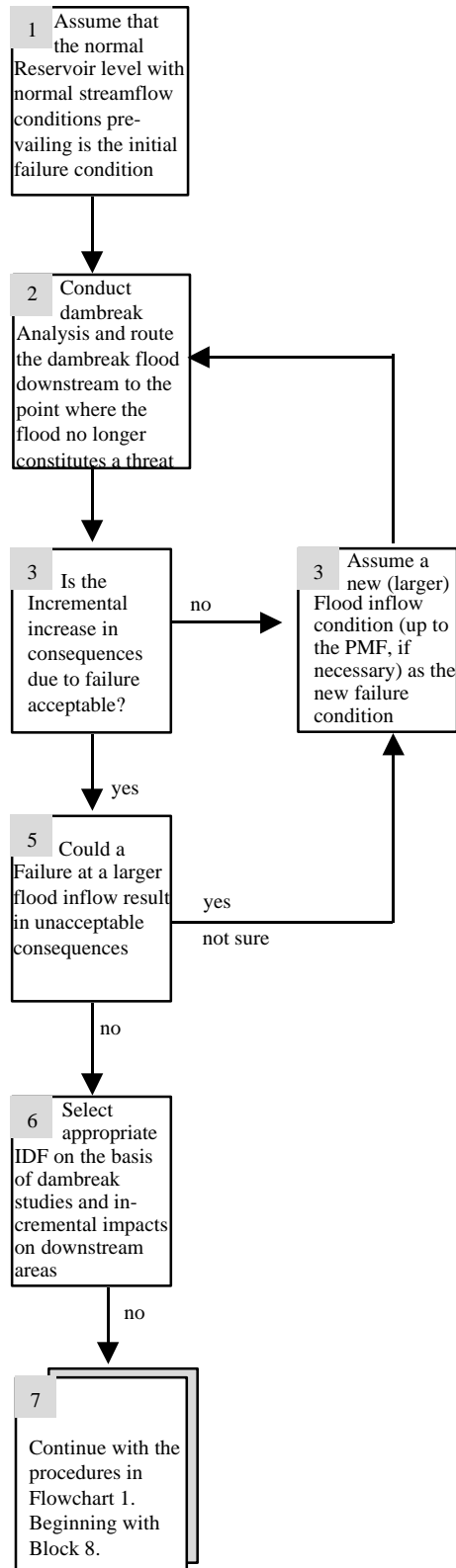
FIGURE 2. FLOWCHART 2 -- PROCEDURES FOR CONDUCTING AN INCREMENTAL HAZARD EVALUATION
