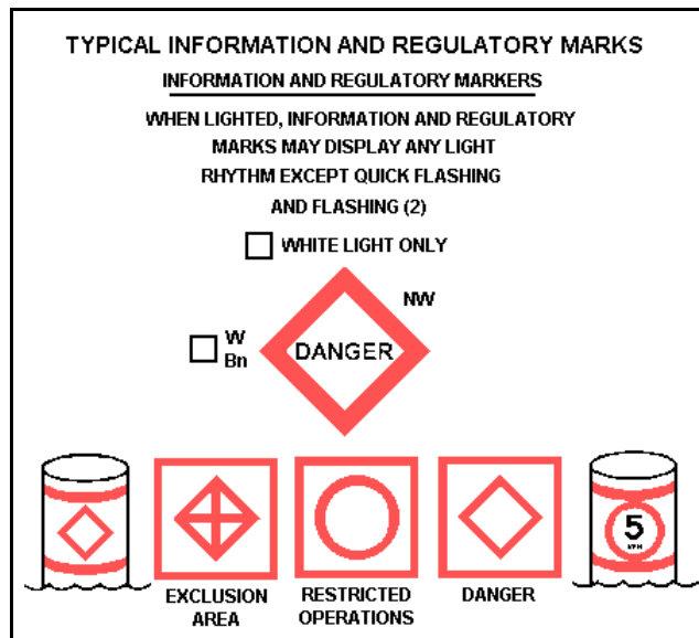
Figure 4. Symbols of the Uniform State Waterway Marking System (Source, USCG web page http://www.uscg.mil/d11/oan/paton/state_buoys.htm accessed March 9, 2001).
