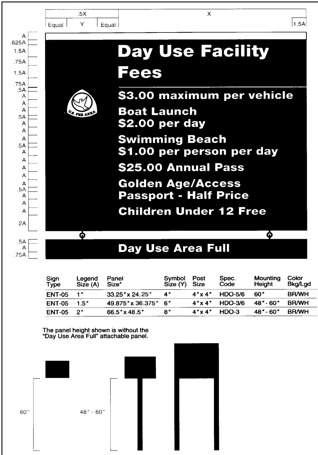
Figure 2. An example of USACE sign design with text heights given in A (the height of the first capital letter in the copy body of the legend text) (Source: USACE, 1995, as modified by the staff)
