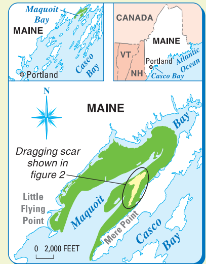
Figure 1. Location of eelgrass beds (shown in green) in Maquoit Bay, Maine.
