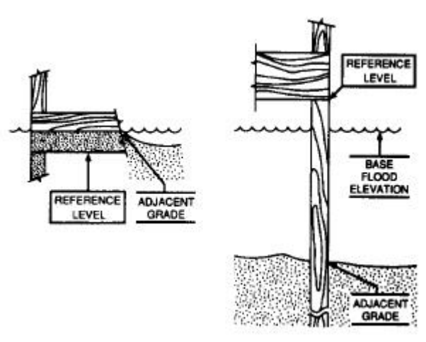
Figure 5-15: In V Zones, the lowest floor is measured from the bottom of the lowest horizontal structural member
