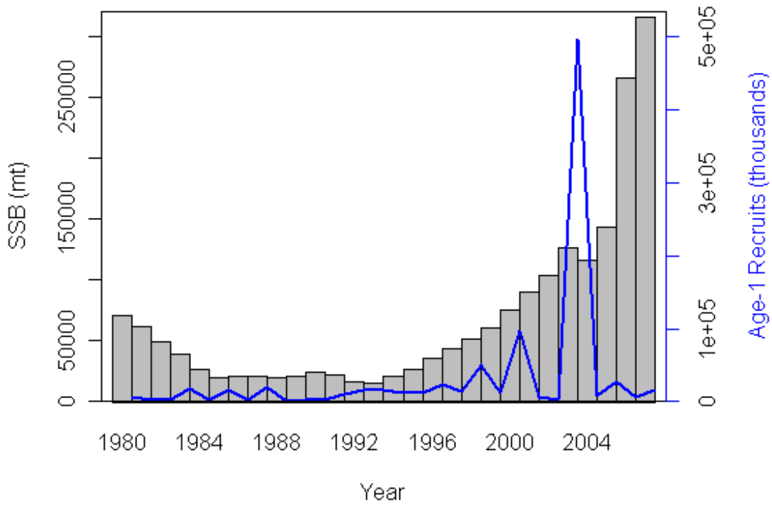
Figure B8. VPA estimates of spawning stock biomass (SSB, mt) and age-1 recruits (thousands) for Georges Bank haddock.
