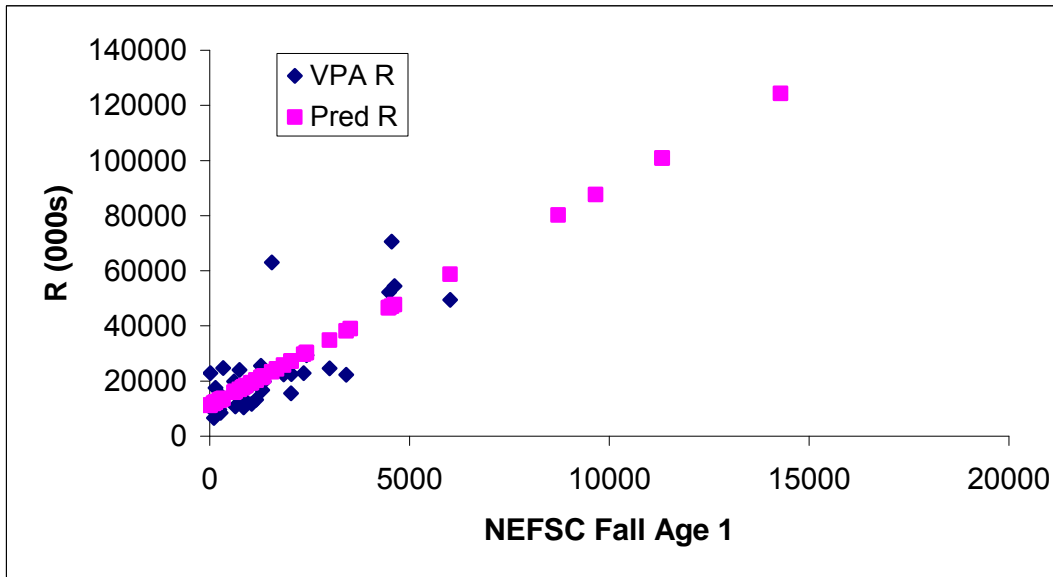
Figure C11. Hindcast estimates of recruitment using the NEFSC Fall survey at age 1.
