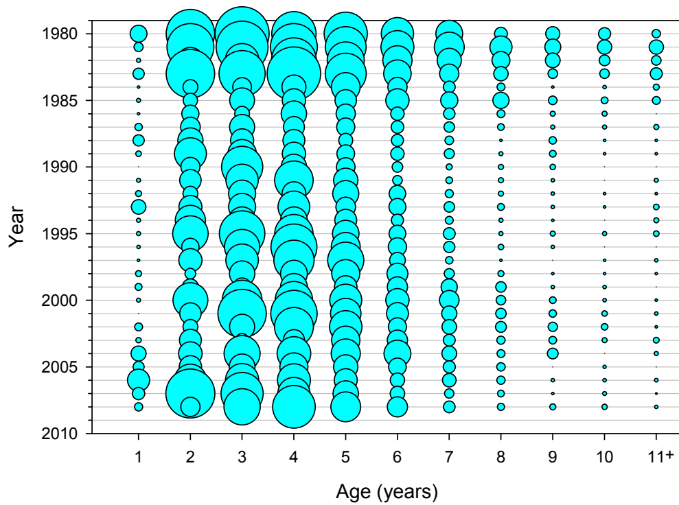
Figure H7. Standardized stratified mean catch per tow at age (numbers) of American plaice in NEFSC spring bottom trawl surveys, 1980-2008.
