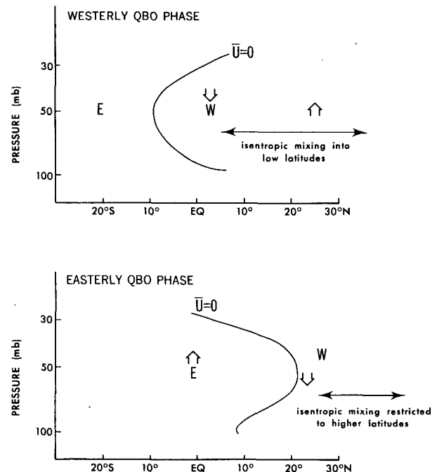
FIG. 2. Schematic diagram showing how the cross-isentropic and along-isentropic (AI) transports may be contributing to the ozone QBO. The top (bottom) panel shows conditions during a boreal winter during the westerly (easterly) phase of the QBO. The wide arrows represent the effects of the QBO-modulated component of the diabatic circulation. The thin arrows are meant to represent the extent of significant AI mixing. In the proposed scheme the AI transport of ozone-rich air from midlatitudes acts to reinforce the maximum in low latitude ozone seen in the westerly phase of the QBO.
