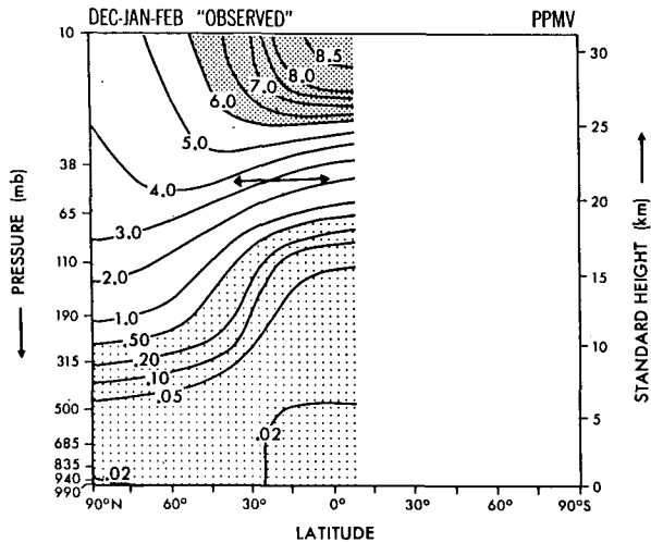
FIG. 1. Climatology of zonal mean ozone mixing ratio for Northern Hemisphere winter. Contours are labelled in parts per million by volume. The heavy arrow is a schematic representation of an isentropic surface. Adapted from Mahlman et al. (1980).
