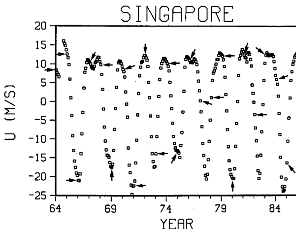
FIG. 5. Time series of monthly mean zonal 50 mb wind at Singapore (1.3°N, 103.9°E) deseasonalized and smoothed as in Fig. 3.
