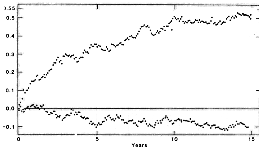
Fig. 1. The normalized response of the globally averaged sea surface temperature plotted at 30-day intervals (upper curve); the response for a calibration experiment (lower curve).
