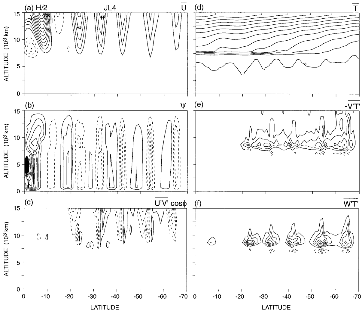
Fig. D3. Meridional sections of the primary fields and eddy transports for the jovian LIN case JL4, a transitional system. The means are based on daily averages taken over 1400–1500 days. In order, the contour interval, maximum and minimum values are (a) (10, 126, -31 ) \text{m s}^{-1} ; (b) (5, 42.4, -30.5) \times 10^3 \text{ m}^2 \text{ s}^{-1} ; (c) (1, 3.4, -6.0 ) \text{m}^2 \text{ s}^{-2} ; (d) (5, 69, -0) \times 10^{-2} \text{ }^\circ\text{C} ; (e) (1, 4.4, -2.3) \times 10^{-3} \text{ }^\circ\text{C m s}^{-1} ; (f) (1, 6.1, -4.3) \times 10^{-4} \text{ }^\circ\text{C m s}^{-1} . The zero-value contours are omitted for the eddy fields.
