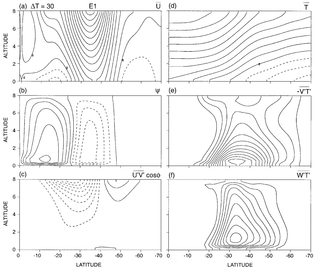
Fig. C1. Meridional sections of the primary fields and eddy transports for the basic terrestrial E1 case with a low baroclinicity ( \Delta T ). The means are based on daily averages taken over 900–1000 days. In order, the contour interval, maximum and minimum values are (a) (2, 29, -4 ) \text{m s}^{-1} ; (b) (1.5, 2, -3.5) \times 10^2 \text{ m}^2 \text{ s}^{-1} ; (c) (2, 6.0, -17.4 ) \text{m}^2 \text{ s}^{-2} ; (d) (4, 44, -13 ) ^\circ\text{C} ; (e) (0.5, 6.8, -0.1 ) ^\circ\text{C m s}^{-1} ; (f) (0.5, 4.7, -0.1) \times 10^{-3} \text{ C m s}^{-1} . The zero-value contours are omitted for the eddy fields.
