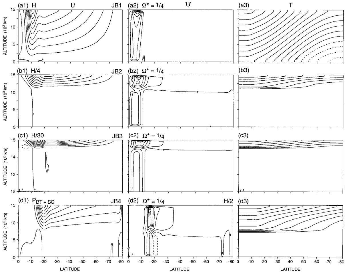
Fig. B2. Meridional sections of the zonal velocity, streamfunction, and temperature for the jovian axisymmetric cases with different thicknesses (JB1–JB3) and a different heating profile (JB4). In order, the contour interval, maximum and minimum values are (a1) (10, 95, -1) m s -1 ; (a2) (10, 58, -0) × 10 3 m 2 s -1 ; (a3) (1, 14, -4) × 10 -2 °C; (b1) (10, 82, -8) m s -1 ; (b2) (2, 11, -2) × 10 3 m 2 s -1 ; (b3) (1, 7.6, 0) × 10 -1 °C; (c1) (10, 104, -15) m s -1 ; (c2) (4, 21, -3) × 10 2 m 2 s -1 ; (c3) (1, 7.6, -0)°C; (d1) (10, 85, -2) m s -1 ; (d2) (10, 68, -14) × 10 2 m 2 s -1 ; (d3) (4, 39, 0) × 10 -2 °C.
