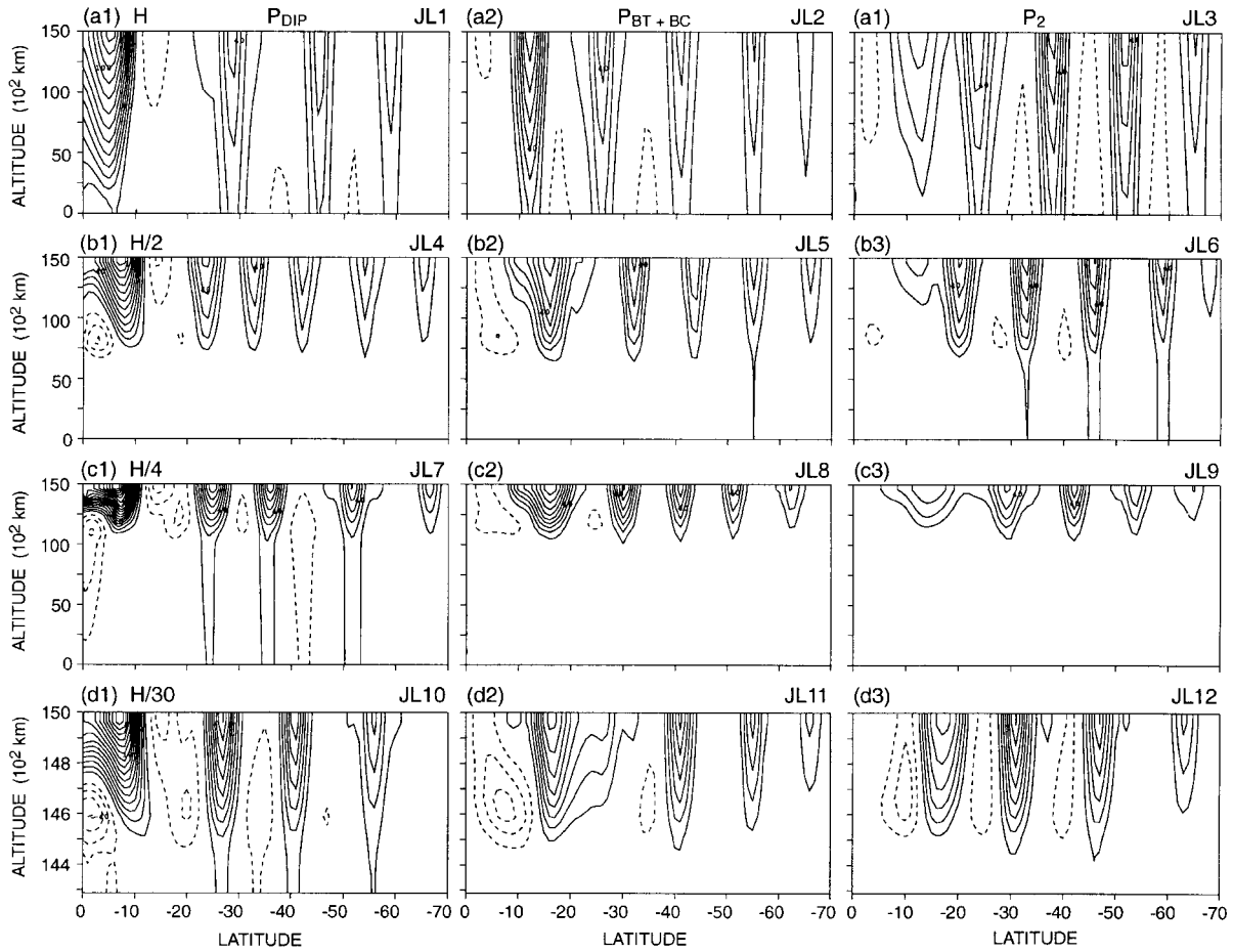
Fig. D1. Meridional zonal velocity sections for the jovian LIN cases, JL1–JL12, with different heating thicknesses and latitudinal profiles. The contour interval equals 10 \text{ m s}^{-1} for all, while the maximum and minimum values and daily averaging intervals are (a1) (134, -19) \text{ m s}^{-1} , 9900–10000 days; (a2) (79, -15) \text{ m s}^{-1} , 3400–3500 days; (a3) (65, -18) \text{ m s}^{-1} , 1400–1500 days; (b1) (126, -31) \text{ m s}^{-1} , 1400–1500 days; (b2) (75, -20) \text{ m s}^{-1} , 1900–2000 days; (b3) (66, -13) \text{ m s}^{-1} , 1400–1500 days; (c1) (176, -34) \text{ m s}^{-1} , 2800–3000 days; (c2) (97, -18) \text{ m s}^{-1} , 2400–2500 days; (c3) (58, -9) \text{ m s}^{-1} , 1400–1500 days; (d1) (166, -41) \text{ m s}^{-1} , 6900–7000 days; (d2) (83, -34) \text{ m s}^{-1} , 1450–1500 days; (d3) (81, -25) \text{ m s}^{-1} , 3950–4000 days. The zero-value contours are omitted.
