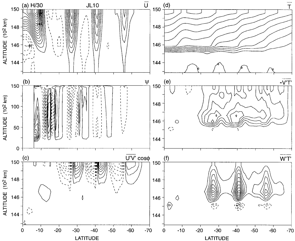
Fig. D4. Meridional sections of the primary fields and eddy transports for the jovian LIN case JL10, a thin system. The means are based on daily averages taken over 100–7000 days. In order, the contour interval, maximum and minimum values are (a) (10, 166, -41 ) \text{m s}^{-1} ; (b) (1, 8.1, -5.3 ) \times 10^3 \text{ m}^2 \text{ s}^{-1} ; (c) (2, 14.2, -17.9 ) \text{m}^2 \text{ s}^{-2} ; (d) (0.8, 9.8, -0 ) ^\circ\text{C} ; (e) (2, 12.4, -2.9 ) \times 10^{-2} \text{ }^\circ\text{C m s}^{-1} ; (f) (2, 19.3, -10.7 ) \times 10^{-4} \text{ }^\circ\text{C m s}^{-1} . The zero-value contours are omitted for the eddy fields. The streamfunction plot skips low latitudes.
