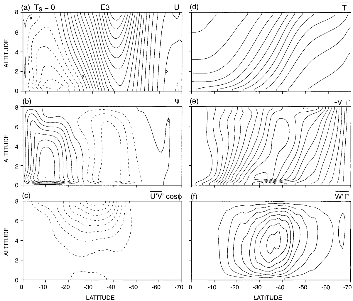
Fig. C3. Meridional sections of the primary fields and eddy transports for the terrestrial E3 case with no background static stability. The means are based on daily averages taken over 800–1000 days. In order, the contour interval, maximum and minimum values are (a) (2, 32, -11 ) \text{m s}^{-1} ; (b) (2, 14.0, -7.2 ) \times 10^2 \text{ m}^2 \text{ s}^{-1} ; (c) (5, 3.2, -43.1 ) \text{m}^2 \text{ s}^{-2} ; (d) (2, 29, 2) ^{\circ}\text{C} ; (e) (0.5, 6.7, -0.1 ) ^{\circ}\text{C m s}^{-1} ; (f) (2, 16.8, -1.5 ) \times 10^{-3} ^{\circ}\text{C m s}^{-1} . The zero-value contours are omitted for the eddy fields.
