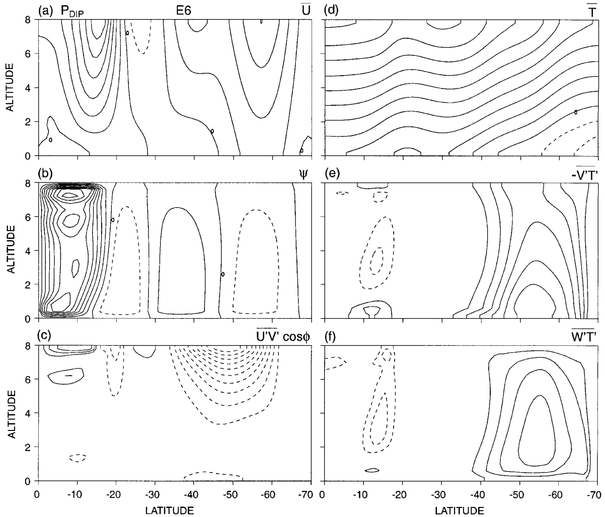
Fig. C6. Meridional sections of the primary fields and eddy transports for the terrestrial E6 case with double jets produced by an extra baroclinicity in low latitudes. The means are based on daily averages taken over 800–1000 days. In order, the contour interval, maximum and minimum values are (a) (5, 35, –8) m s -1 ; (b) (1, 9.5, –2.0) × 10 2 m 2 s -1 ; (c) (1, 3.9, –10.8) m 2 s -2 ; (d) (4, 45, –11) °C; (e) (0.5, 3.5, –1.1) °C m s -1 ; (f) (0.5, 2.3, –1.4) × 10 -3 °C m s -1 . The zero-value contours are omitted for the eddy fields.
