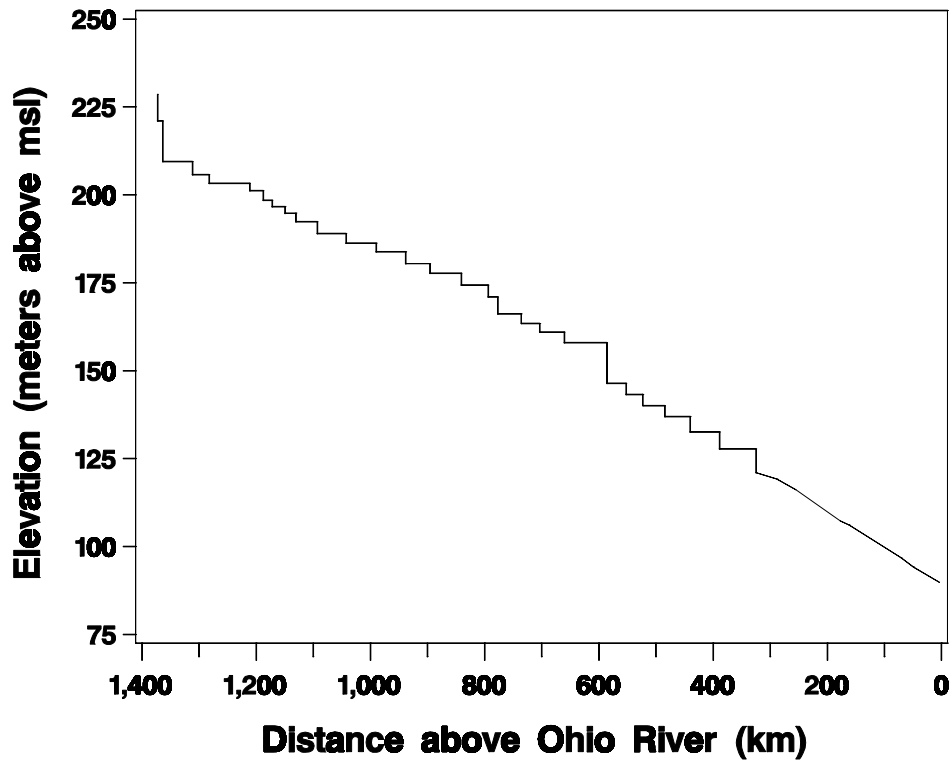
Figure 2. Water surface elevation (meters above mean sea level [msl]) of the Mississippi River from the head of navigation near St. Paul, Minnesota, to the confluence of the Ohio River near Cairo, Illinois.
