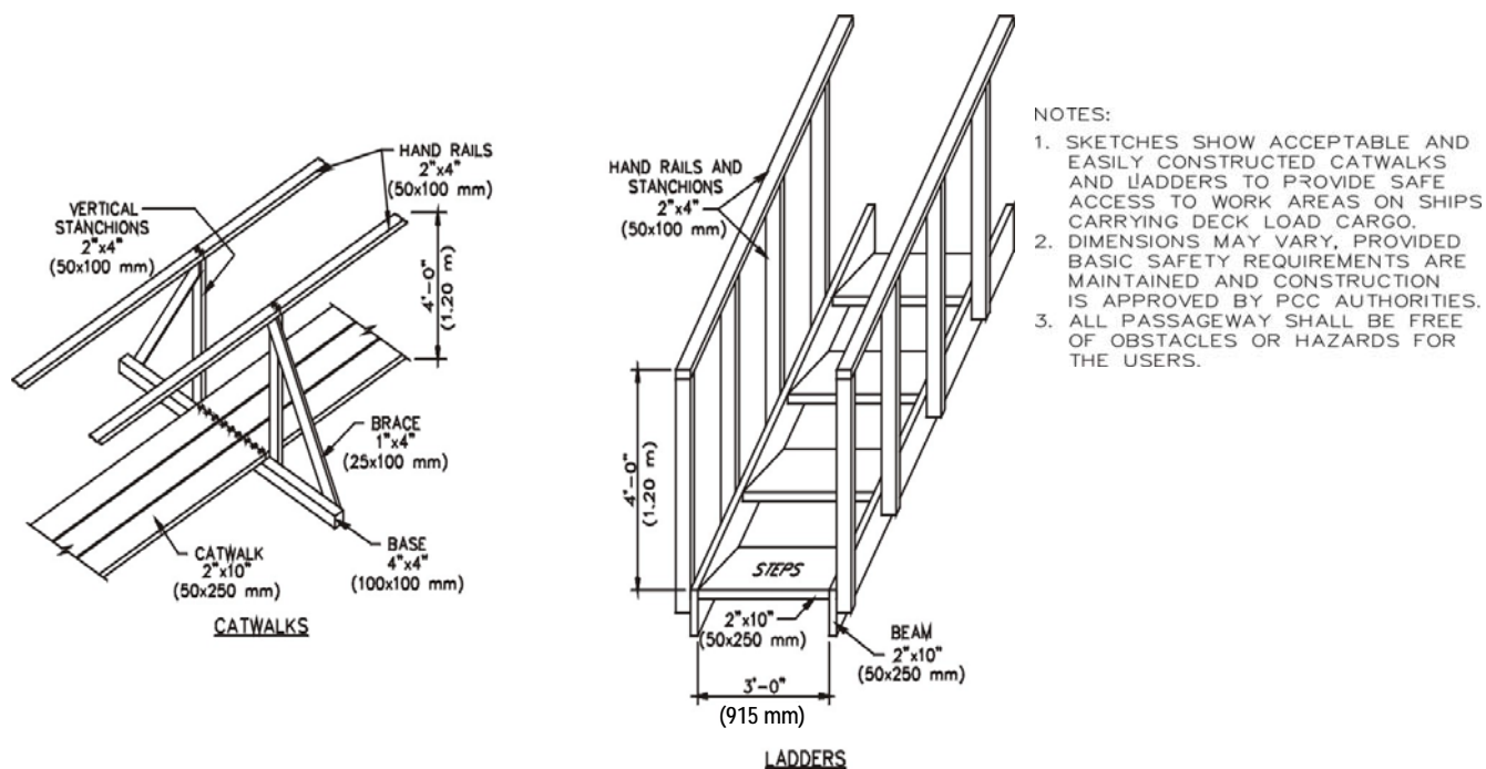
FIGURE 5 - Catwalk and Ladder Sketches
