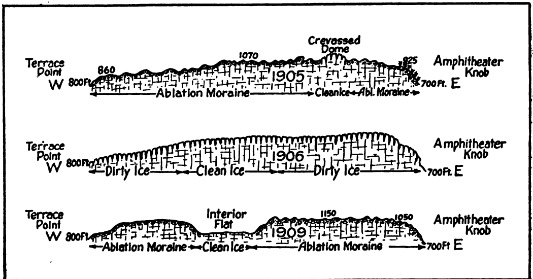
FIG. 5. CROSS-SECTIONS OF ATREVIDA GLACIER.
