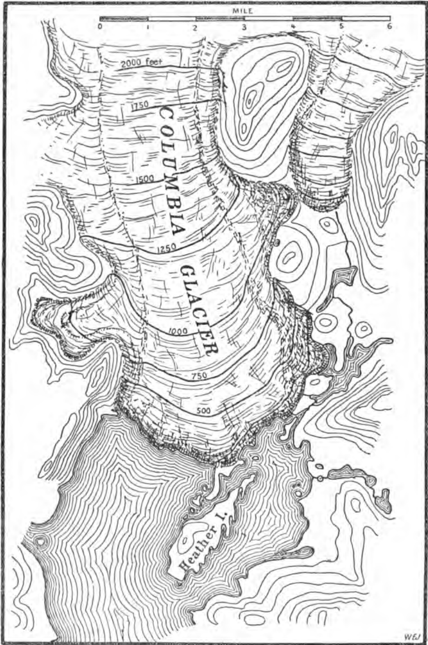
FIG. 29. GILBERT'S MAP OF COLUMBIA GLACIER IN 1899.
