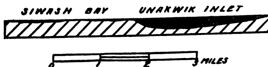
FIG. 39. NATURAL SCALE CROSS-SECTION OF UNAKWIK INLET.
