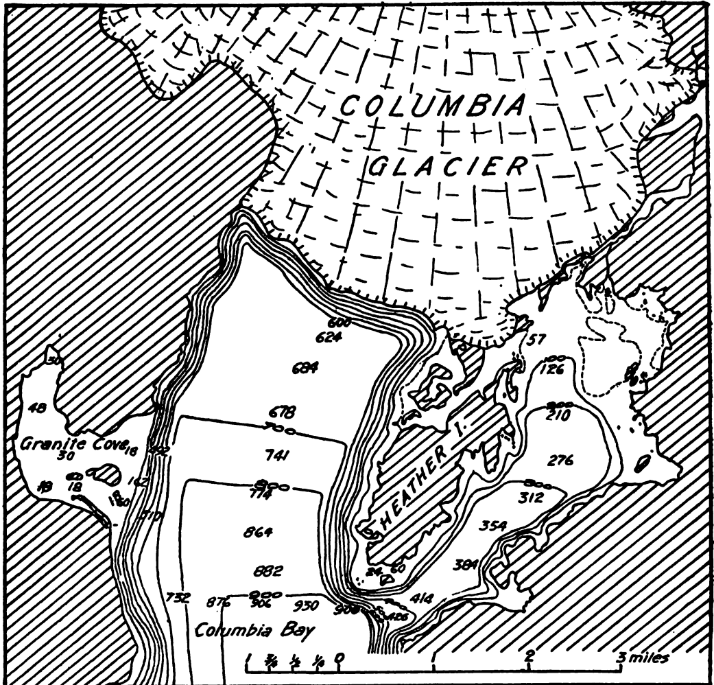
FIG. 35. SUBMARINE CONTOURS IN FRONT OF COLUMBIA GLACIER.
