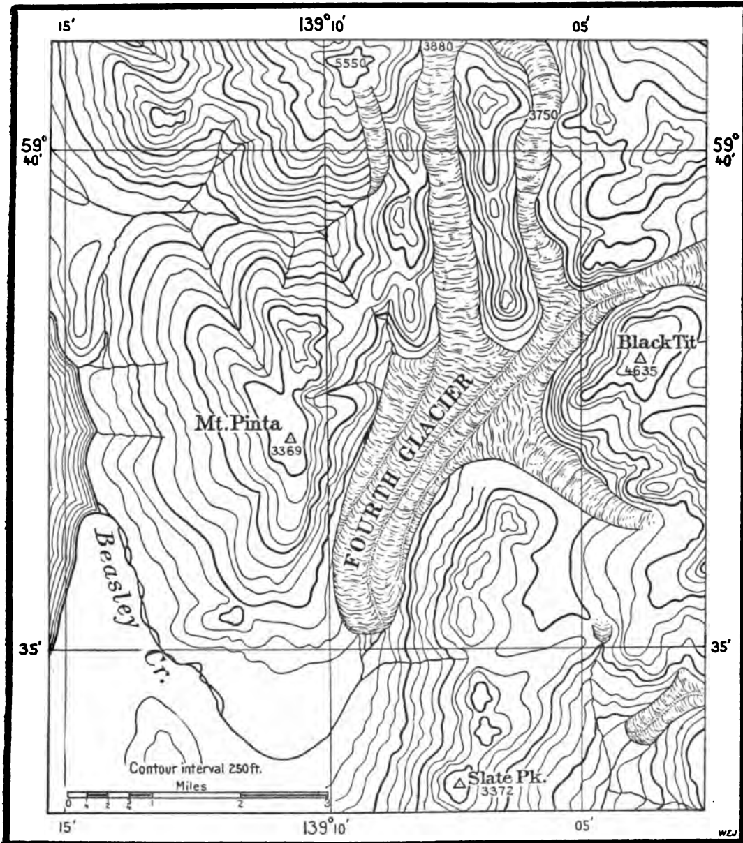
FIG. 15. FOURTH GLACIER IN 1906, BY CANADIAN BOUNDARY SURVEY.
