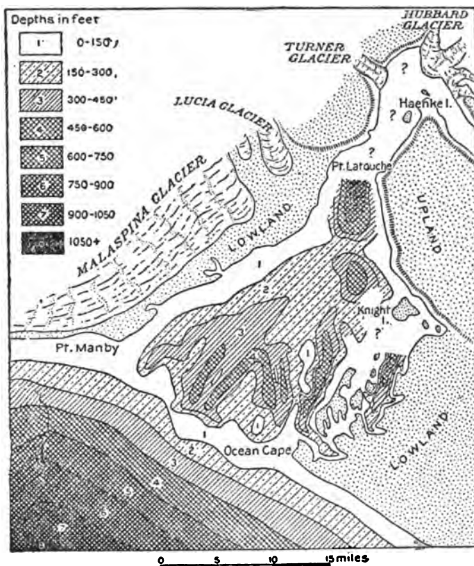
FIG. 21. YAKUTAT BAY, SHOWING CONTOURS OF DEPTH AND SUBMARINE MORAINE BETWEEN OCEAN CAPE AND POINT MANBY (AFTER G. K. GILBERT).
