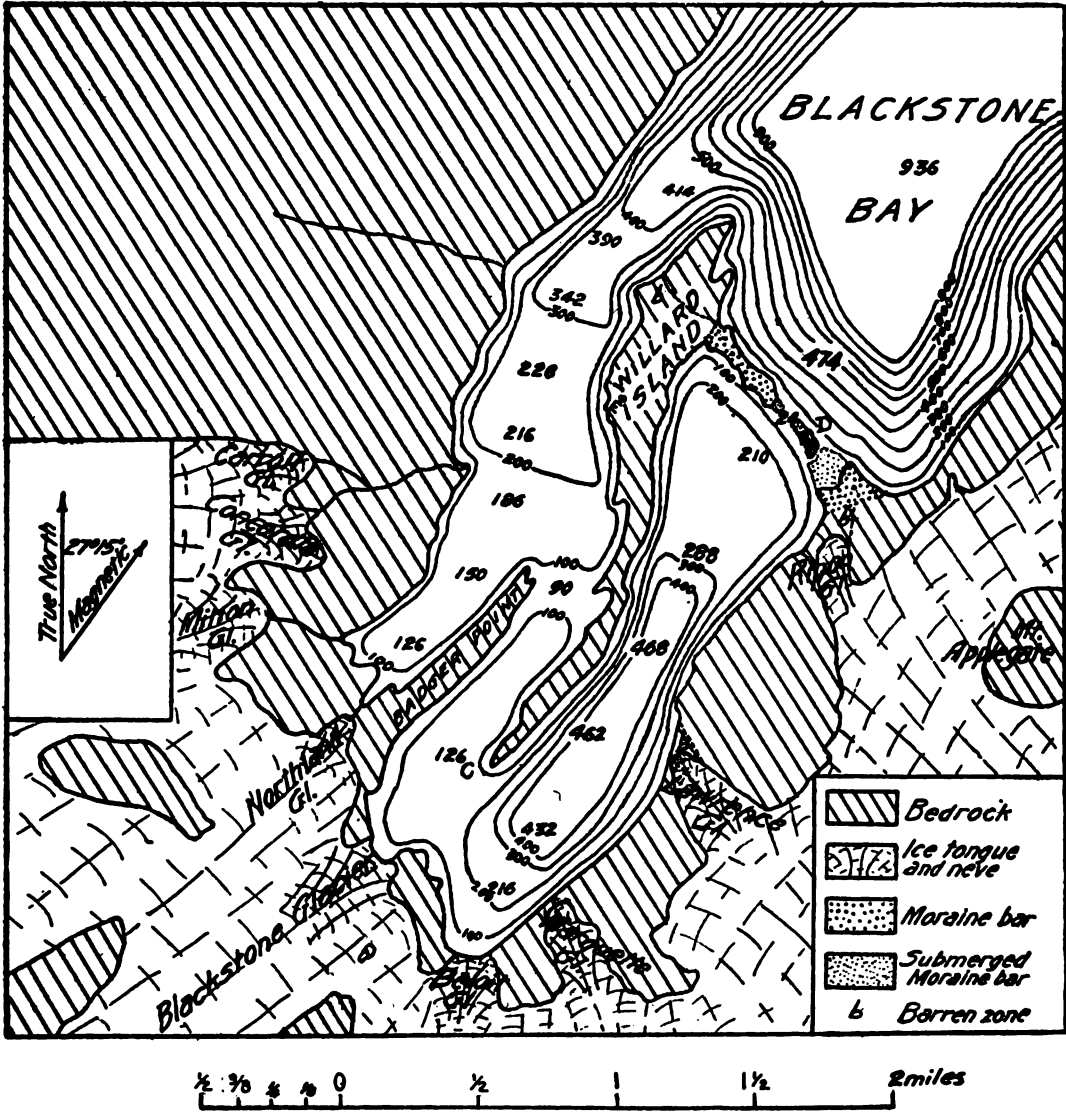
FIG. 58. GLACIERS AND SUBMARINE CONTOURS OF BLACKSTONE BAY. Soundings in feet. Photographic stations shown by letters C, D, and E.
