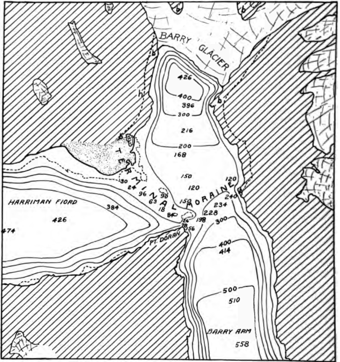
BARRY GLACIER Showing crescentic submarine terminal moraine.
