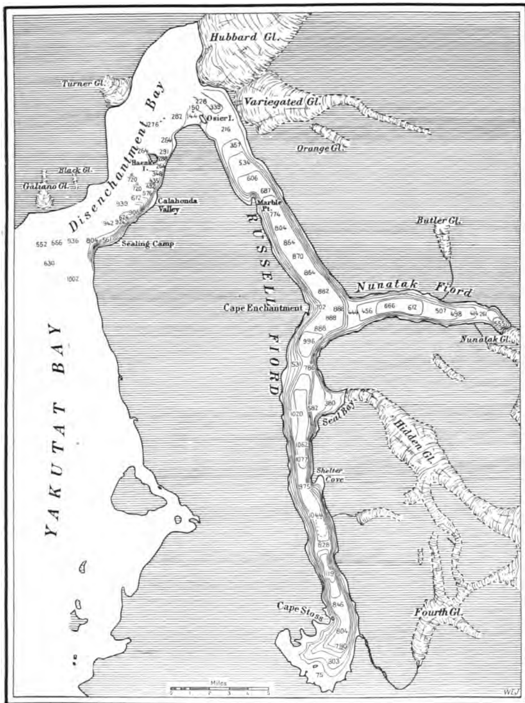
SOUNDINGS AND SUBMERGED CONTOURS IN RUSSELL FIORDE AND DISENCHANTMENT BAY
