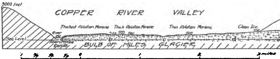
FIG. 63. NATURAL SCALE CROSS-SECTION OF COPPER RIVER VALLEY.
