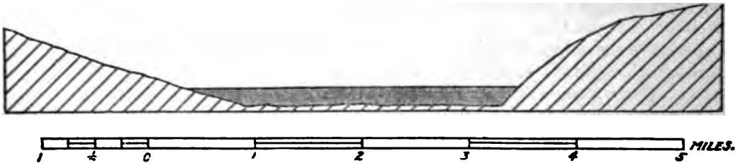
FIG. 27. NATURAL SCALE CROSS-SECTION OF PORT VALDEZ.
