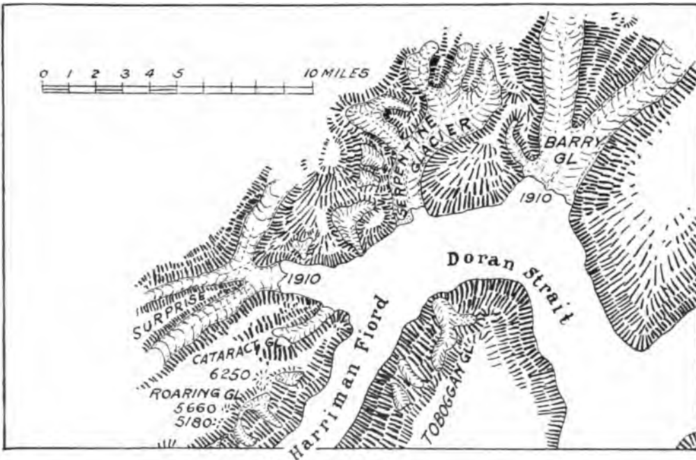
B. HARRIMAN FIORD IN 1910 Showing the retreat of Barry and Surprise Glaciers since 1899.
