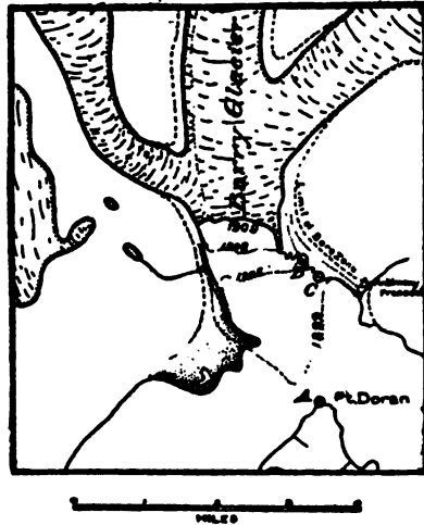
FIG. 44. FRONT OF BARRY GLACIER. Showing recession from 1899 to 1909 (After Grant and Higgins).
