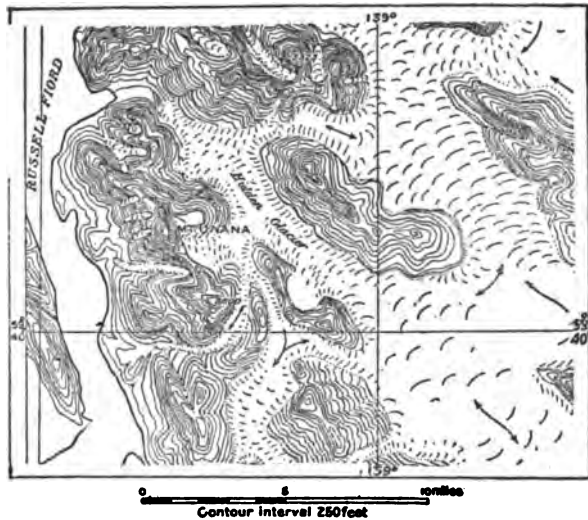
FIG. 12. THE WHOLE OF HIDDEN GLACIER. FRONT SHOWN AS MAPPED BY CANADIAN BOUNDARY SURVEY IN 1895.
