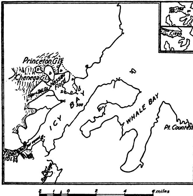
FIG. 56. THE GLACIERS OF ICY BAY IN 1794, 1898, AND 1908.
