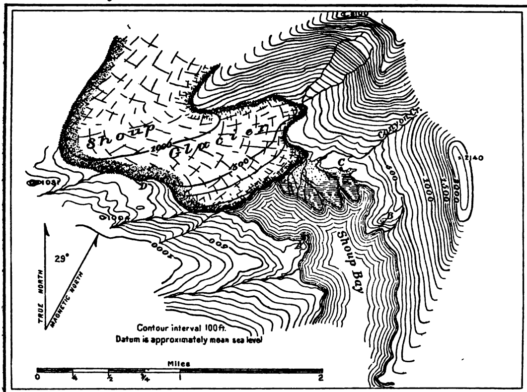
FIG. 24. SKETCH MAP OF SHOUP GLACIER IN 1909.
