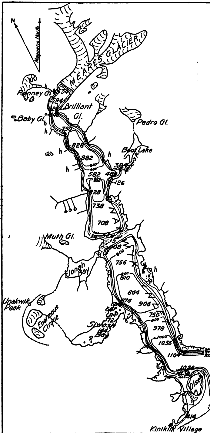
FIG. 38. SUBMARINE CONTOURS IN UNAKWIK INLET. Outline of coast and glaciers after Grant and Higgins.
