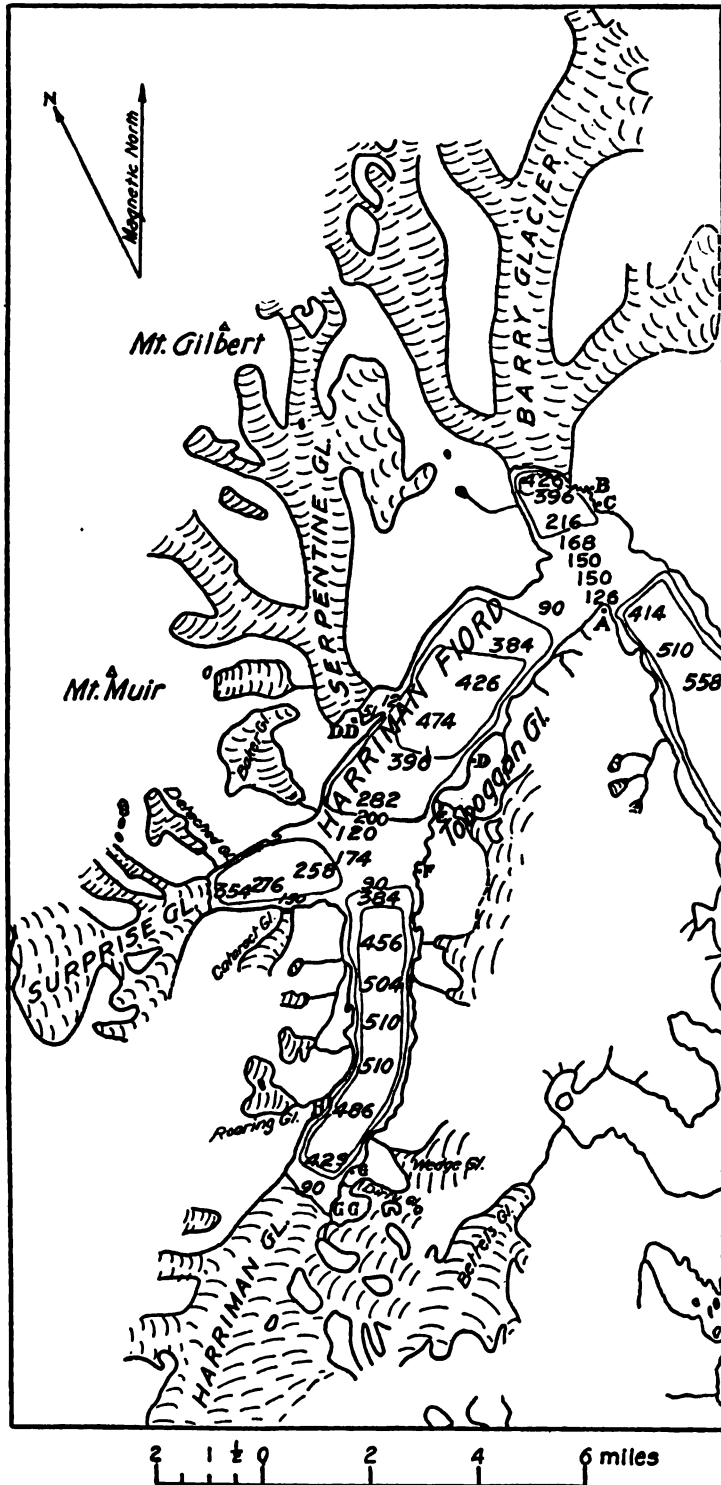
FIG. 50. SUBMARINE TOPOGRAPHY OF HARRIMAN FIORD.
