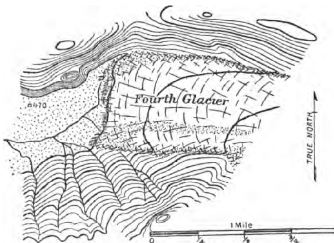
FIG. 16. SKETCH MAP OF FOURTH GLACIER IN 1909.
