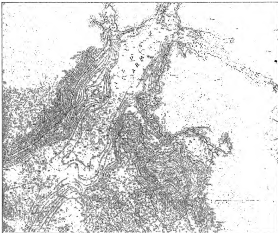
FIG. 28. SUBMARINE CONTOURS OF VALDEZ ARM.
