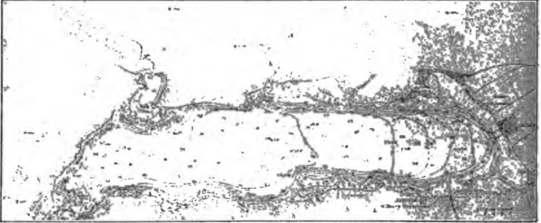
FIG. 26. SUBMARINE CONTOURS OF PORT VALDEZ.
