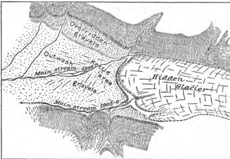
FIG. 15. HIDDEN GLACIER IN 1905, SHOWING FOSSE BETWEEN THE GLACIER AND THE WORDS Kettle area .
