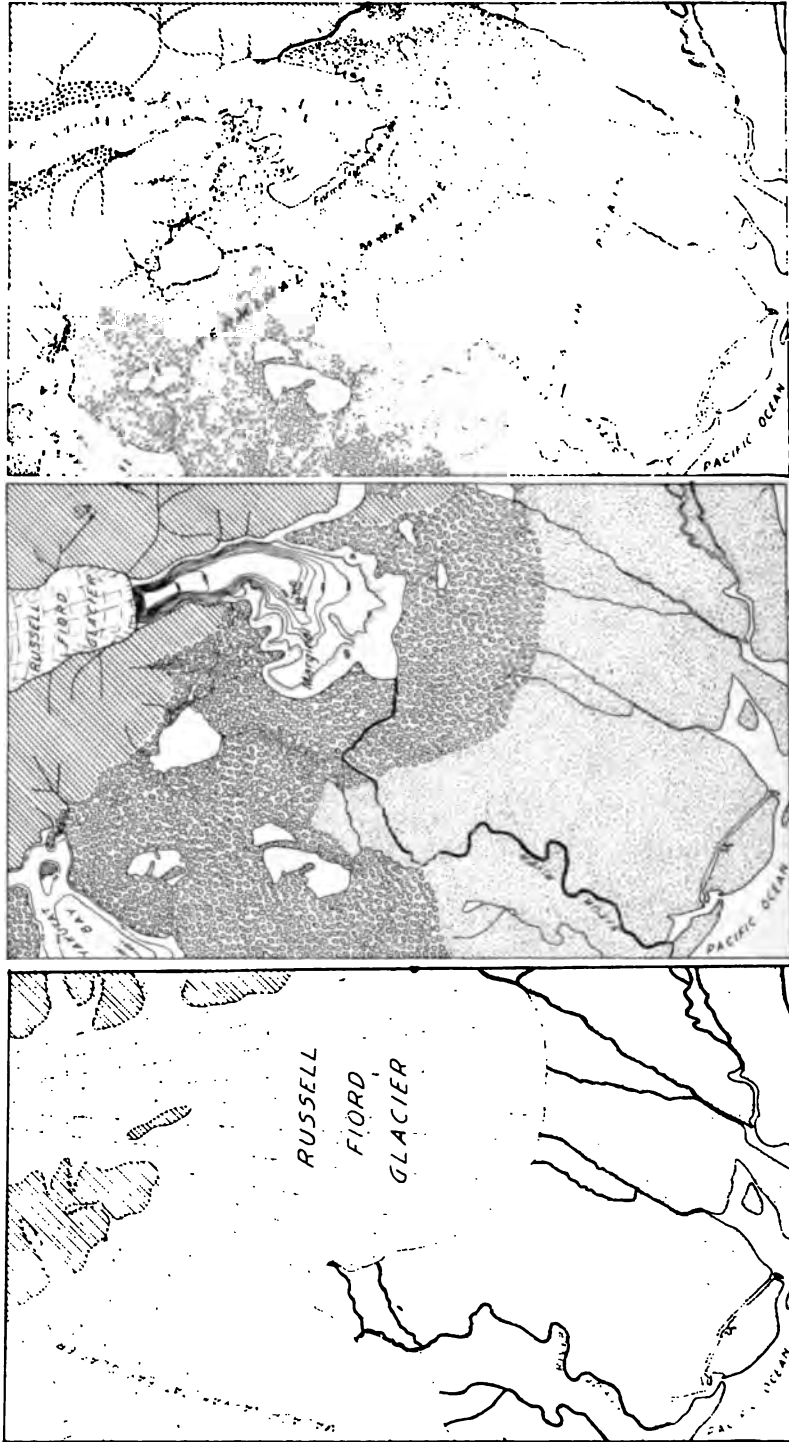
THREE MAPS SHOWING SOUTH END OF RUSSELL FIORD
