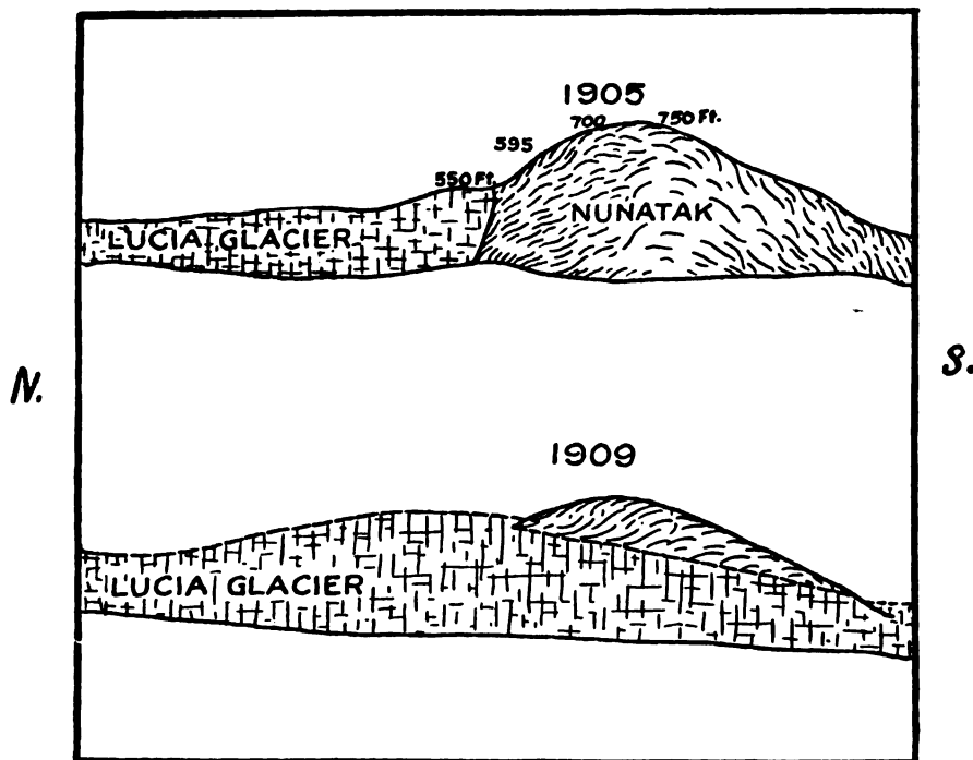
FIG. 4. LONGITUDINAL SECTIONS OF LUCIA GLACIER AND NUNATAK.
