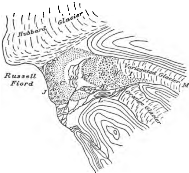
FIG. 7. Sketch map of banded moraines of Variegated Glacier in 1905. A, White granite moraine; B, red rusted moraine; C, hornblende gneiss moraine; D, interior flat; E, red moraine; F, purple moraine; G, green moraine; H, orange moraine; I, ice surface; J, beach; K, glacial stream, 1905; L, glacial stream, 1906; M, highest point reached in 1905.
