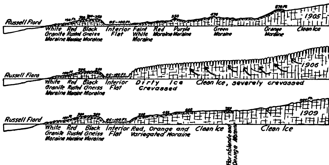
FIG. 8. LONGITUDINAL SECTIONS OF VARIEGATED GLACIER.
