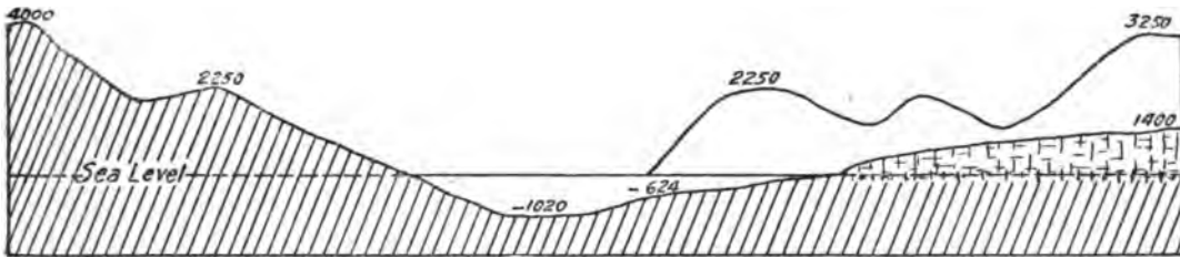
FIG. 17. SECTION OF SEAL BAY AND HIDDEN GLACIER WITH ITS SUBMERGED HANGING VALLEY. CROSS-SECTION OF RUSSELL FIORD. VERTICAL AND HORIZONTAL SCALES THE SAME.
