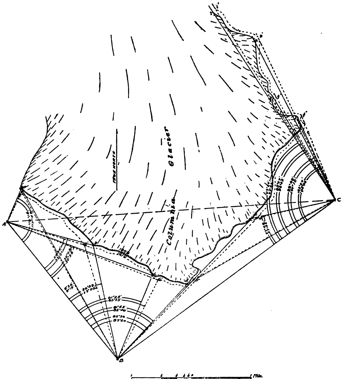
FIG. 30. TRIANGULATION ON FRONT OF COLUMBIA GLACIER SHOWING ADVANCE FROM 1909 TO 1910.
