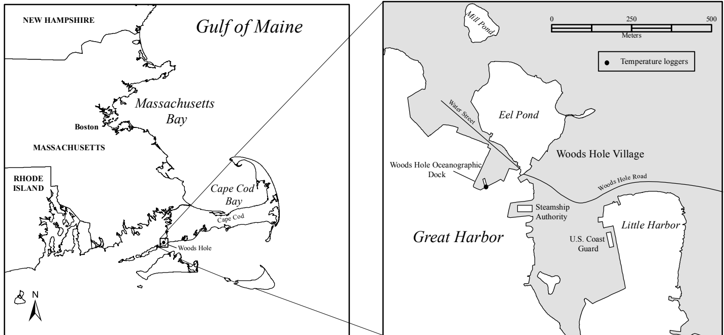
Figure 2. Maps showing Great Harbor and the location of temperature loggers hung at 2 m, 5 m, and 10 m from the dock of the Woods Hole Oceanographic Institution in Woods Hole, MA.
