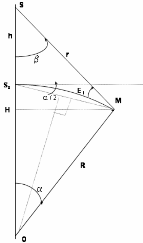
FIGURE A3-2 Satellite GS geometry in two dimensions
