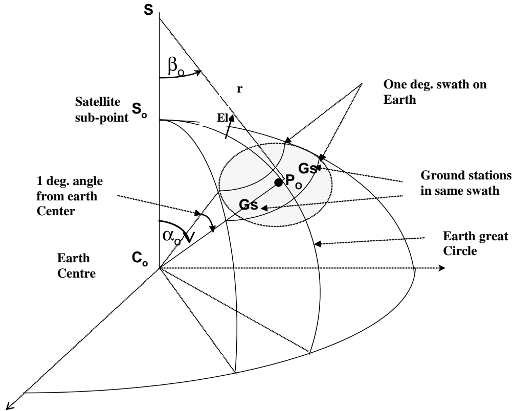
FIGURE A3-1 Earth, satellite and ground stations geometrical configuration
