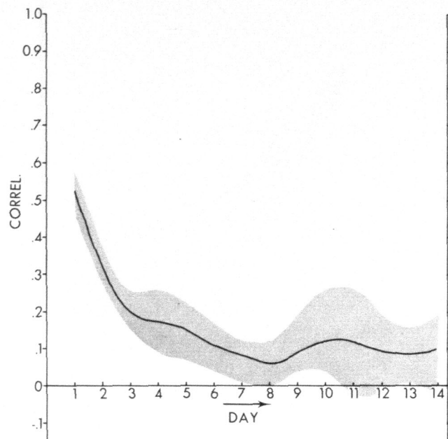
FIGURE 15.—The correlation coefficients for the Laplacian of 500-mb height anomalies, \nabla^2(z-z_n) .
