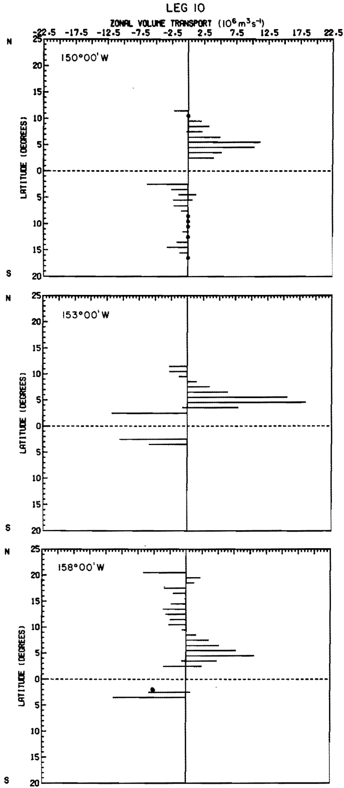
Figure 73.--Distribution of eastward (positive) and westward (negative) volume transport relative to 1000 db at 158°00', 153°00' and 150°00'W on Leg 10. Refer to individual sections for dates. Circles indicate zero transport.
