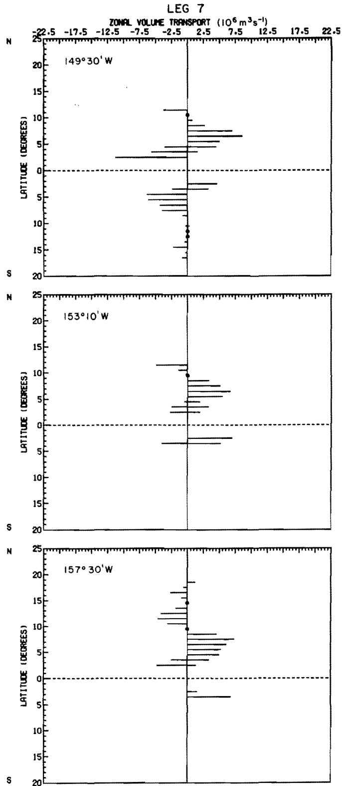
Figure 70.--Distributions of eastward (positive) and westward (negative) volume transport relative to 1000 db at 157°30', 153°10', and 149°30'W on Leg 7. Refer to individual sections for dates. Circles indicate zero transport.
