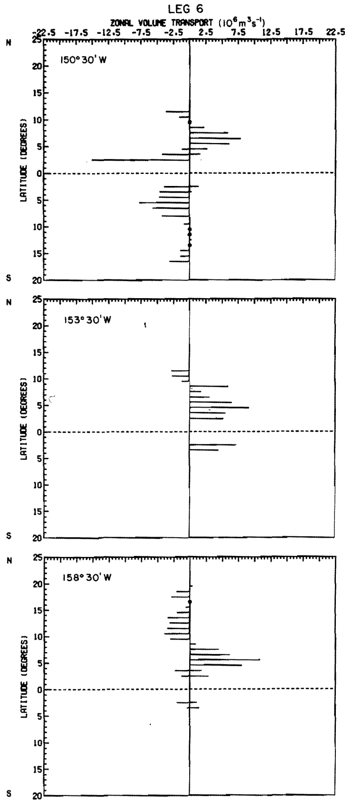
Figure 69. --Distributions of eastward (positive) and westward (negative) volume transport relative to 1000 db at 158°30', 153°30' and 150°30'W on Leg 6. Refer to individual sections for dates. Circles indicate zero transport.
