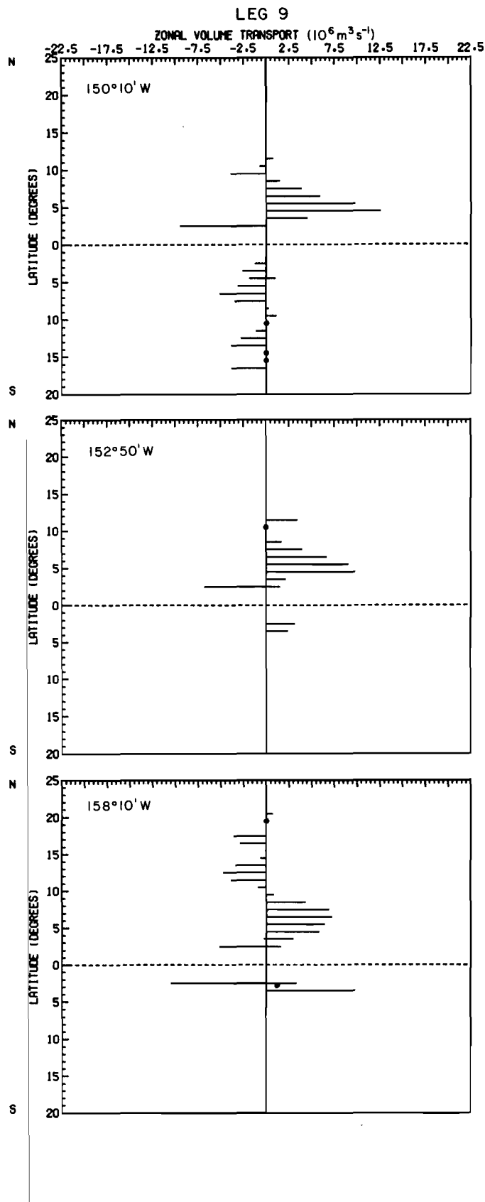
Figure 72.--Distributions of eastward (positive) and westward (negative) volume transport relative to 1000 db at 158°10', 152°50' and 150°10'W on Leg 9. Refer to individual sections for dates. Circles indicate zero transport.
