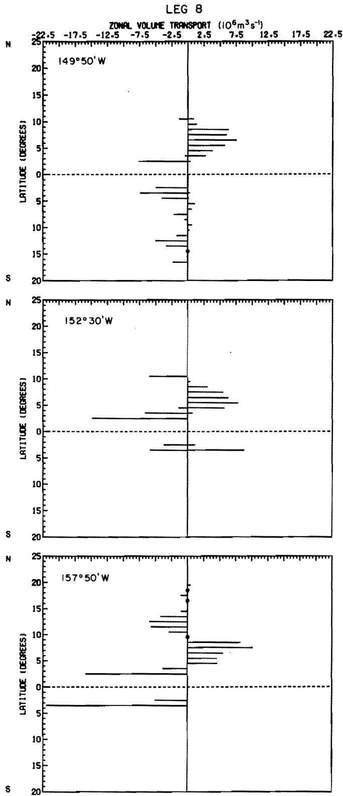
Figure 71.--Distributions of eastward (positive) and westward (negative) volume transport relative to 1000 db at 157°50', 152°30' and 149°50'W on Leg 8. Refer to individual sections for dates. Circles indicate zero transport.
