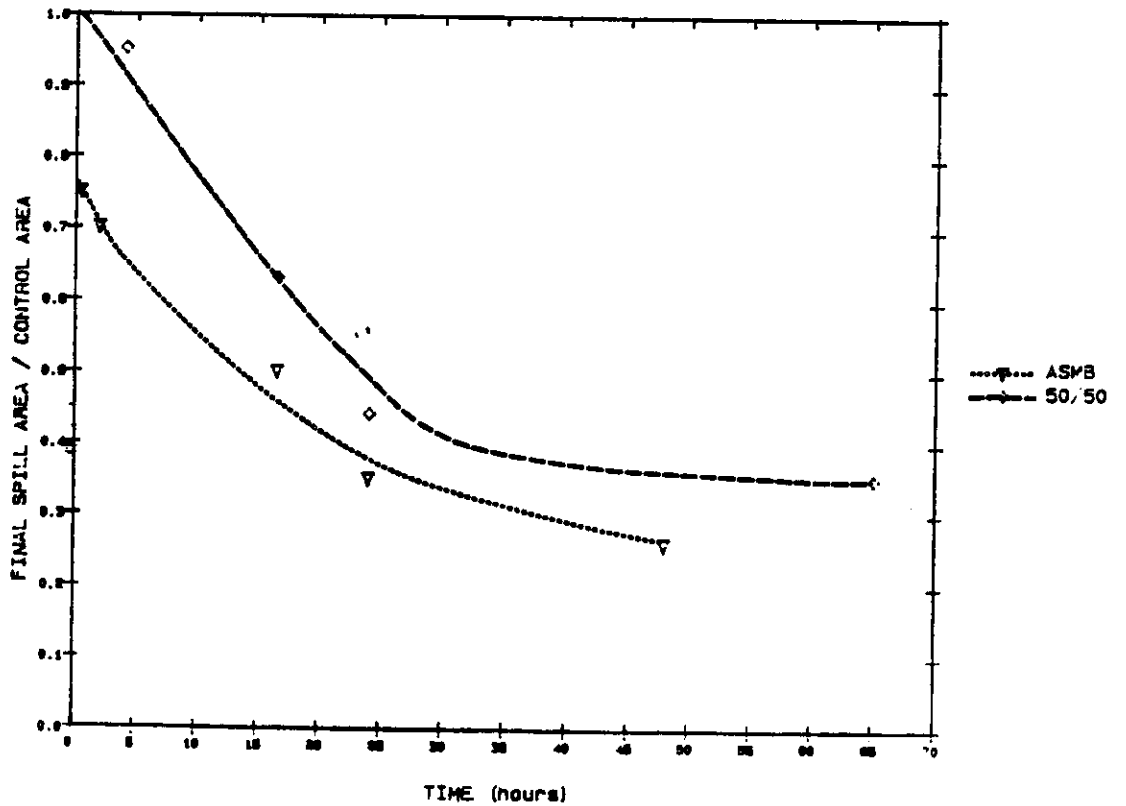
Figure 2-20. The extent of spreading versus reaction time for ASMB and the Emulsifying Mix with 6000 ppm of Elastol at 15 deg. C.
