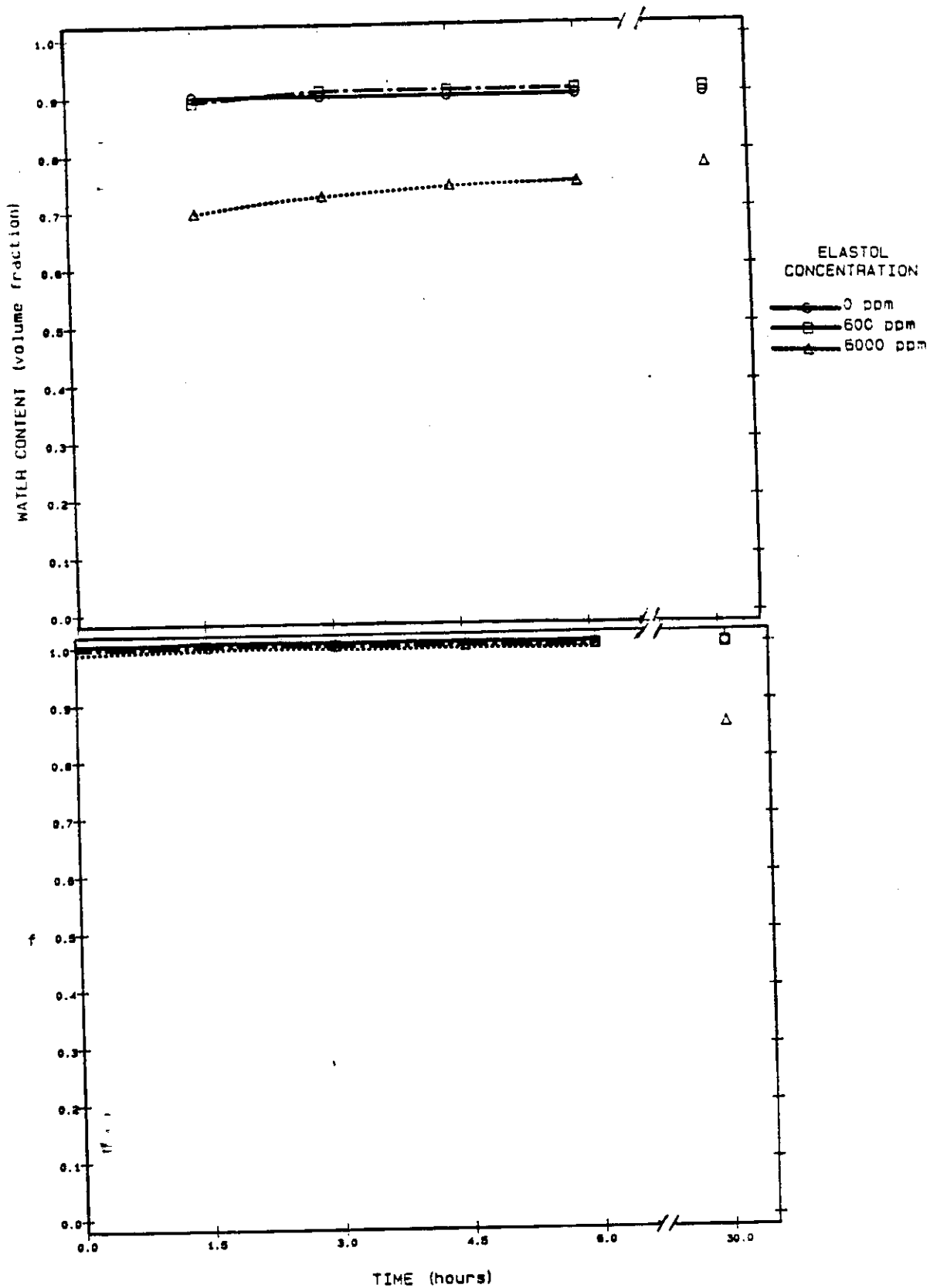
Figure 2-22. Plots of f and water content versus time for ASMB 15% weathered at 15 deg. C.
