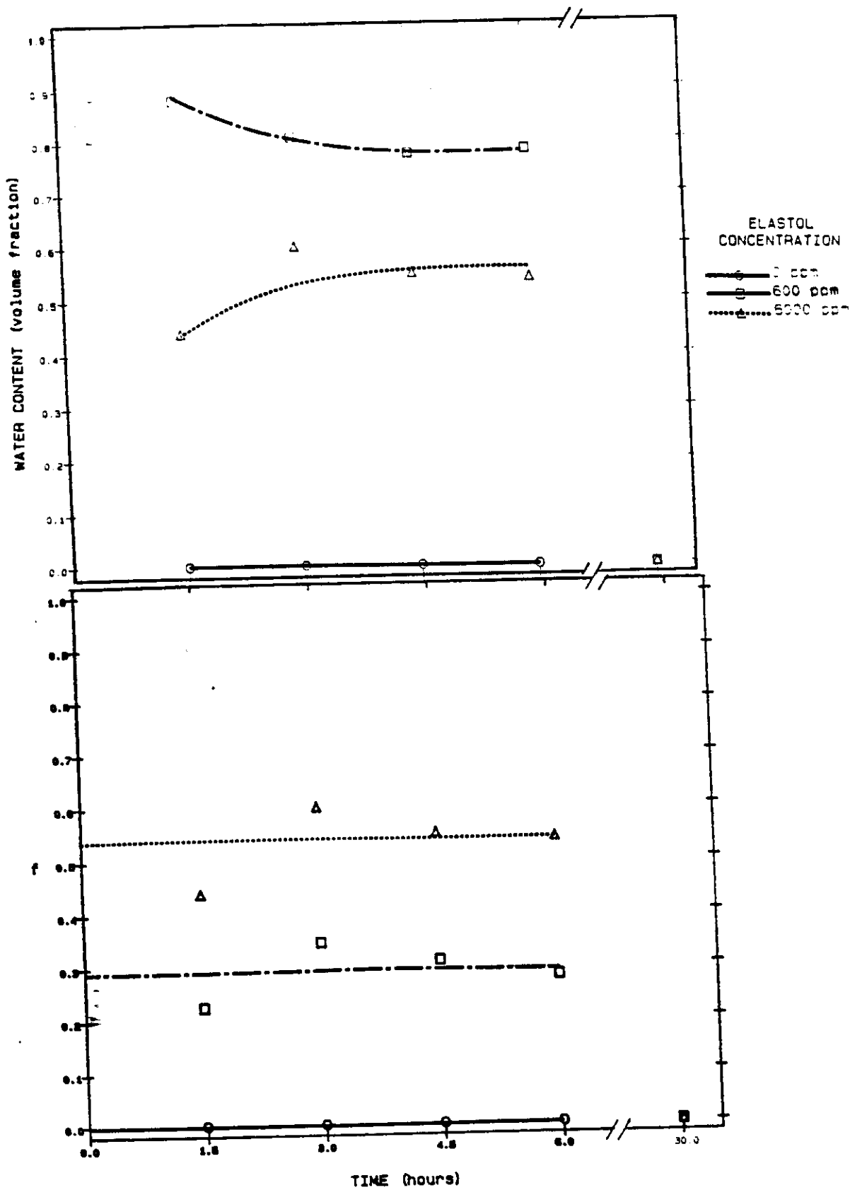
Figure 2-26. Plots of f and water content versus time for Amalgak at 15 deg. C.
