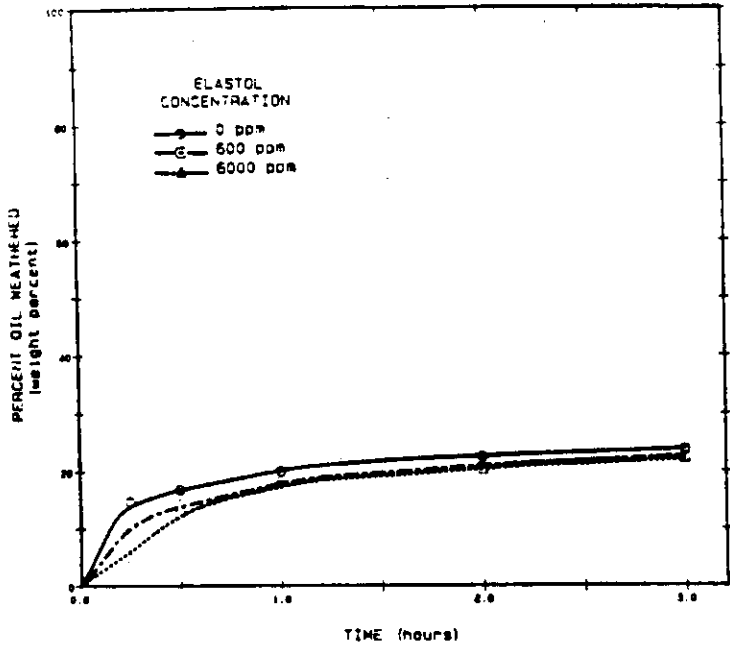
a) ASMB: 15 Deg. C, 150 r.p.m., Salt water.
