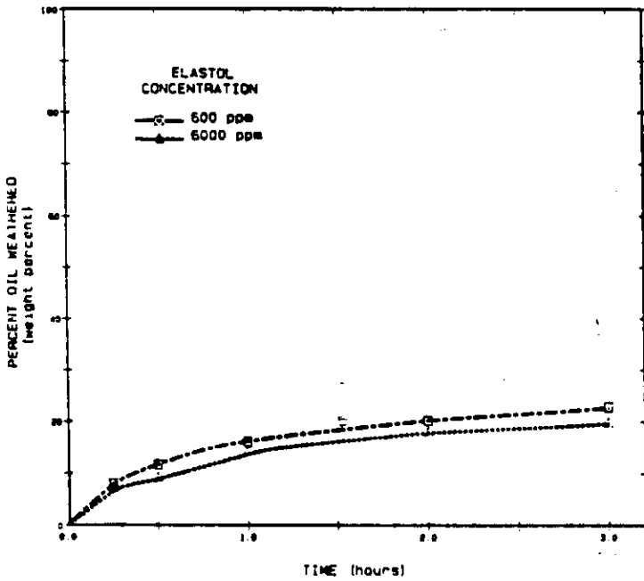
c) ASMB: 15 Deg. C, 150 r.p.m., Fresh water.
