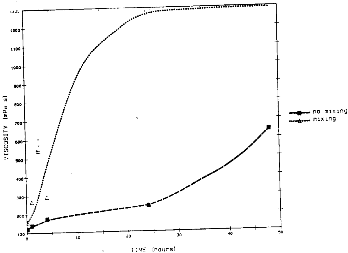
Figure 2-14. Effect of mixing on the viscoelastic properties of Emulsifying Mix with 6000 ppm of Elastol at 15 deg. C.
