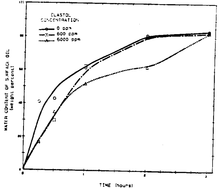
b) Emulsification versus time.
