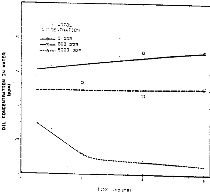
a) Dispersion versus time.
