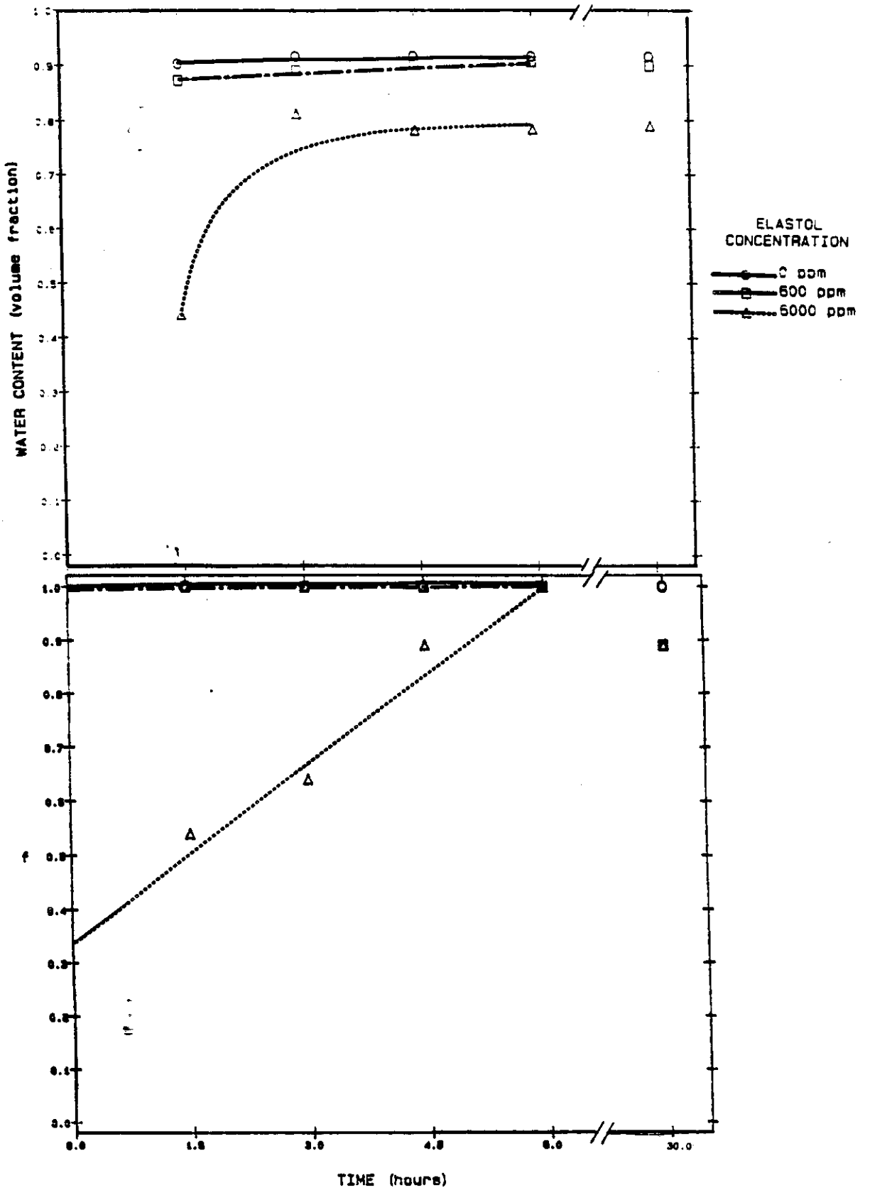
Figure 2-35. Plots of f and water content versus time for Prudhoe Bay at 0 deg. C.
