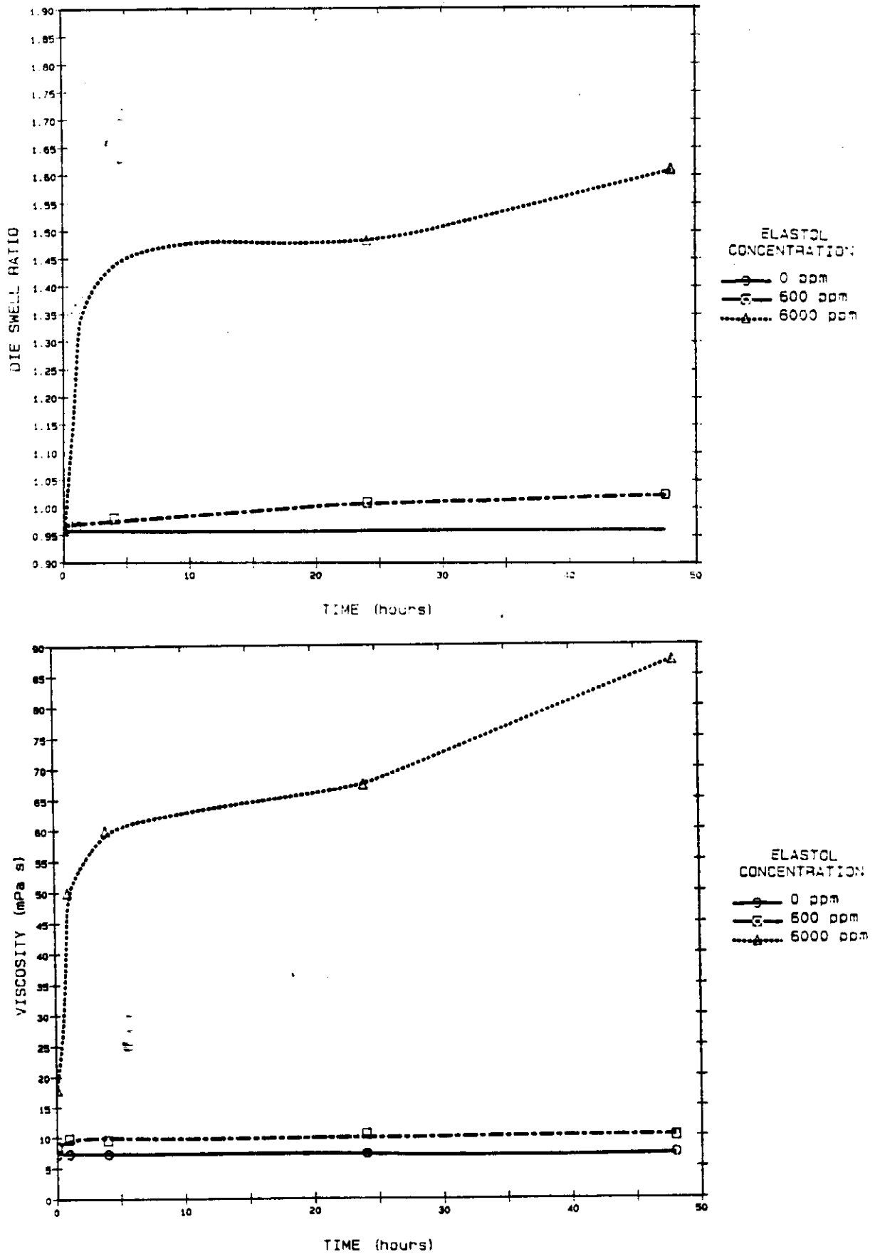
Figure 2-10. Die swell ratio and viscosity versus time for Tarsiut at 15 deg. C.
