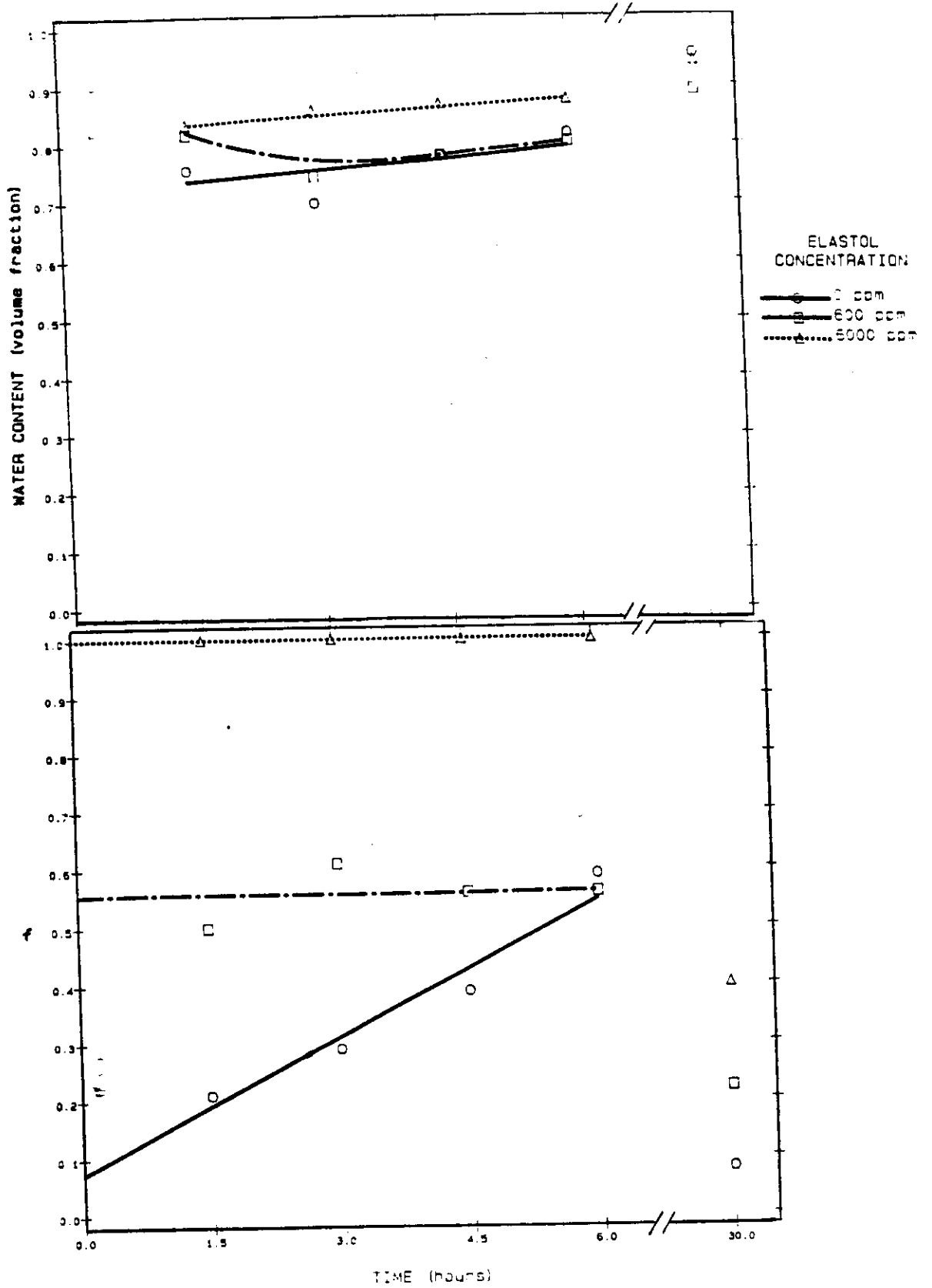
Figure 2-28. Plots of f and water content versus time for Tarsiut at 15 deg. C.
