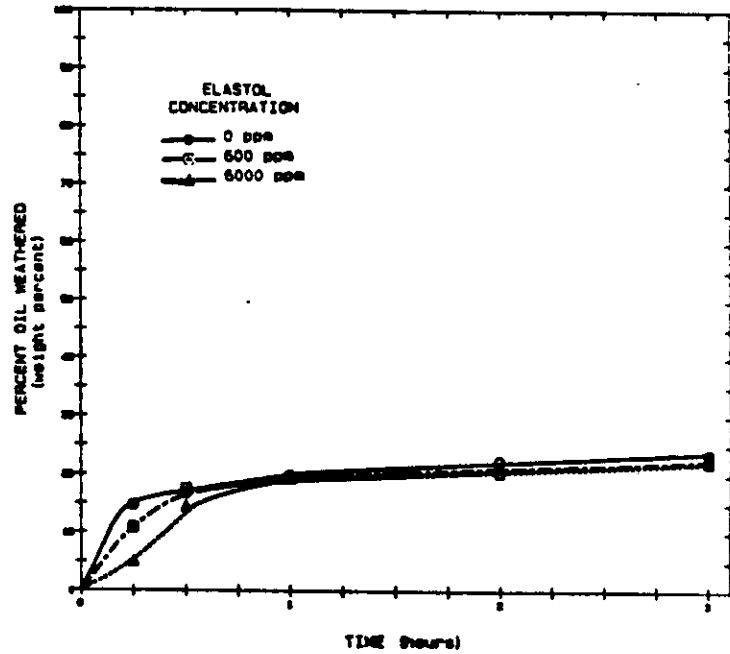
d) ASMB: 15 Deg. C, 220 r.p.m., Salt water.
