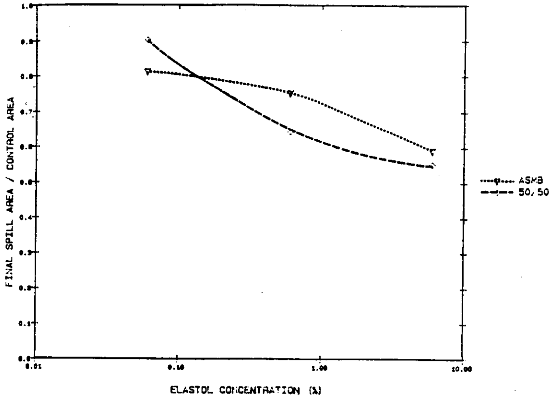
Figure 2-19. The extent of spreading versus concentration of Elastol for ASMB and the Emulsifying Mix at 15 deg. C.
