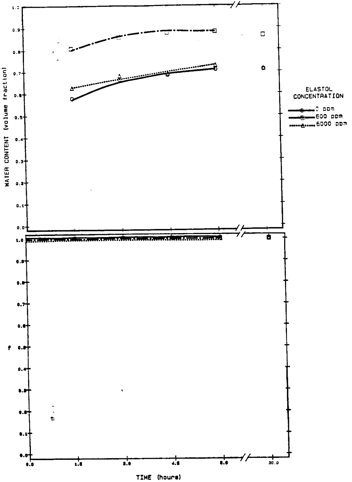
Figure 2-33. Plots of f and water content versus time for Hybernia at 0 deg. C.
