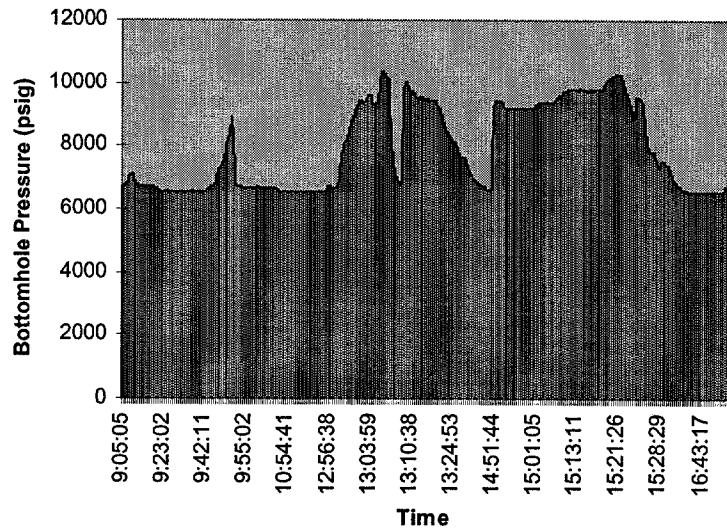
Figure 4.2: Typical Ship Shoal Frac Pack Treatment
