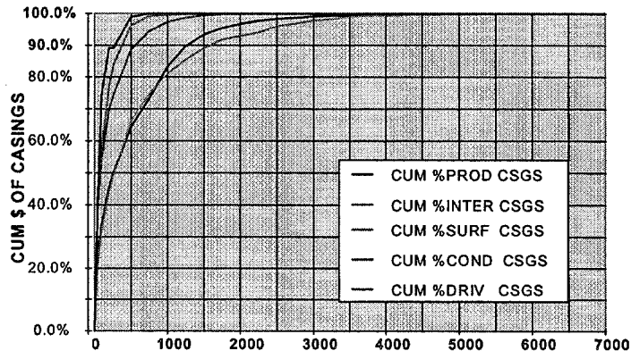
Figure 3.5: Pressure Distribution by Occurrence in Each Casing.
