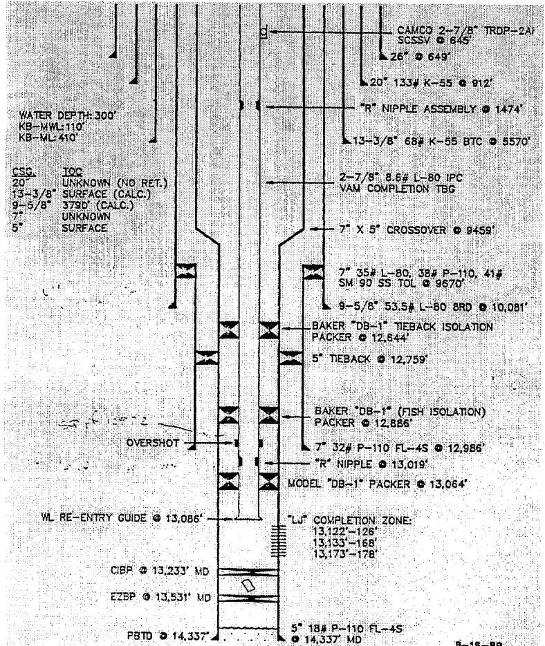
Figure 7.3: Wellbore Schematic for Case History 1.
