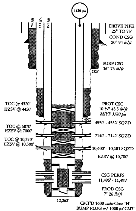
Figure 7.1 - Example 1 of Unsuccessful Workover for SCP
