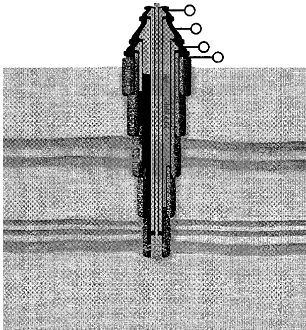
Figure 2.1 - Simplified Well Schematic.
