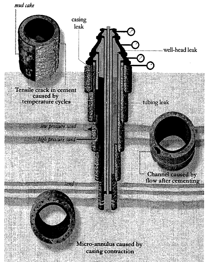
Figure 4.1: Origins of Sustained Casing Pressure
