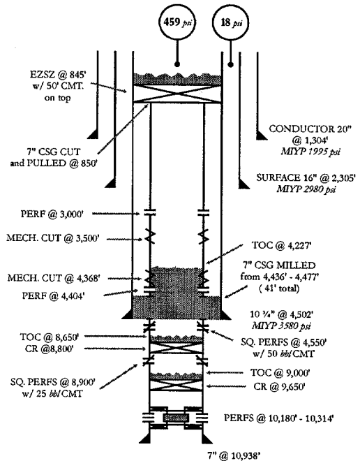
Figure 7.2 - Example 2 of Unsuccessful Workover for SCP
