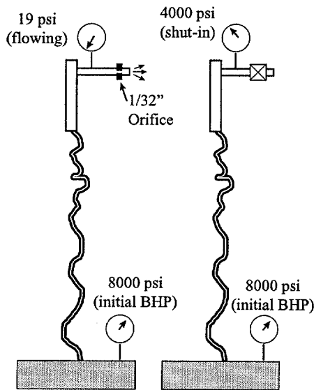
Figure 7.6: Flow Behavior for Case History 1
