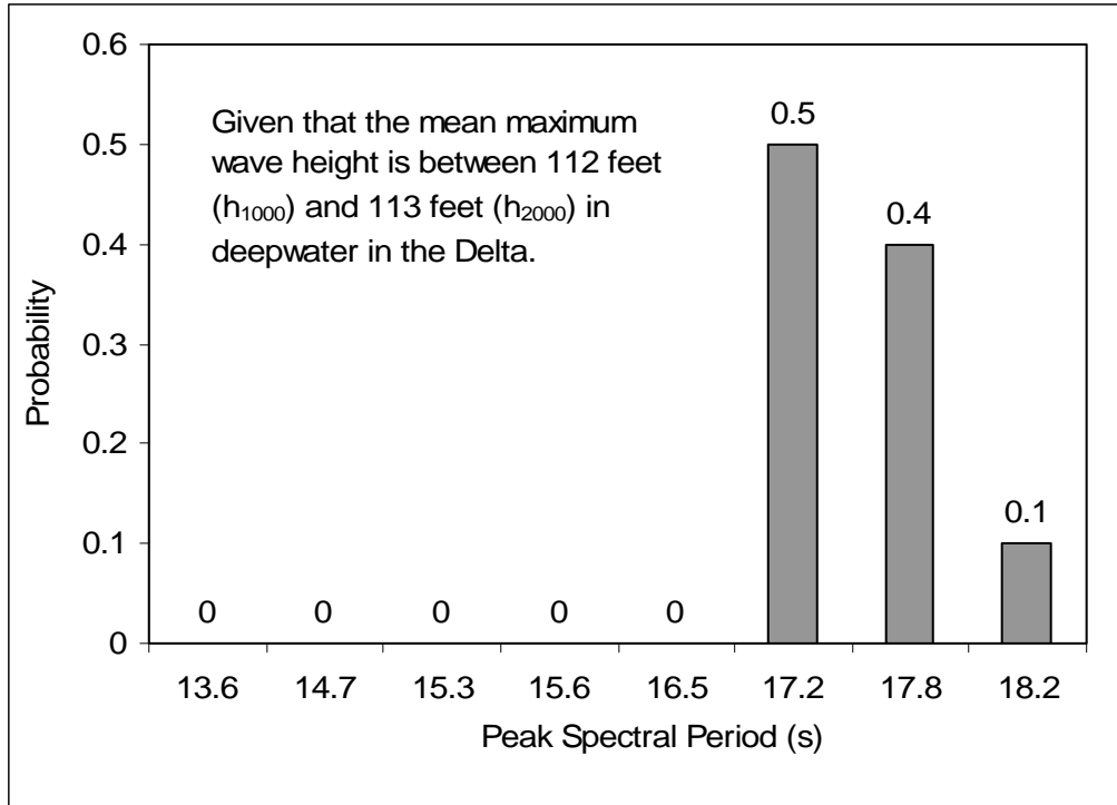
Figure 10. Conditional probability distribution for peak spectral period given that the mean maximum wave height is between 112 and 113 feet in deepwater in the Delta (or between the 1000-year and 2000-year return period values for any water depth in the Delta)
