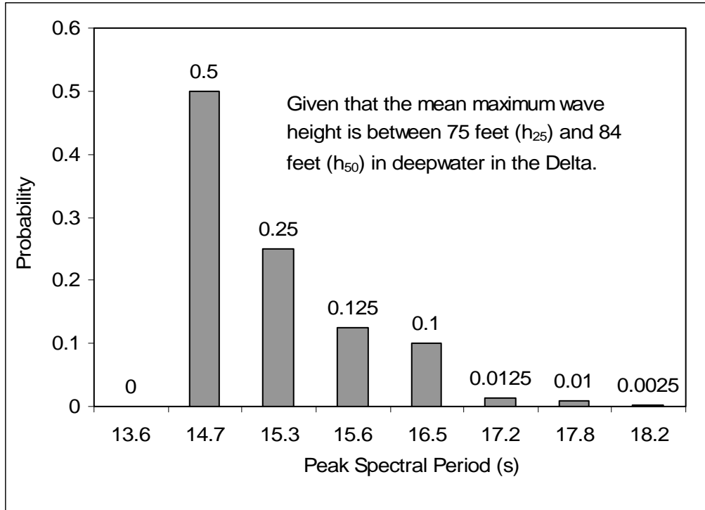
Figure 6. Conditional probability distribution for peak spectral period given that the mean maximum wave height is between 75 and 84 feet in deepwater in the Delta (or between the 25-year and 50-year return period values for any water depth in the Delta)
