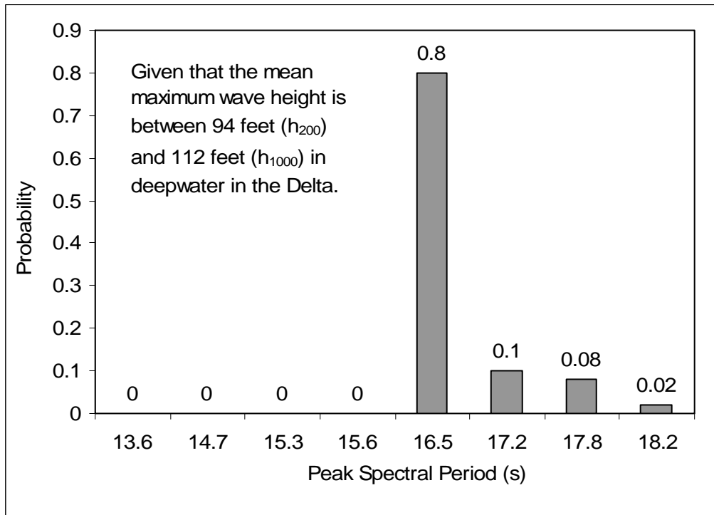
Figure 9. Conditional probability distribution for peak spectral period given that the mean maximum wave height is between 94 and 112 feet in deepwater in the Delta (or between the 200-year and 1000-year return period values for any water depth in the Delta)
