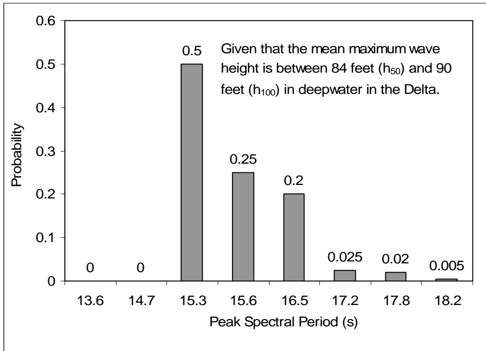
Figure 7. Conditional probability distribution for peak spectral period given that the mean maximum wave height is between 84 and 90 feet in deepwater in the Delta (or between the 50-year and 100-year return period values for any water depth in the Delta)
