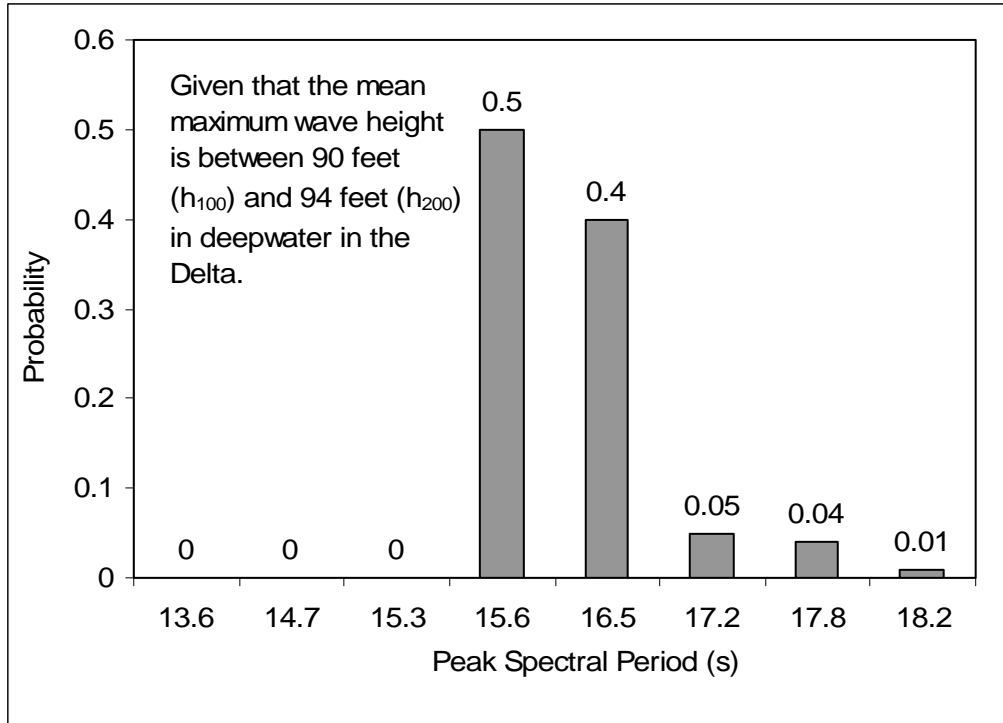
Figure 8. Conditional probability distribution for peak spectral period given that the mean maximum wave height is between 90 and 94 feet in deepwater in the Delta (or between the 100-year and 200-year return period values for any water depth in the Delta)
