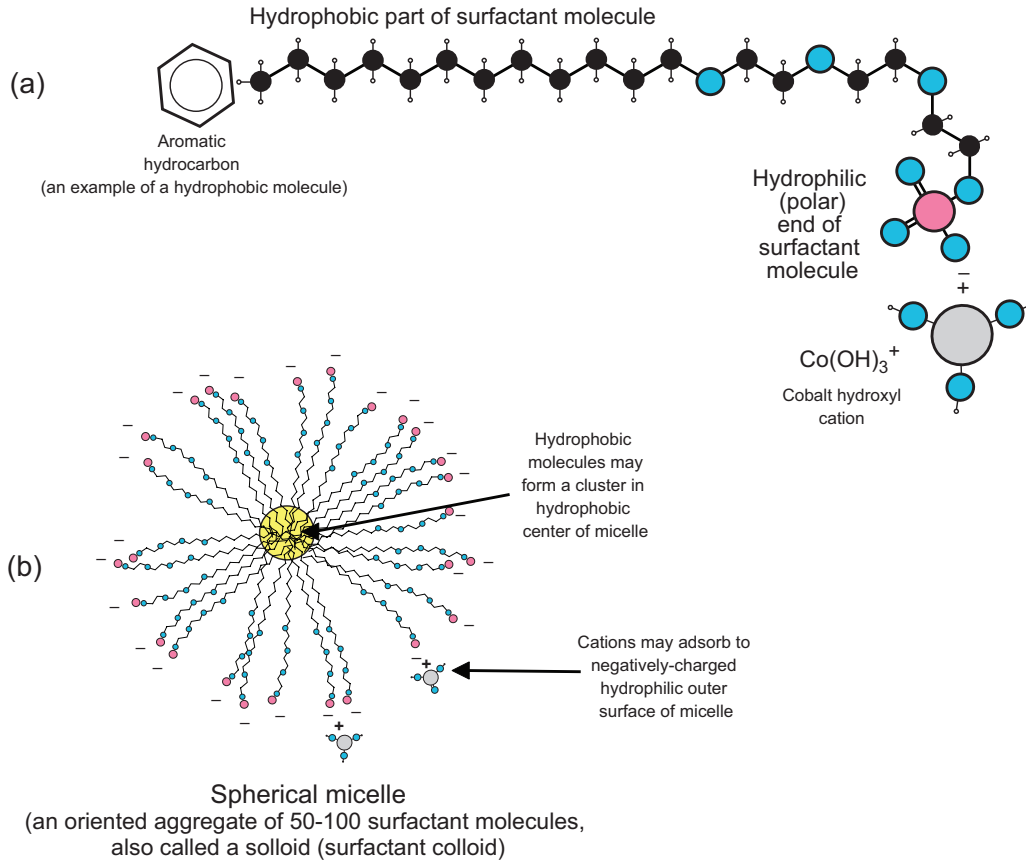
Figure 4-12. Schematics of potential interactions between anionic surfactants and constituents in groundwater: (a) interactions with hydrophobic and hydrophilic ends of a surfactant molecule, and (b) interactions with a surfactant micelle
