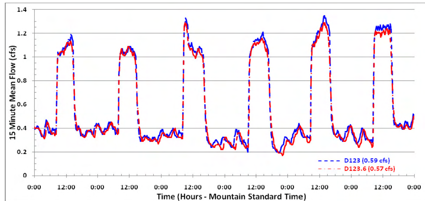
Figure C-1.0-2 Hydrographs from gaging stations D123 and D123.6 from April 21 to April 23, 2008, with time of D123.6 hydrograph shifted by 1.5 hr to better show relationship with D123; average daily discharge at gages shown in parentheses; average discharge from NPDES outfalls = 0.55 cfs for this period
