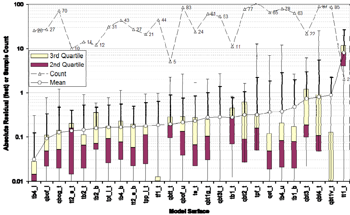
Figure J-2.0-6 Geologic framework model WC08 absolute residual statistics for modeled surfaces as compared to measured elevations
