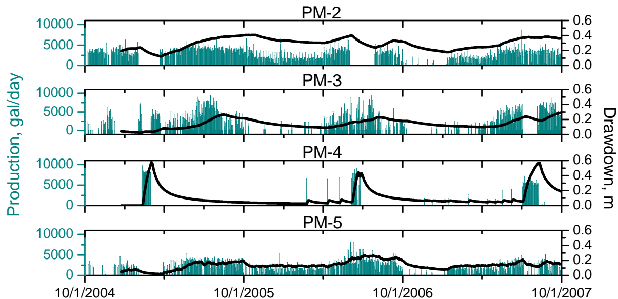
Figure F-4.0-4 Model-predicted drawdown contributions from each water supply well at R-15. The plots also present well production data. Note the different scale of drawdown axes compared to Figures F-4.0-3 and F-4.0-5. The model did not predict that there are transients in the water levels that are not related to the existing pumping; as a result, there is no plot of a trend line.
