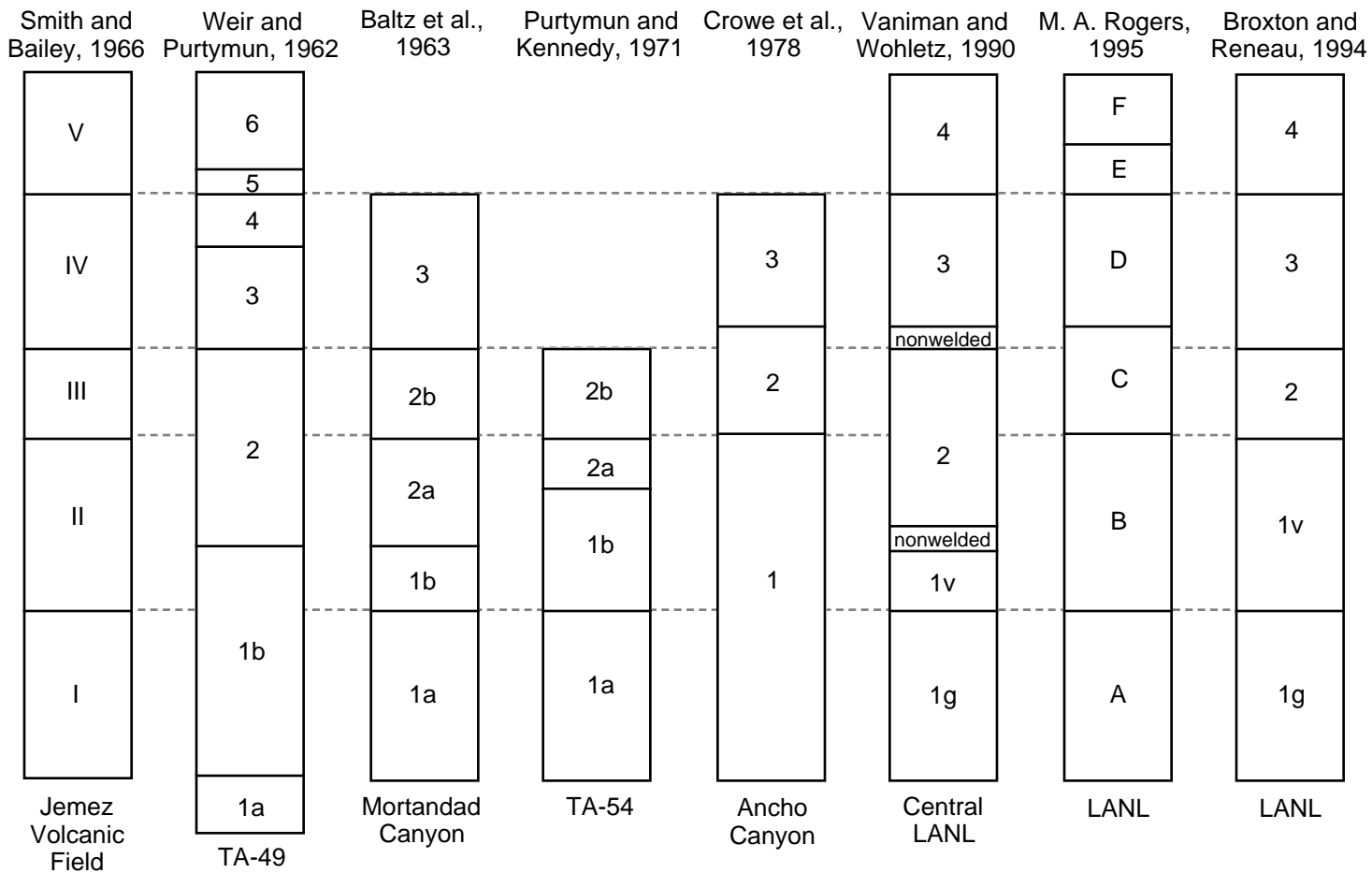
Figure 3. The various correlation schemes suggested for the Tshirege Member of the Bandelier Tuff (after Broxton and Reneau, 1994).
