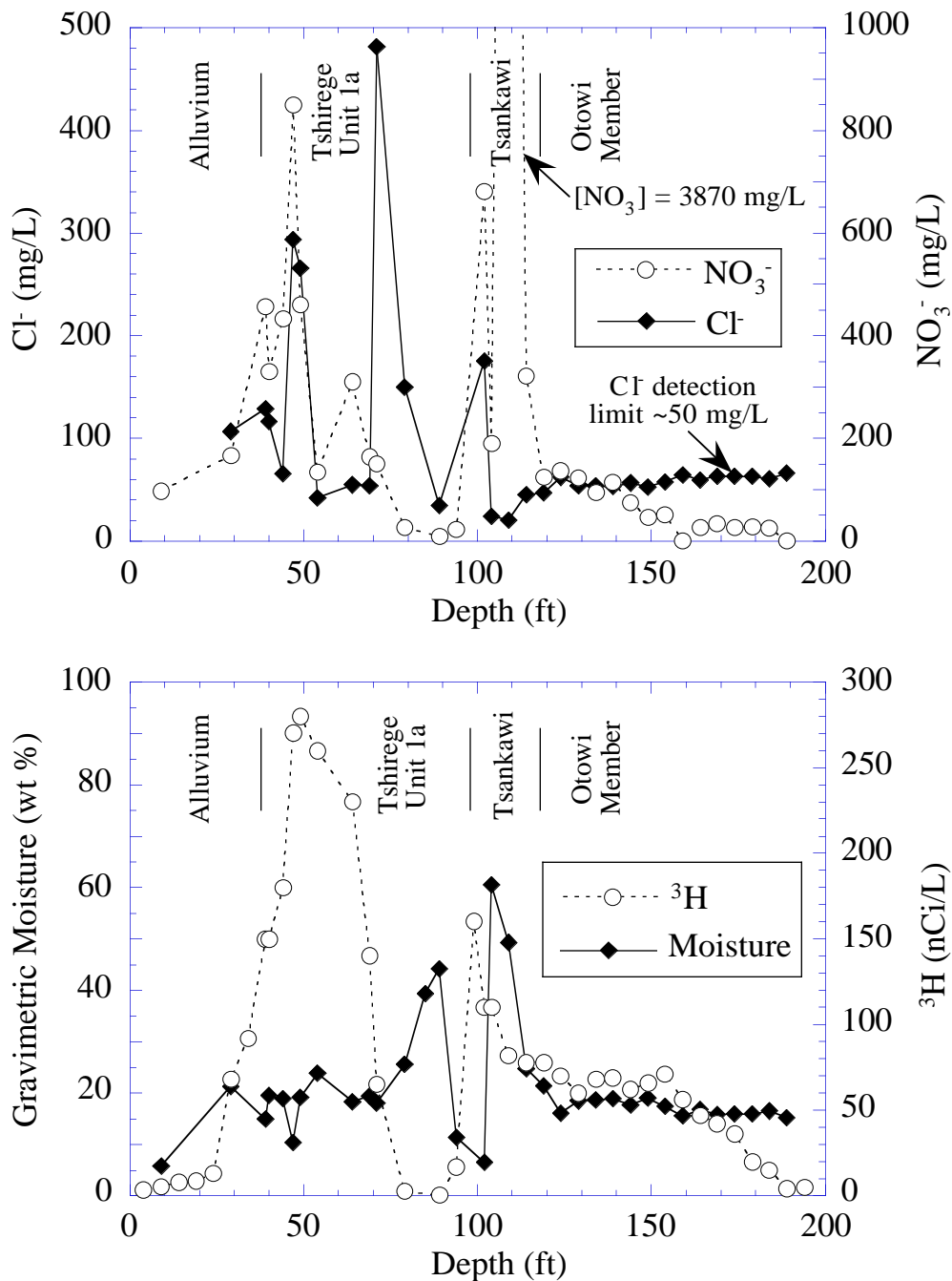
Figure 35. Borehole MCM-5.9A profiles of Cl - and NO 3 - (top) and gravimetric moisture and tritium ( 3 H) (bottom). The data are from Stoker et al. (1991). The Cl - and NO 3 - concentrations were determined as μg/g by leaching core samples with water. The results were converted from μg/g to mg/L using the core gravimetric moisture content. The minimum detection limit for Cl - was 10 μg/g, which converts to about 47–66 mg/L for a gravimetric moisture contents of 15%–21%.
