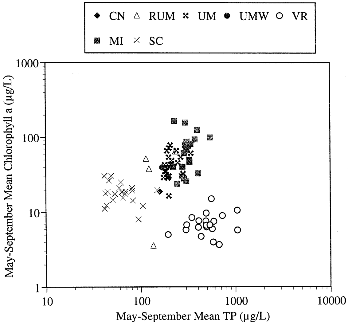
FIGURE 3.26. Mean chlorophyll a concentration for May–September versus mean total P concentration for the same period at sampling sites in the metropolitan Twin Cities area. (Data from C. Larson, Metropolitan Council Environmental Services, St. Paul, MN, 1998.) CN = Cannon River; MI = Minnesota River; RUM = Rum River; SC = St. Croix River; UM = Upper Mississippi River; UMW = Upper Mississippi River, Wisconsin channel (downstream of Hastings, MN); VR = Vermillion River.
