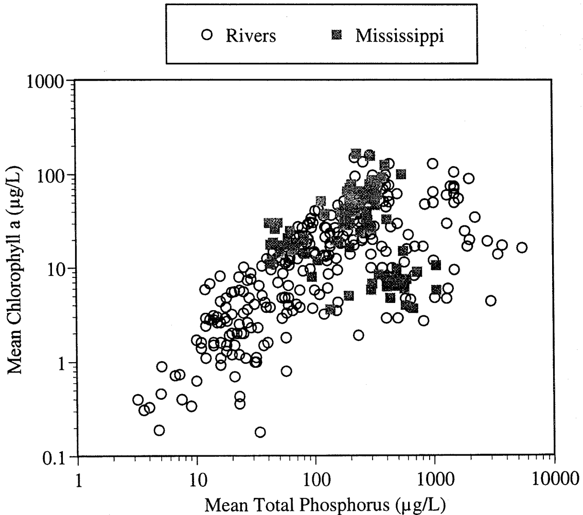
FIGURE 3.29. Growing season mean chlorophyll a concentrations versus corresponding TP concentrations for various rivers. (Data for open circles, from Van Nieuwenhuysse and Jones 1996; data for closed squares, from Metropolitan Council Environmental Services sites in the Twin Cities area.)
