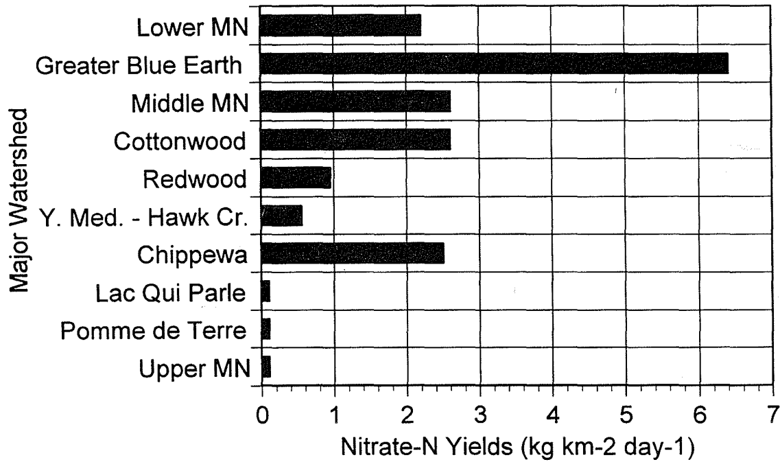
FIGURE 3.8. Nitrate yields (kg km -2 da -1 ) for major watersheds in the Minnesota River Basin. NOTE: The basins are listed from top to bottom in general east to west order of their location in the basin. (From D. Mulla, unpublished, University of Minnesota, 1998.)
