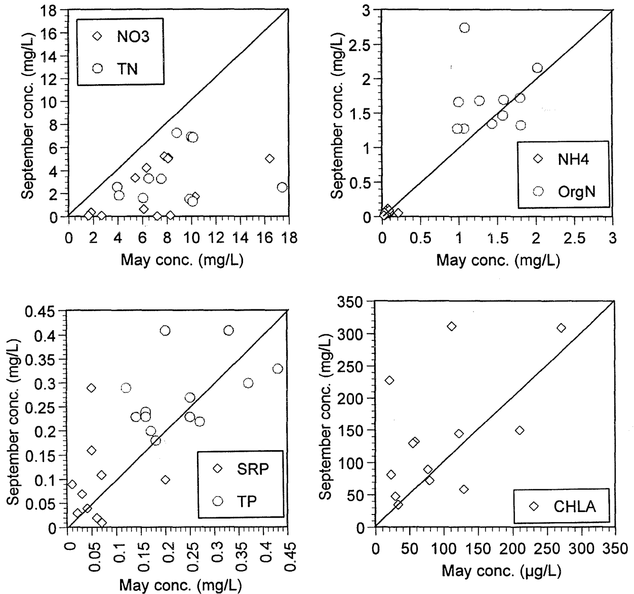
FIGURE 3.16. Plots of late summer (September) concentrations of various nutrient (N and P) forms and chlorophyll a , versus corresponding spring (May) values for the Minnesota River at Jordan, MN. NOTE: Each datum represents the mean monthly values for a given year between 1980 and 1992. Not all years had data for all variables; thus, 13 data points are not present on all graphs. (Data from Metropolitan Council Environmental Services, St. Paul, MN.)
