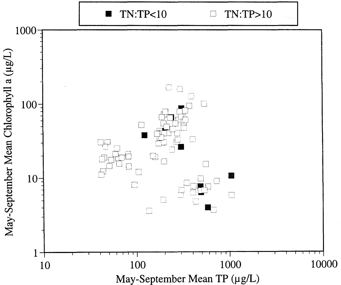
FIGURE 3.27. Replot of Figure 3.26 with data coded according to the ratio TN:TP.
