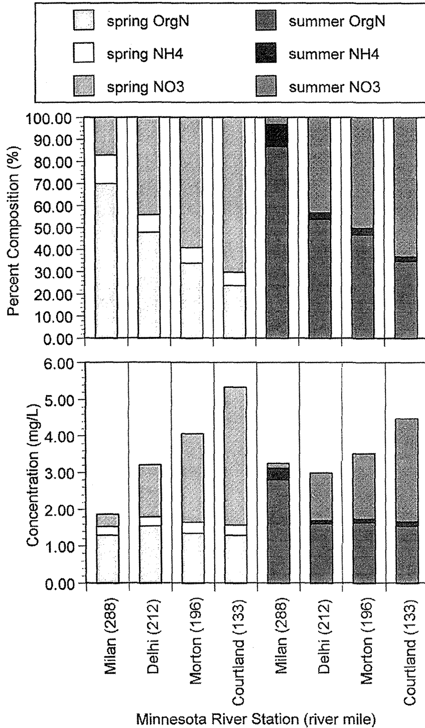
FIGURE 3.19. Percent composition (upper panel) and concentrations (lower panel) of nitrogen forms in spring (four bars to the left) and summer (four bars to the right) for four stations in the Minnesota River. NOTE: Stations are plotted left to right in order of downstream direction. (Data from various agencies and assembled by D. Mulla, University of Minnesota, St. Paul, MN.)
