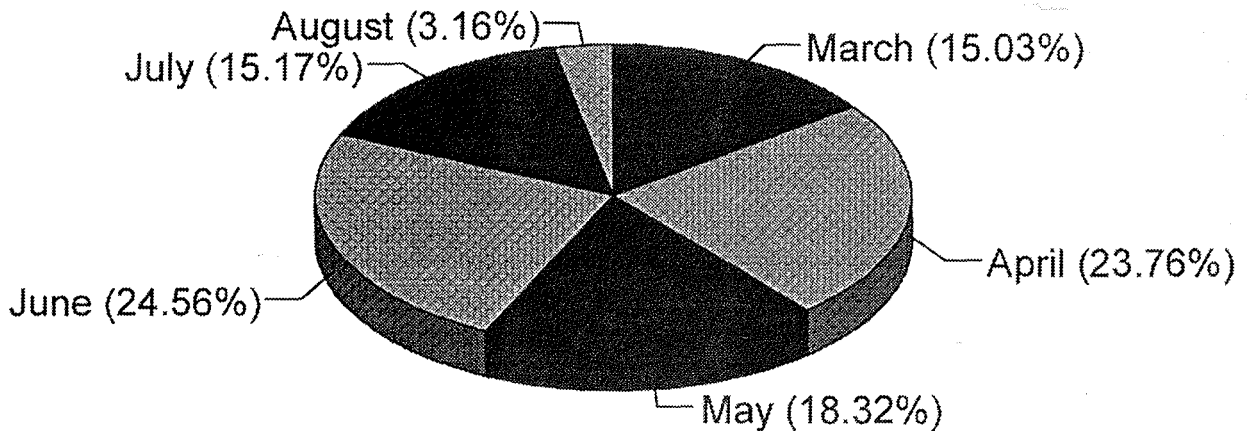
FIGURE 3.10. Distribution of monthly nitrate loadings from Minnesota's Greater Blue Earth River for March–August as a monthly percentage of the total load over the six-month period. (From Mulla, unpublished, 1998.)
