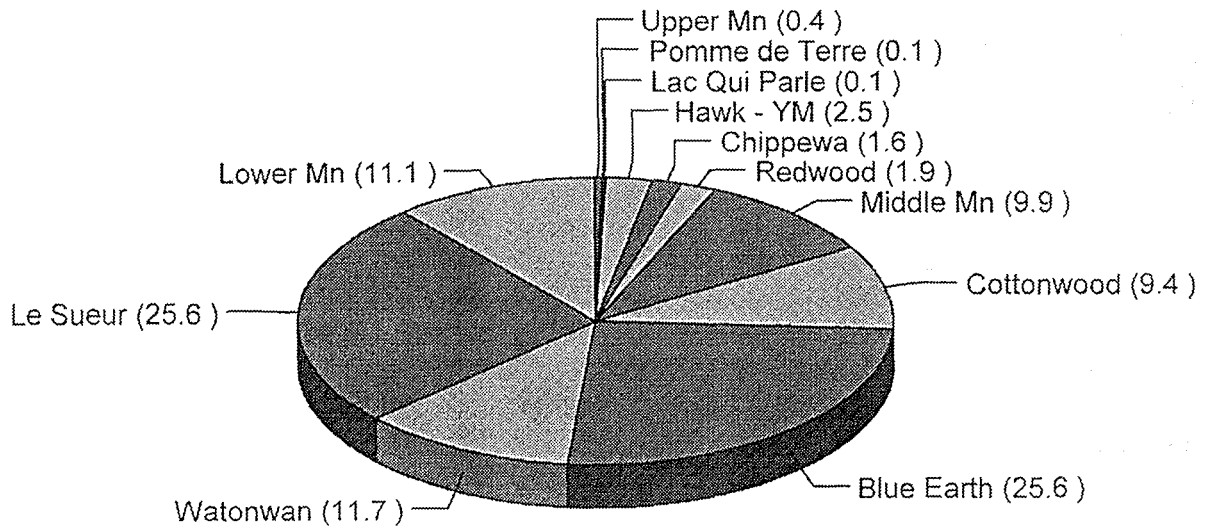
FIGURE 3.7. Percentage contributions of major watersheds in the Minnesota River Basin to the total nitrate load contributed by the river to the Mississippi. NOTE: See Figure 3.5 for the location of the major watersheds. (From Mulla and Mallawatantri 1997.)
