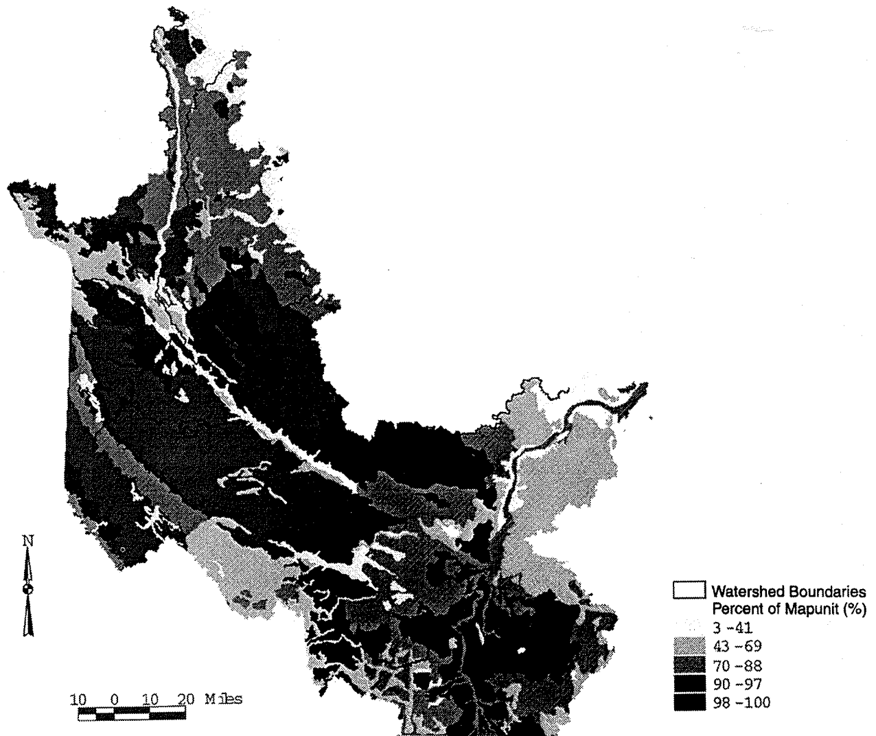
FIGURE 3.6. Distribution of surface soils in the Minnesota River Basin that contain more than 4% organic matter. NOTE: Map units represent a combination of major watersheds and agro-ecoregions. (D. Mulla and J. Bell, unpublished, University of Minnesota, St. Paul, 1998.)
