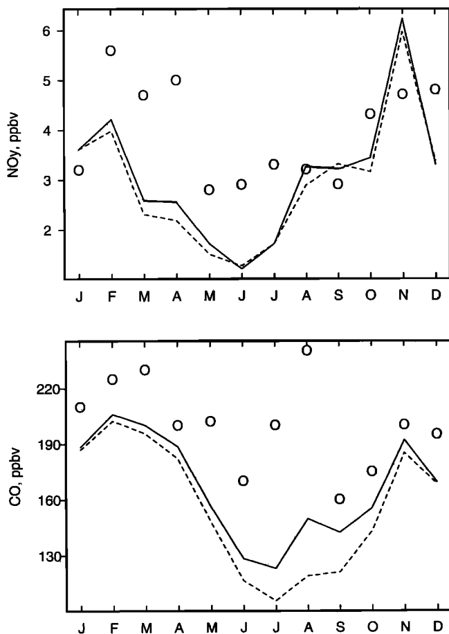
Figure 7. Seasonal variation of monthly mean concentrations of \text{NO}_y and CO at Shenandoah National Park, Virginia (mountain ridge site, 1100 m altitude). The observations were sampled at 0000–4000 LT to avoid the effect of daytime upslope flow [Poulida et al. , 1991] while model results are 24-hour averages sampled in model layer 2 (Figure 1). Observations (Table 2) are plotted as open circles, and model results are plotted as solid lines. The observations are for 1 year only, hence no interannual standard deviations are shown. The dashed lines show model results for a simulation without emission of isoprene.
