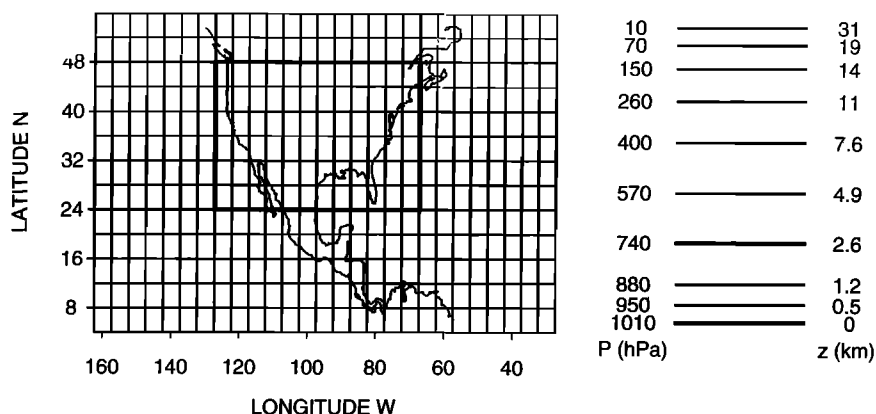
Figure 1. Model domain and grid. The edges of the figure are the boundaries of the model domain. The thick line delineates the U.S. boundary layer as defined in the paper for regional budget analyses.
