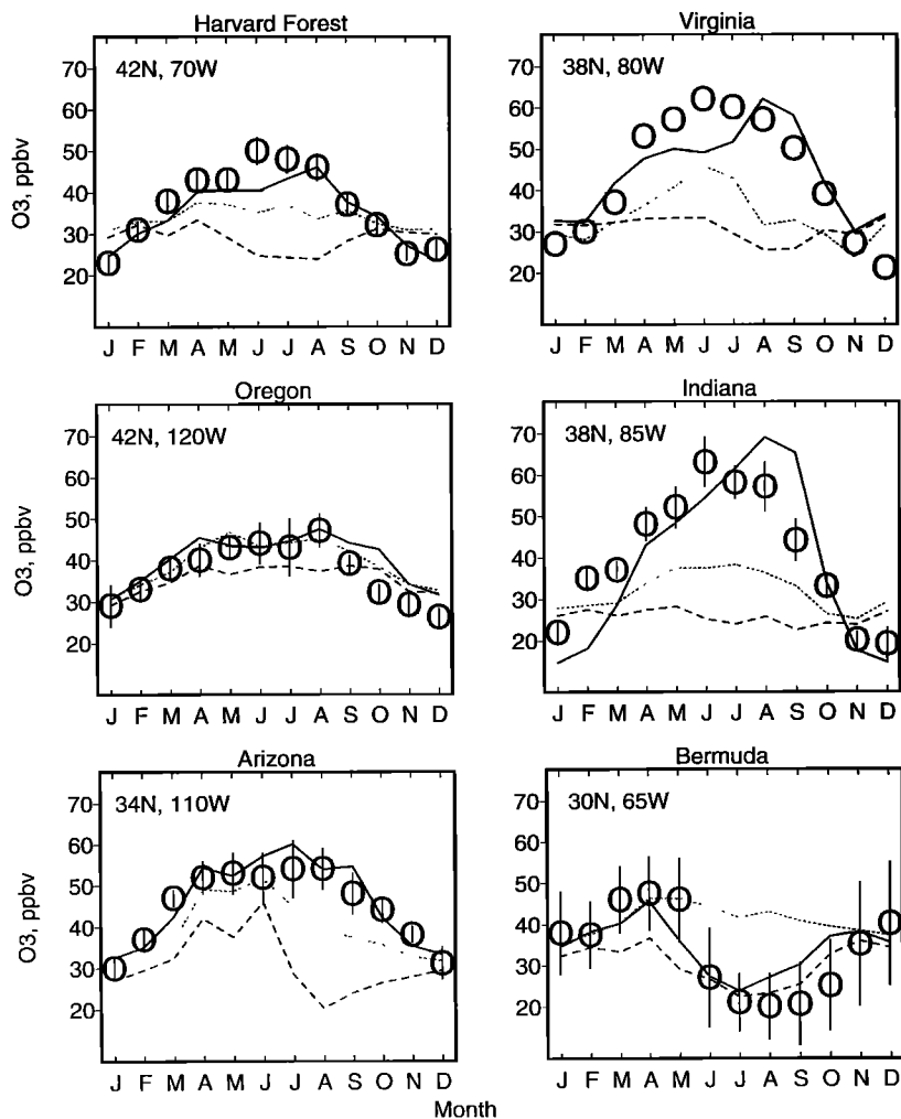
Figure 4. Seasonal variation of simulated and observed monthly mean O_3 concentrations (ppbv) in surface air at 1300-1600 local time. Observed monthly means for 1980-1995 are plotted as open circles; the vertical bars are the interannual standard deviations. Model results are shown for the standard simulation (solid lines), the no-chemistry simulation (dotted lines), and the zero- NO_x simulation (dashed lines). The observations are from the EPA/AIRS network averaged over 4^\circ \times 5^\circ grid squares (the center of the grid square is indicated), except for Harvard Forest (Munger et al., submitted manuscript, 1997) and Bermuda [Olmans and Levy, 1992]. Concentrations at Bermuda are 24-hour averages.
