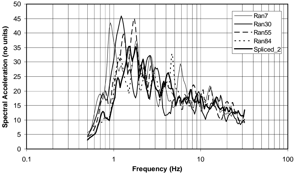
Figure C3-16. Response spectra of selected transverse records (5% of critical damping).
