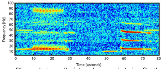
Blue whale call (above) recorded in Southern California
