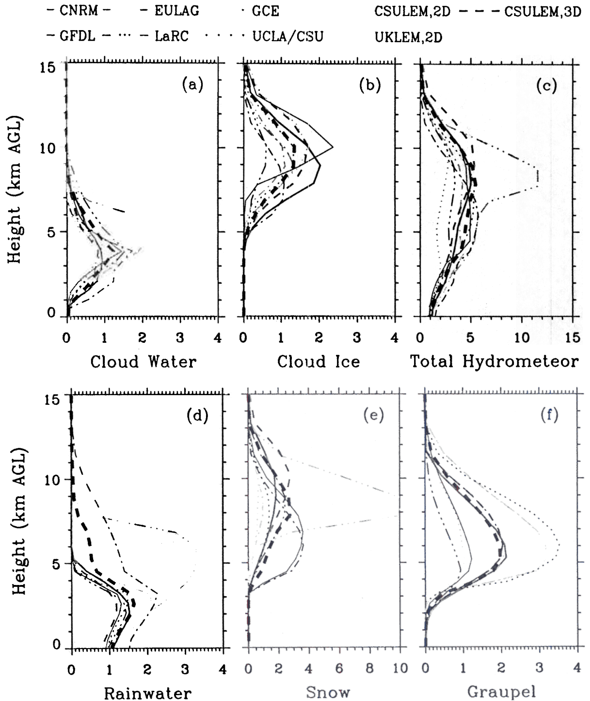
Figure 9. The all-sub-case mean profiles (AGL = above ground level) of the mixing ratios of (a) cloud-water mixing ratio, (b) cloud-ice mixing ratio, (c) total hydrometeor, (d) rainwater, (e) snow and (f) graupel/hail. The black dashed lines in (a), (b) and (c) show the consensus of all models. Units for all horizontal axes are 0.01 \text{ g kg}^{-1} . No observations are available for comparison. See Table 2 for explanation of acronyms.
