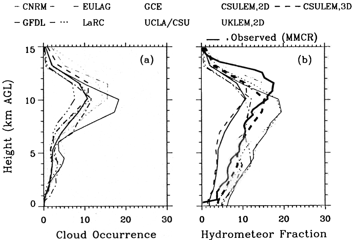
Figure Same as Fig. 9 except for cloud occurrence and hydrometeor fractions. Units for the horizontal axes are percentages.
