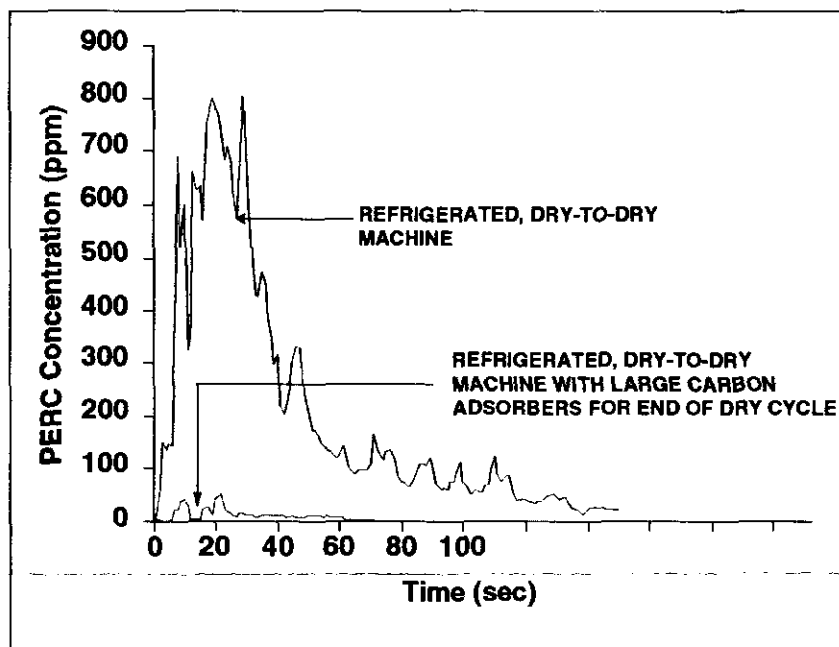
Figure 1. Operator exposure when loading or unloading a dry-to-dry, refrigerated, drycleaning machine vs. same machine with a retrofitted large, closed-loop, carbon adsorber used as a secondary vapor control system.
