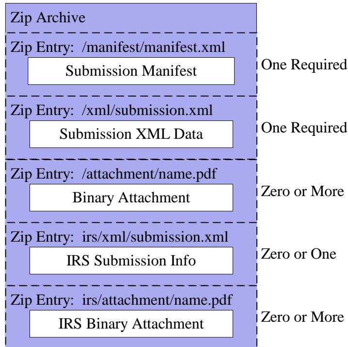
Figure 1-5. State Submission Message Structure
