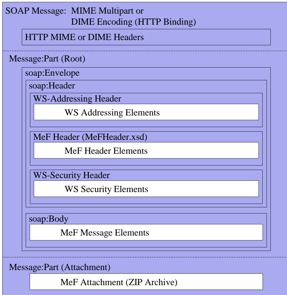
Figure 1-3. MeF Basic SOAP with Attachments Message Structure
