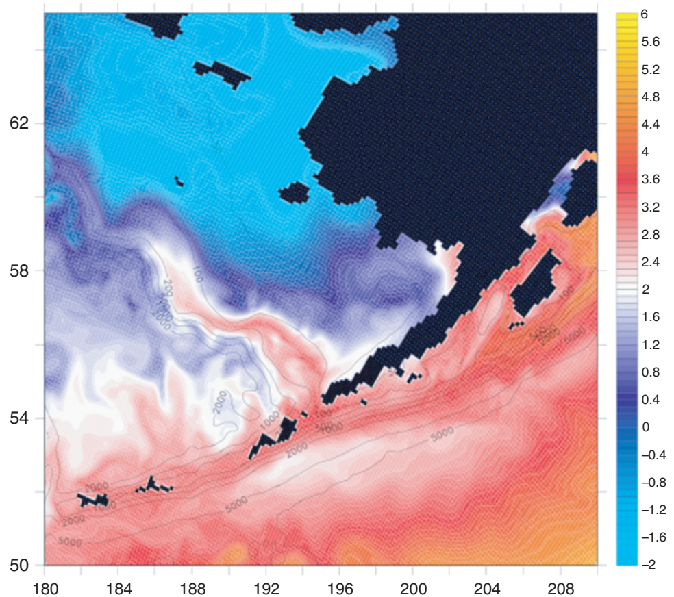
Figure 3.29: Model-generated sea surface temperature in the southeastern Bering Sea for 15 April 2000. Axes denote latitude ( ^{\circ} N) and longitude ( ^{\circ} E). Bathymetry is contoured in meters. Note the penetration of warmer waters from the Gulf of Alaska through Unimak Pass.
