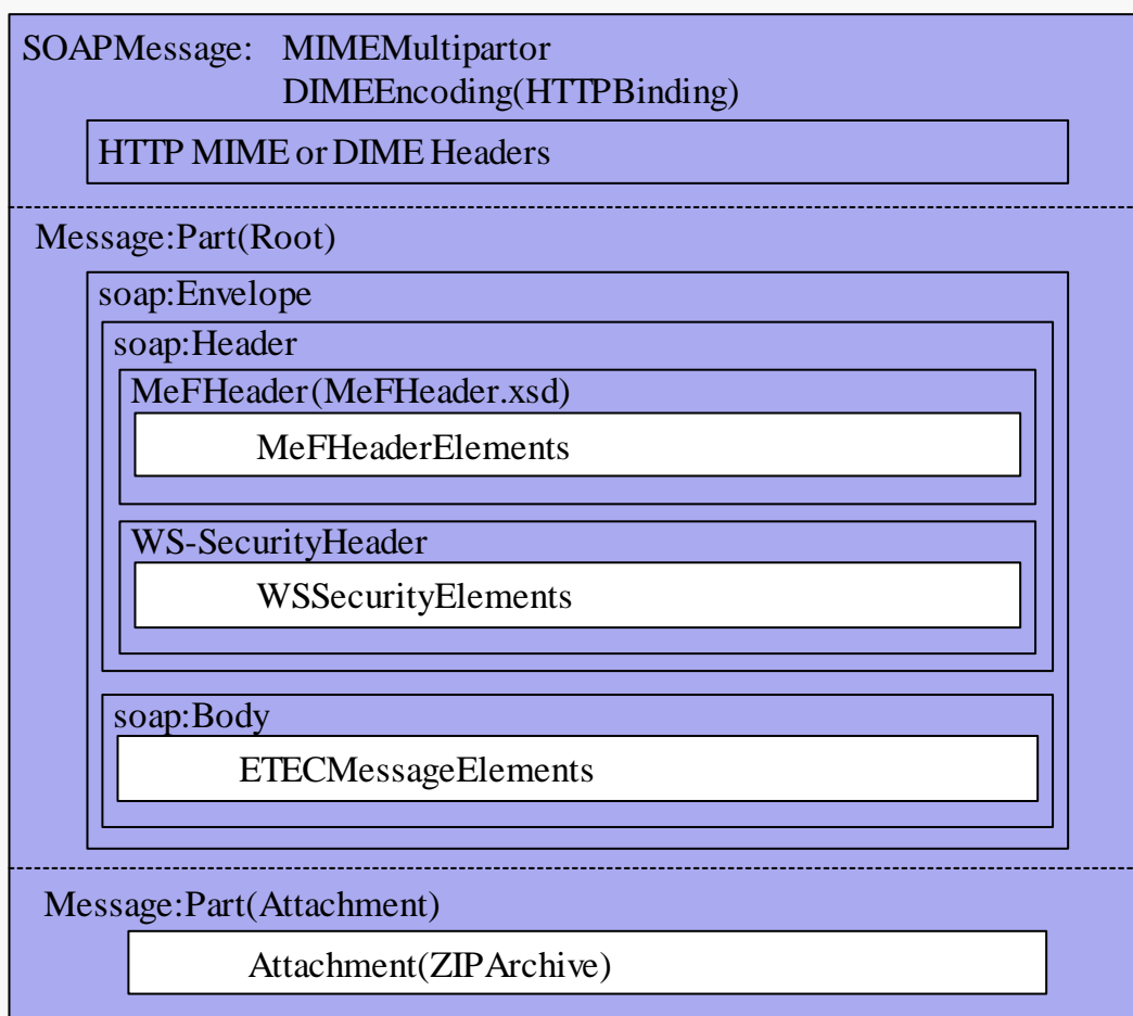
Figure 1-3. ETEC and MeF Basic SOAP with Attachments Message Structure
