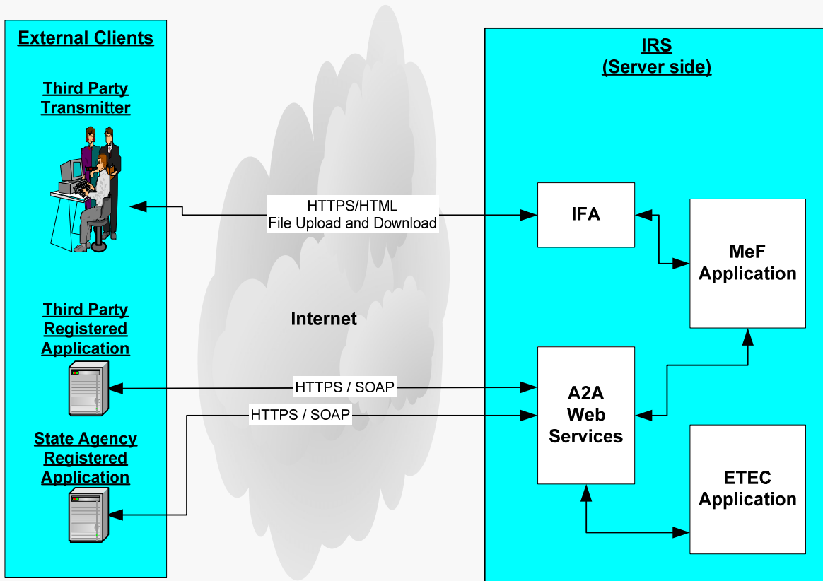
Figure 1-1. ETEC and MeF Interface Overview
